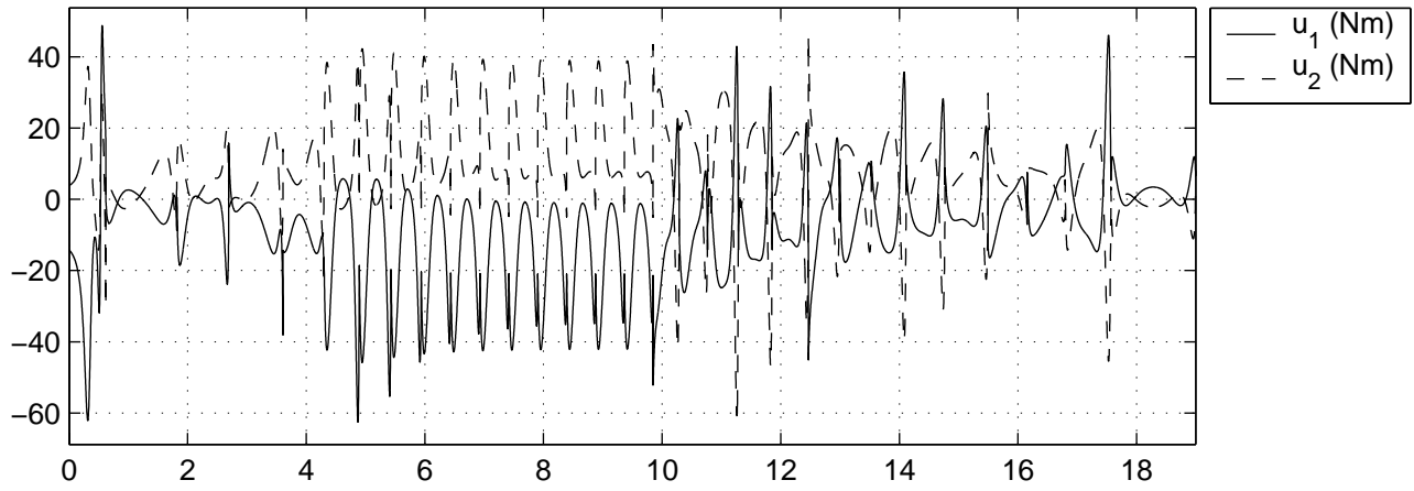
Hip controls
