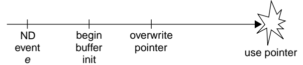
Figure 5: Sample propagation failure timeline. A non-deterministic event e causes buffer initialization to overflow and trash a pointer. A commit any time after e will prevent recovery from this failure.
