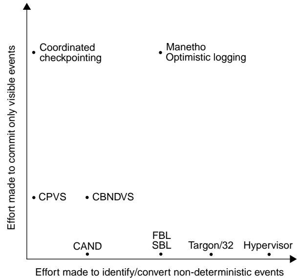
Figure 3: Protocol space. All consistent recovery protocols fall somewhere in this space. Some protocols focus on dealing with non-determinism, while others concern themselves with visible events. Some do a little of each.
