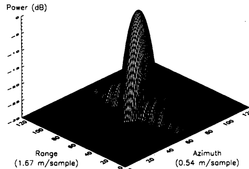
Fig. 3. Impulse response function from SIR-C data (C-Band, HH polarization).
