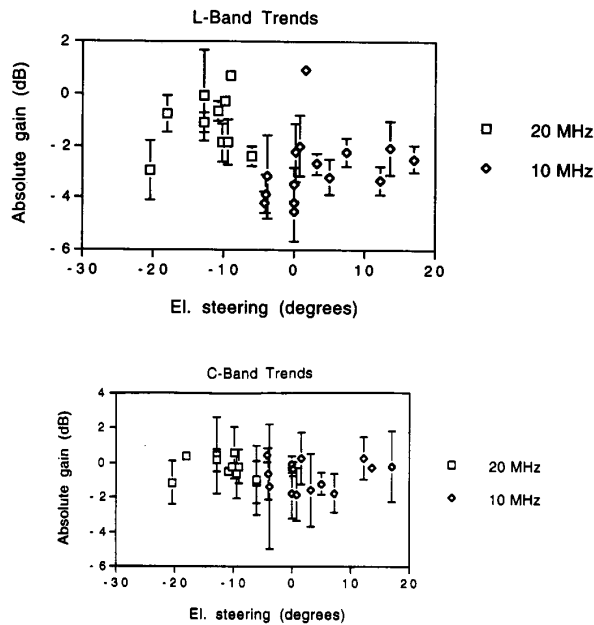
Fig. 7. Plots of residual absolute gain versus electronic steering angle.
