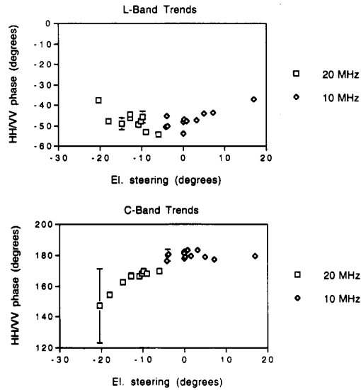
Fig. 6. Plots of average HH/VV phase differences versus electronic steering angle.
