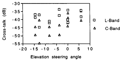
Fig. 5. Average cross-talk estimates versus elevation steering angle.
