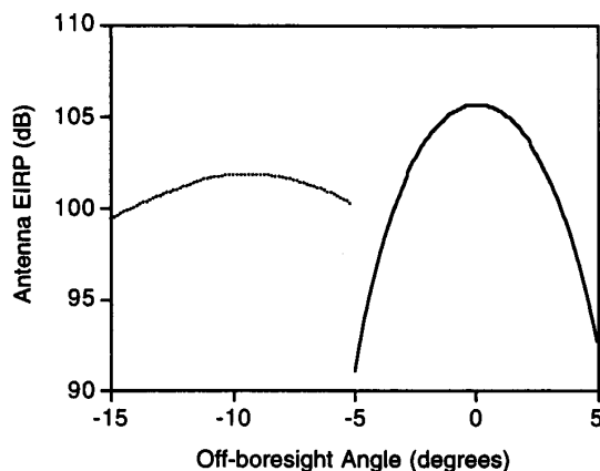
Fig. 2. Plots of Equivalent Isotropic Radiated Power (EIRP) for two SIR-C transmit antenna patterns ( L -band, H -polarization). The right-hand pattern in the figure corresponds to the L -band H -polarized pattern on transmit for zero degree beam steering and no spoiling. The left-hand pattern in the figure corresponds to the L -band H -polarized pattern on transmit for -10 degree beam steering and maximum spoiling.
