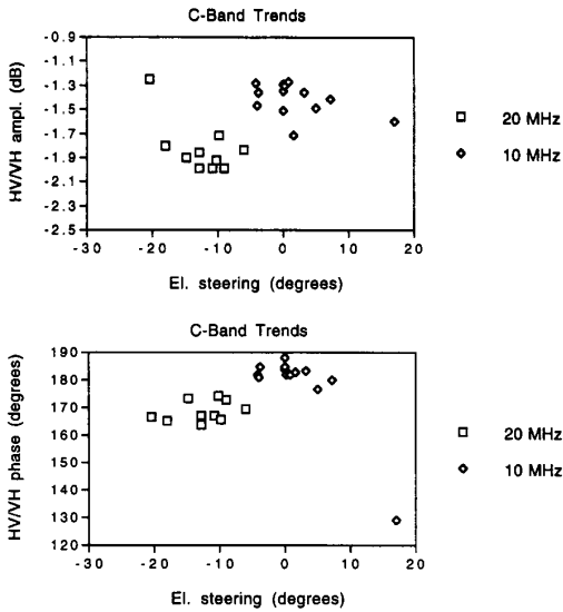
Fig. 4. HV/VH amplitude variations for different electronic steering angles.
