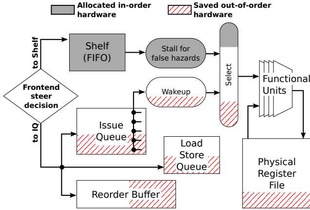
Figure 3: Design overview with FIFO shelf.
