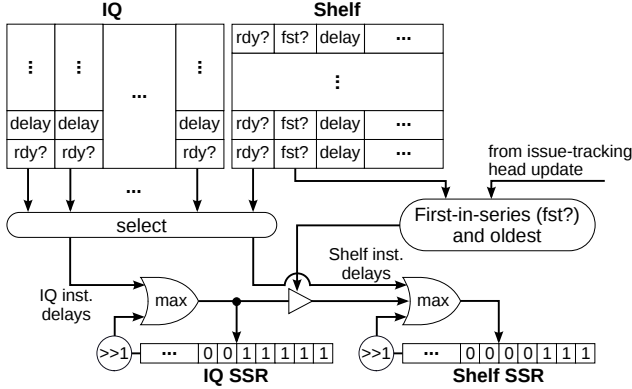
Figure 5: Delaying the shelf for speculation.
