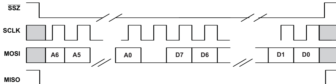
Figure 5-56. SPI Timing Diagram for Register Write
