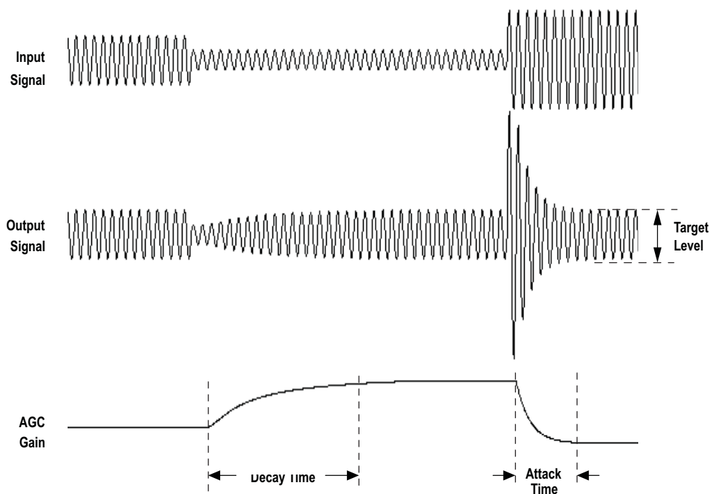
Figure 5-3. AGC Characteristics
