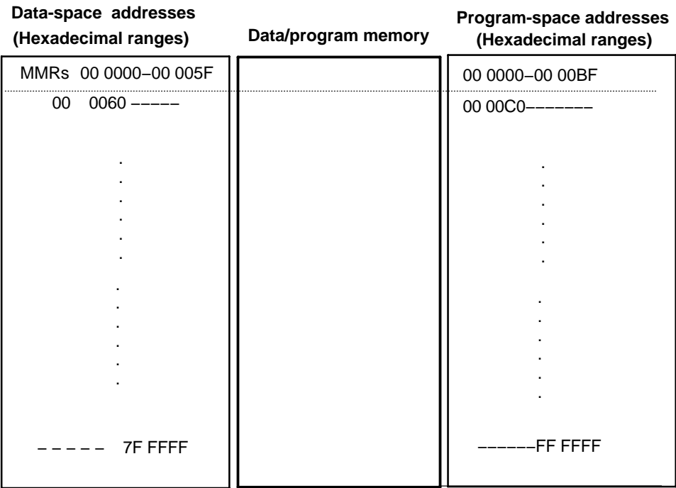
Figure 3–1. -Memory Map
