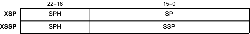
Figure 2–10. Extended Stack Pointers
