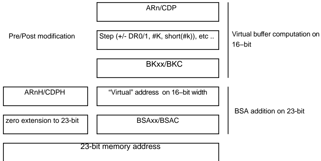
Figure 6–14. Circular Buffer Computation in 23-bit
