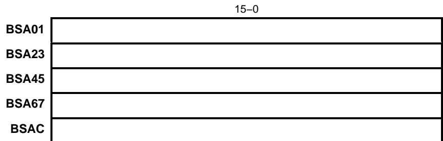
Figure 2–6. Circular Buffer Start Address Registers
