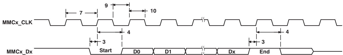
Figure 6-23. MMC/SD Card Response Timing
