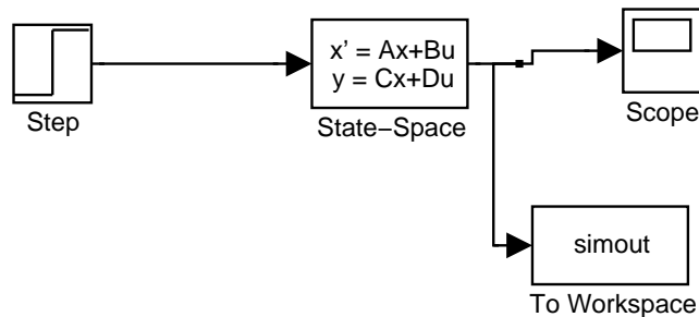
Figure 1: Simulink model to test numerical integration. Set the “Save format” option of the “To Workspace” block to “Array”.
