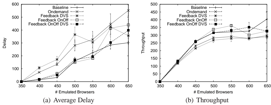
Fig. 12 Other Metrics: Average Delay, Deadline Miss Ratio, and Throughput
