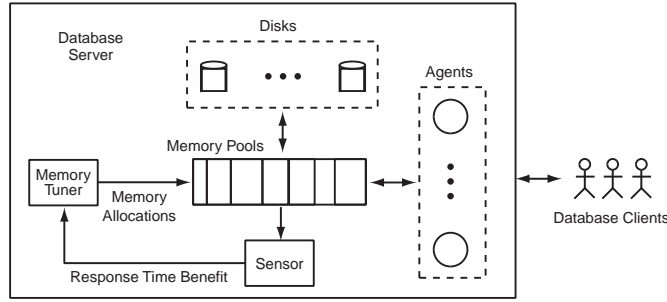
Fig. 4 Architecture of database memory management.
