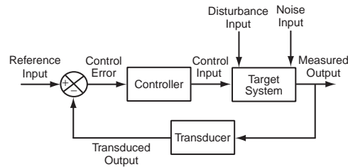
Fig. 1 Block diagram of a feedback control system.
