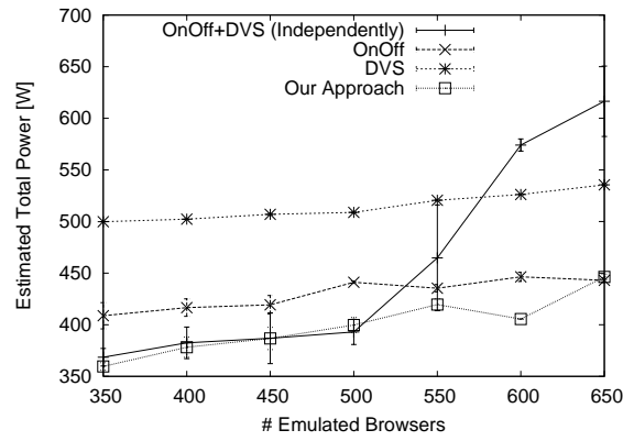
Fig. 11 Comparison of total system power consumption for different adaptive policies in the Web server case study.
