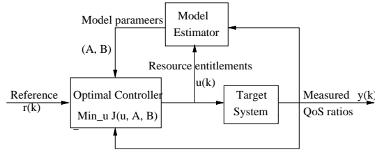
Fig. 9 A self-tuning optimal resource control system
