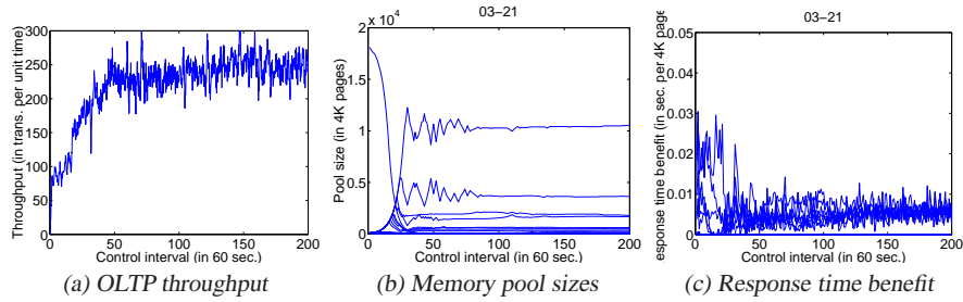
Fig. 5 Control performance under an OLTP workload.
