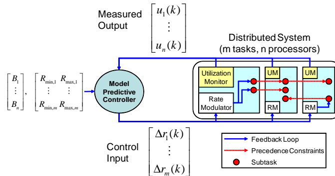
Fig. 6 The feedback control loop of EUCON.
