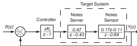
Fig. 3 Block diagram of a feedback system to control RPCs in System for the IBM Lotus Notes Domino Server.
