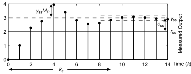
Fig. 2 Response of a stable system to a step change in the reference input. At time 0, the reference input changes from 0 to 2. The system reaches steady state when its output always lies between the light weight dashed lines. Depicted are the steady state error ( e_{ss} ), settling time ( k_s ), and maximum overshoot ( M_p ).
