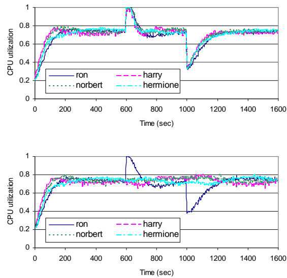
Fig. 7 The CPU utilization of all the processors in a Linux cluster when subtask execution times change on all four processors (top figure) and only one processor (bottom figure)
