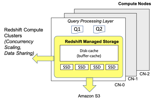
Figure 5: Redshift Managed Storage
