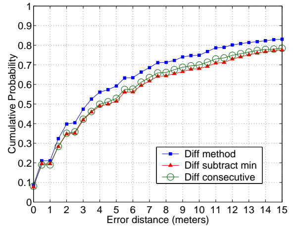
Figure 16: Cumulative error for the three Diff methods over the four hallways, where the transmission power level changes for every packet transmitted.
