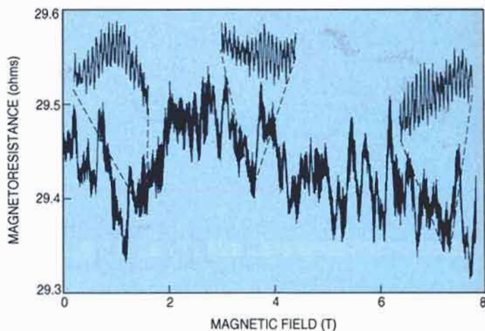
Electrical resistance of a tiny gold ring (electron micrograph, left), as a function of imposed magnetic field, measured by the authors 5 at 0.06 kelvin. The fine Aharonov–Bohm oscillations (shown expanded) correspond to a flux periodicity of h/e through the area encircled by the ring. Figure 2
