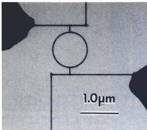
Electrical resistance of a tiny gold ring (electron micrograph, left), as a function of imposed magnetic field, measured by the authors 5 at 0.06 kelvin. The fine Aharonov–Bohm oscillations (shown expanded) correspond to a flux periodicity of h/e through the area encircled by the ring. Figure 2
