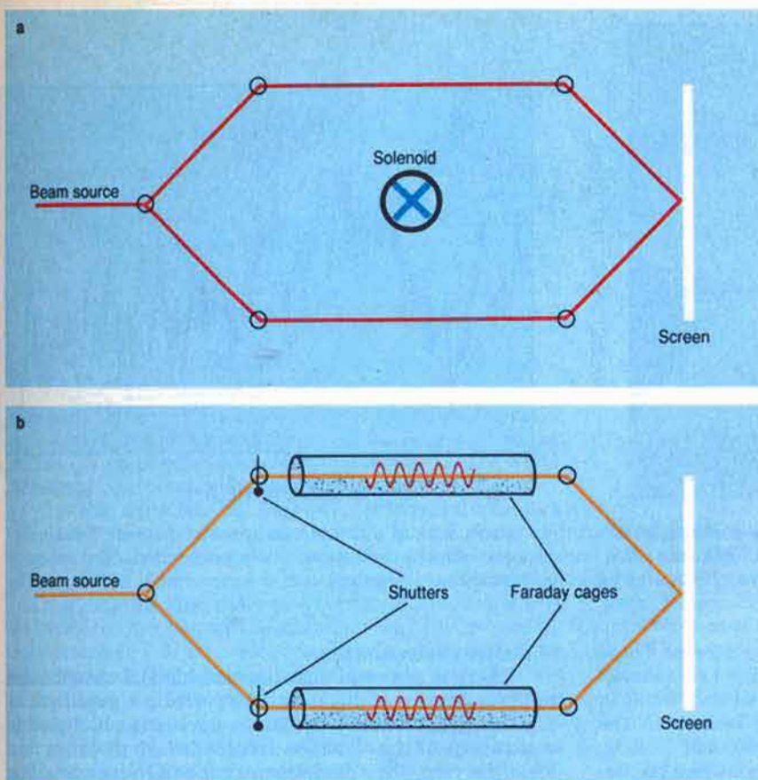
Aharonov-Bohm magnetic (a) and electrostatic (b) effects are counterintuitive consequences of quantum theory. An electron beam, split into two alternative paths, can exhibit interference effects when the beams recombine. Surprisingly, the relative phase between the two paths depends on potentials whose derivative force fields are completely shielded from the electrons. In a the phase difference is determined by the magnetic flux \Phi through a long solenoid threaded between the paths. Changing \Phi alters the interference pattern at the screen. In b the two paths are subjected to different electrostatic potentials, but only while the chopped beams are shielded within Faraday cages. Nonetheless, the potentials effect the interference. Figure 1
