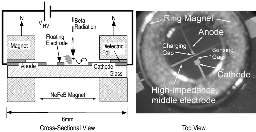
Left – Cross-section of the micro-Geiger counter on a 6\text{mm}^2 \times 6\text{mm}^2 glass chip in a ring magnet configuration, Right – Photograph of top view showing high-impedance middle electrode. Magnets were positioned to enhance the wireless signal emitted during operation.
