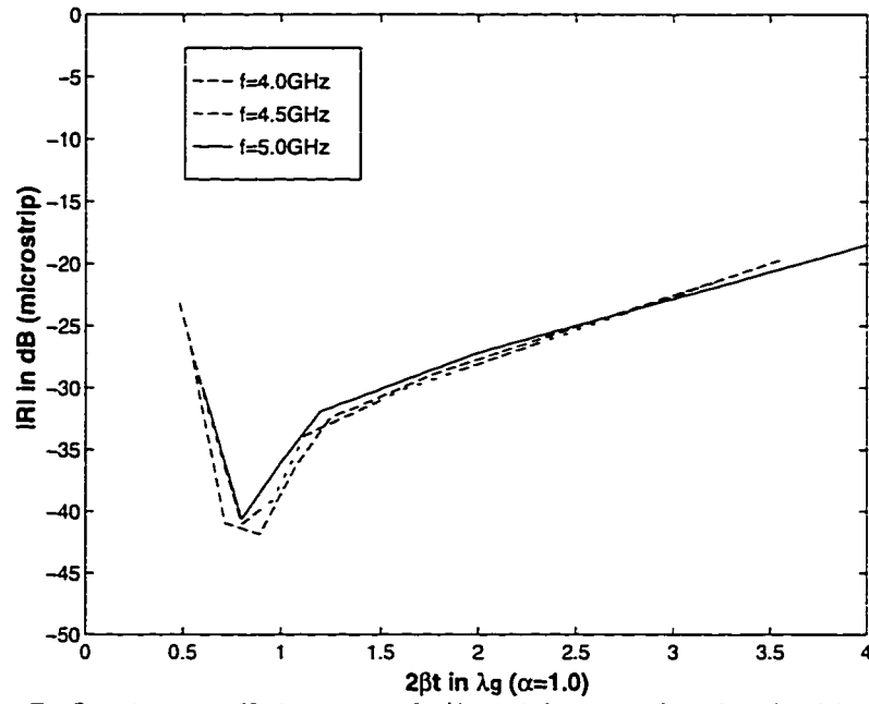
Figure 7.9: Reflection coefficient vs 2\beta t/\lambda_g with \alpha=1.0 , for the shielded microstrip line terminated by the perfectly matched uniaxial layer.
