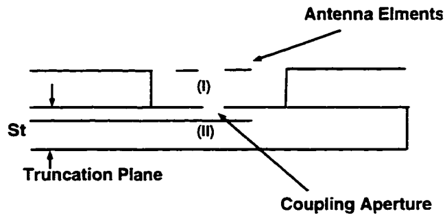
Figure 6.1: Cross-section of an aperture coupled patch antenna, showing the cavity region I and the microstrip line region II for two different FEM computation domains.
