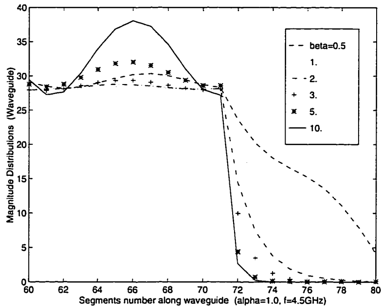
Figure 7.6: Field values of the TE_{10} mode inside a waveguide terminated by a perfectly matched uniaxial layer. The absorber is 10 elements thick and each element was 0.5 cm which translates to about 13 samples per wavelength at 4.5 GHz.
