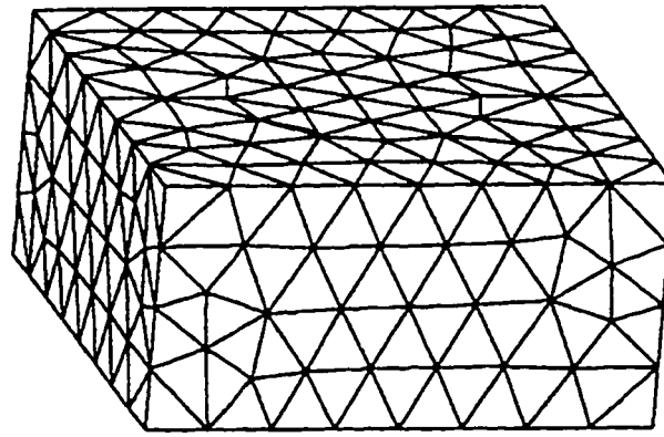
Figure 3.4: A typical geometry/mesh for a cavity-backed circular patch antenna.
