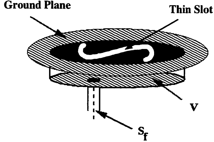
Figure 5.1: Geometry of cavity-backed microstrip antennas
