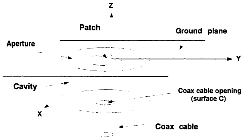
Figure 6.3: Illustration of a cavity-backed patch antenna with a coax cable feed.
