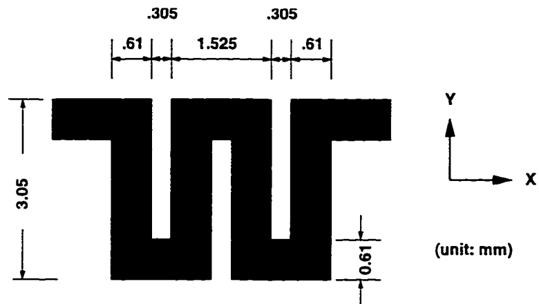
Figure 7.12: Illustration of a meander line geometry used for comparison with measurement.
