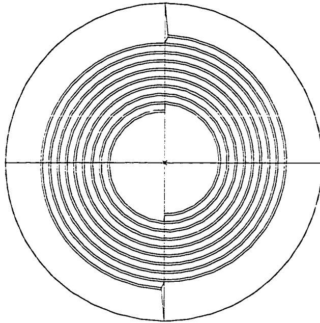
Figure 5.9: Illustration of a typical 2-arm slot-spiral design frequency=1.1GHz
