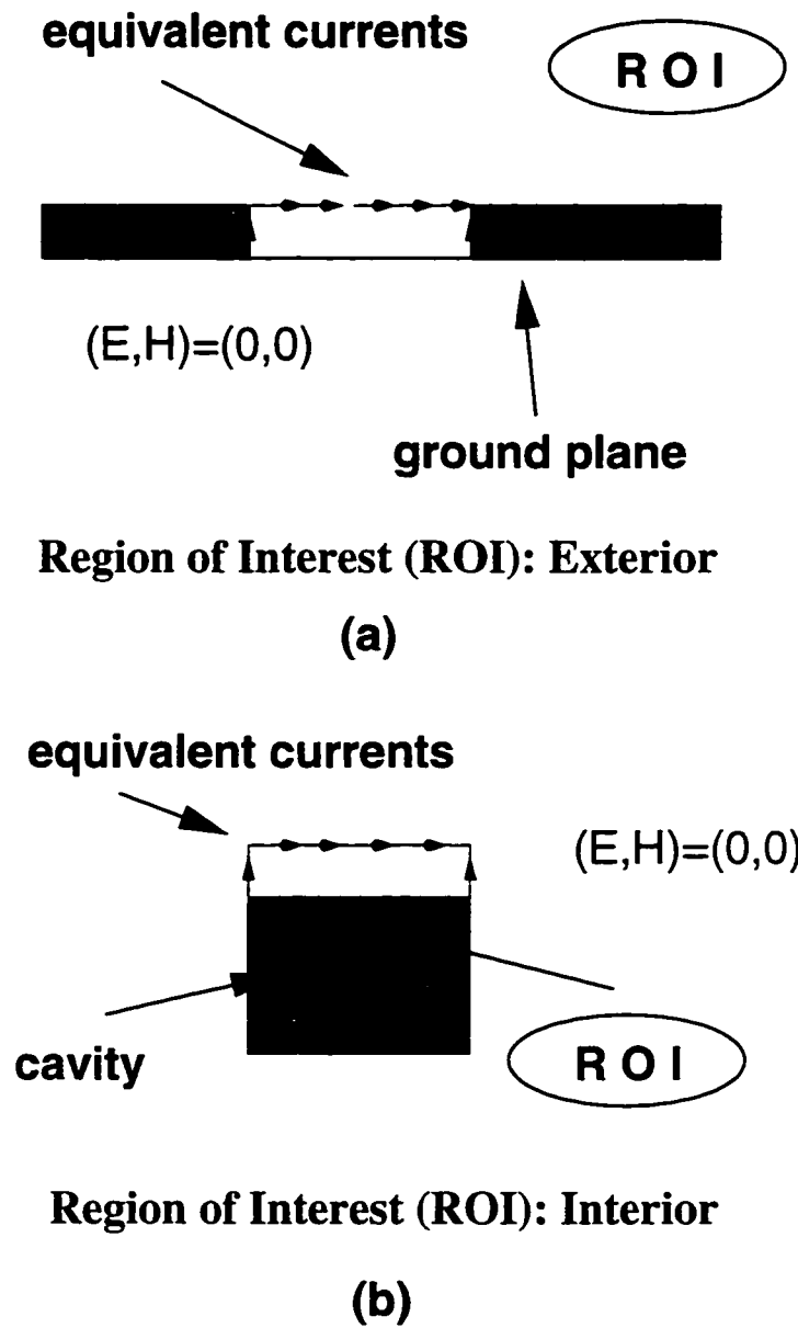
Figure 1.3: Illustrations of equivalence principle when applied to the structure shown in fig. 1.1b.
