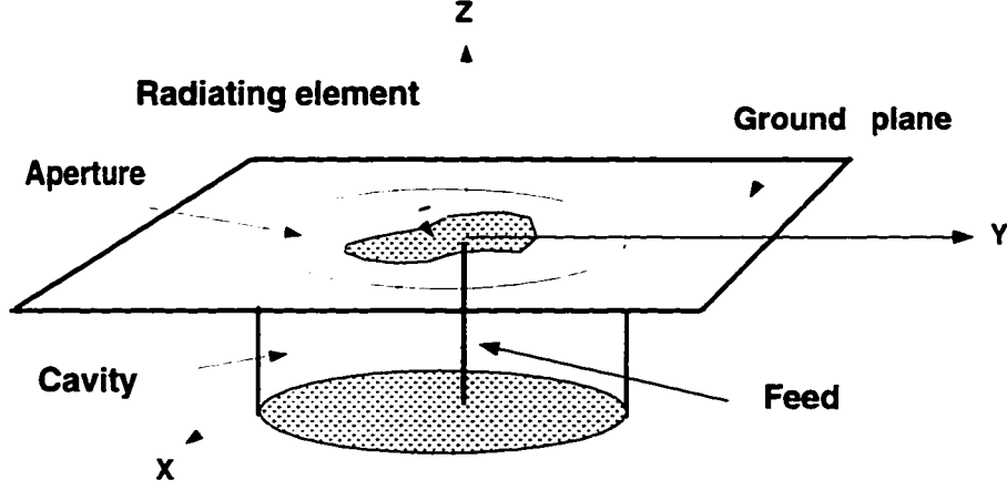
Figure 2.1: Illustration of a typical conformal antenna configuration.
