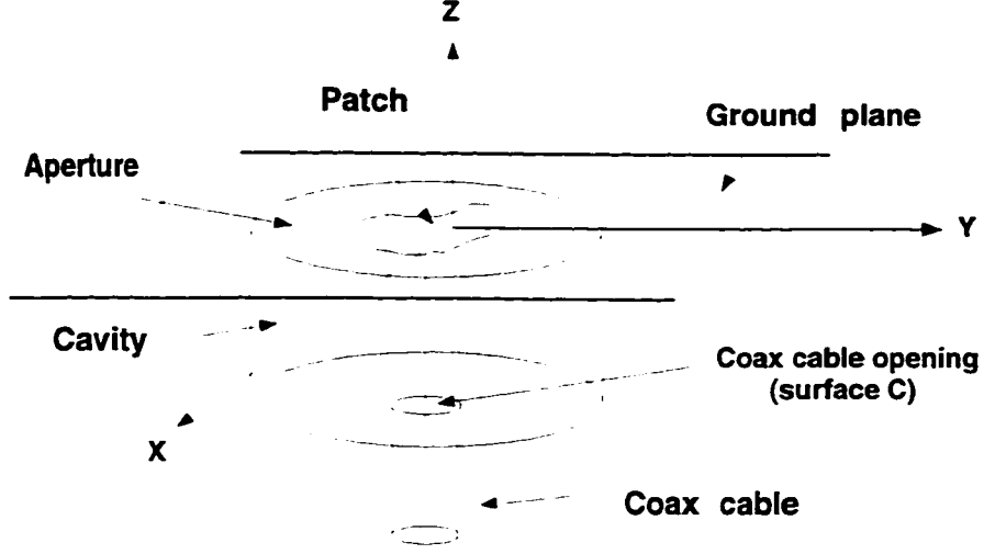
Figure 3.1: Illustration of a typical radiation and scattering problem.
