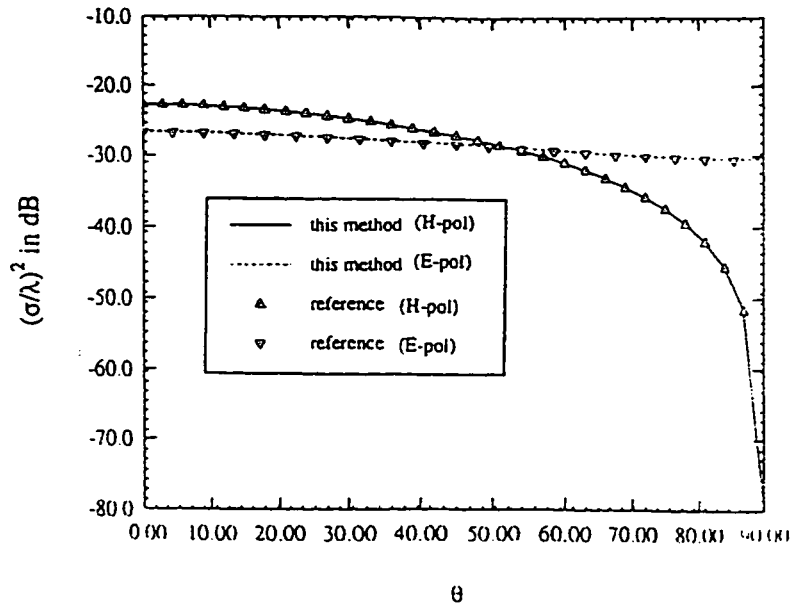
Figure 4.8: Comparisons of the monostatic radar cross section scattering by an empty aperture with the same cavity size and dielectric filling ( \epsilon_r=1 ) as the structure shown in fig. 4.6. Again, the results were calculated using the regular BiCG FE-BI technique described in chapter 3 and using the BiCG-FFT proposed in this chapter.
