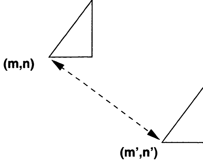
Figure 4.2: Illustration of two triangles with the corresponding indices to help to prove the convolutional property of the boundary integral.
