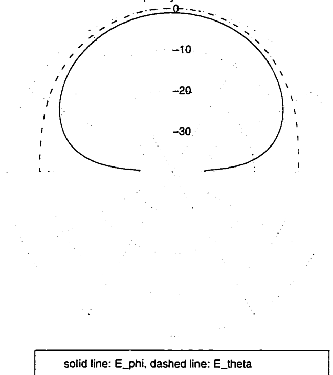
Figure 5.9: Illustration of a typical 2-arm slot-spiral design frequency=1.1GHz
