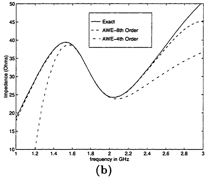
Figure 8.3: 4th order and 8th order AWE implementations using one point expansion at 1.78 GHz are shown to compare with the reference data. With the 4th order AWE solutions, 56% and 33% bandwidth agreement can be achieved for the real (a) and imaginary (b) parts of impedance computations, respectively. It is also shown that the 8th order solutions agree excellently with the reference data over the entire band. (a) Real Part (b) Imaginary Part computations
