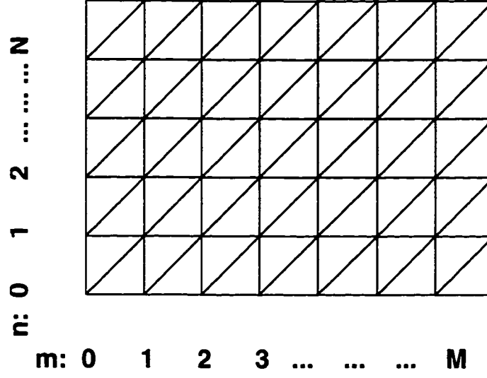
Figure 4.1: Structured mesh consists of equal right triangles
