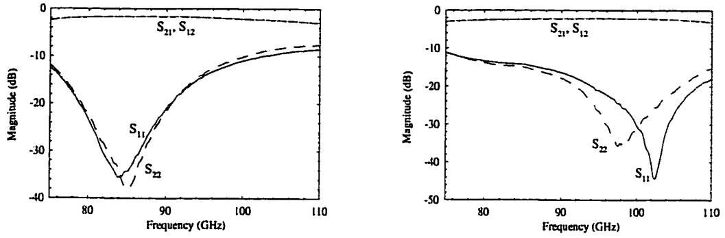
Figure 3.19: Measured S-parameters of back-to-back vertical interconnects: a) 734 \mu\text{m} midsection, 230 \mu\text{m} stub, and 100 \mu\text{m} air bridge. b) 934 \mu\text{m} midsection, 240 \mu\text{m} stub, and 130 \mu\text{m} air bridge.
