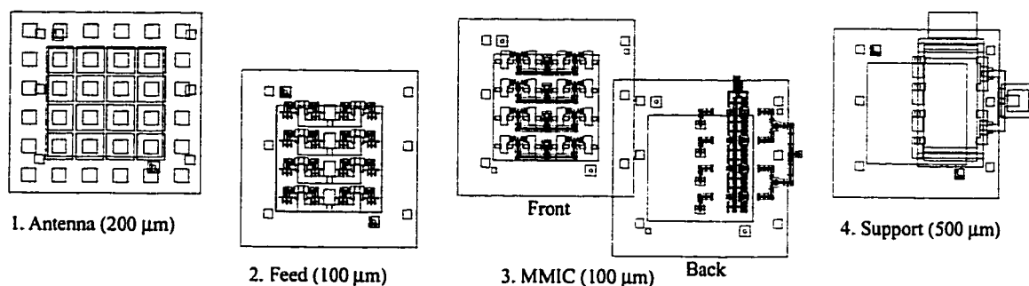
Figure 6.3: Illustration of power cube layers.
