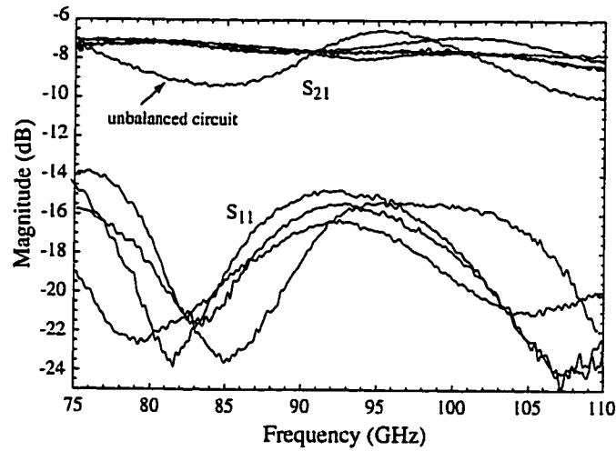
Figure B.3: Measured mismatch of 1:4 distribution network.
