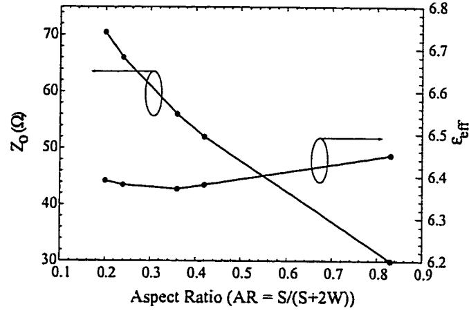
Figure 1.13: Z_0 and \epsilon_{eff} for various FGC aspect ratios where S is the center conductor width and W is the aperture width.
