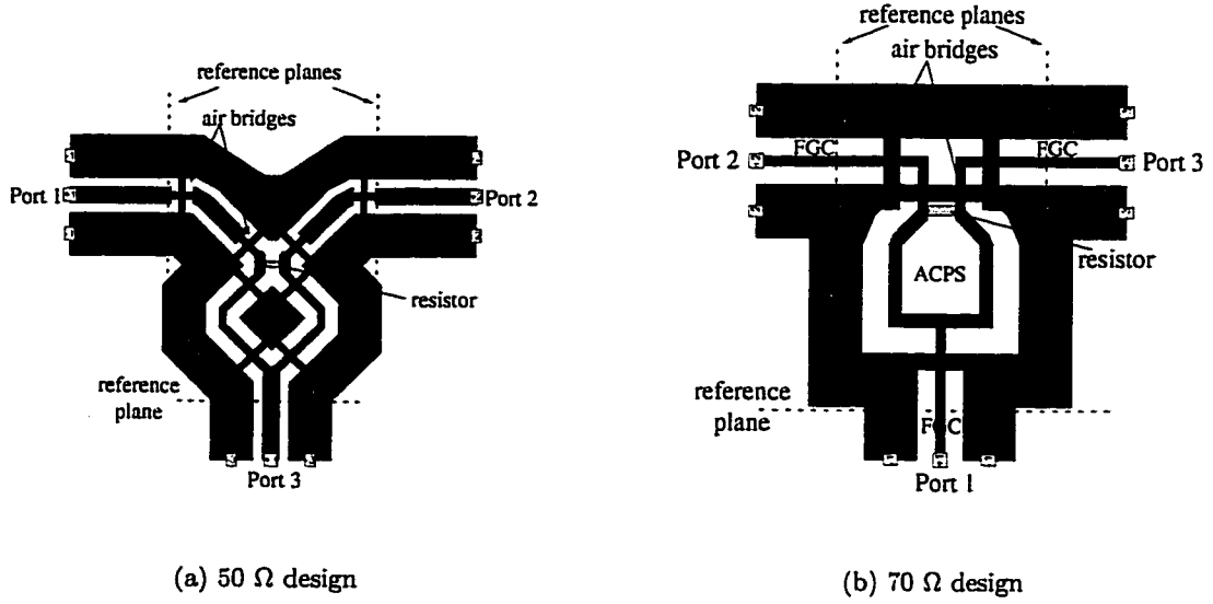
Figure 5.2: Schematics of Wilkinson power dividers as simulated in IE3D [132]: a) 50 \Omega b) 70 \Omega .
