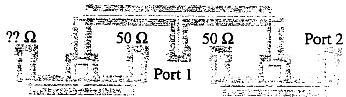
Figure B.1: Schematic of simulated network with one of three output port terminations varied from 50 \Omega .
