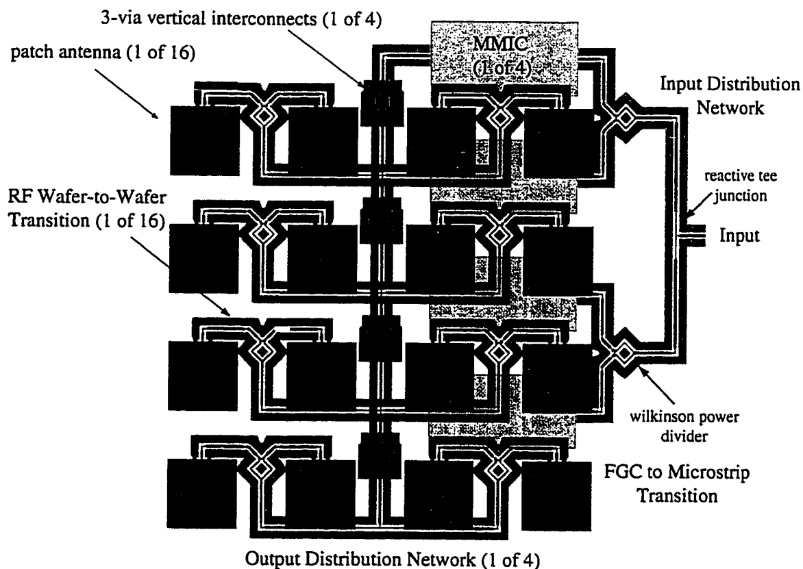
Figure 6.4: Top view illustration of power cube layers.
