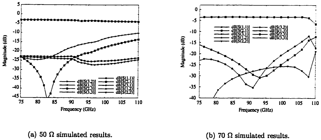
Figure 5.3: S-parameters of Wilkinson power dividers as simulated in IE3D [132]: a) 50 \Omega b) 70 \Omega .
