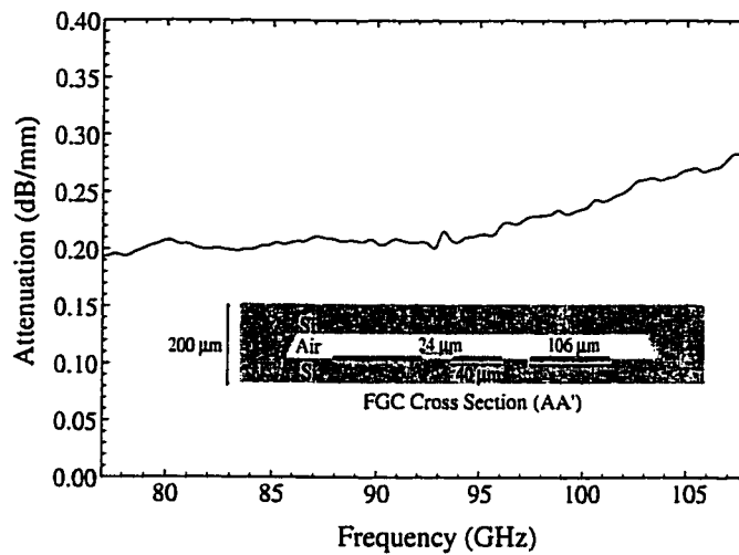
Figure 4.14: Measured Attenuation for FGC line.
