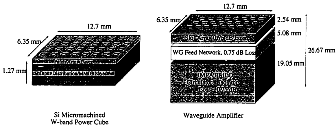
Figure 6.1: W-band micromachined power cube versus waveguide amplifier (courtesy Dr. Robert T. Kihm).
