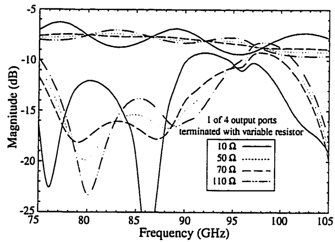
Figure B.2: Simulated effect of mismatch on 1:4 network.
