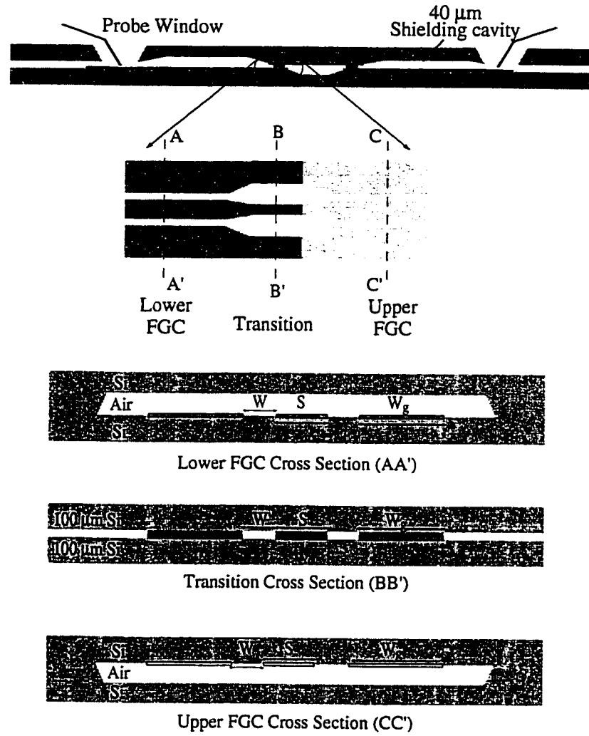
Figure 4.2: Illustration of wafer to wafer transition.
