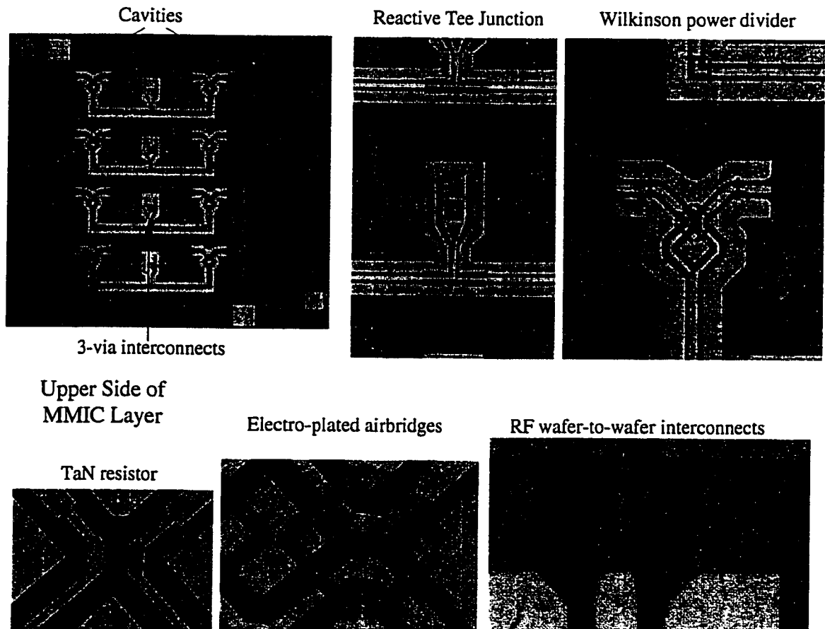
Figure 6.18: Photos of upper side MMIC layer.
