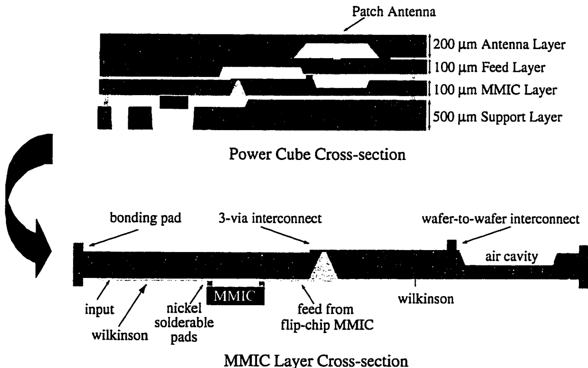
Figure 6.5: Cross section of power cube layers with close-up of MMIC layer cross section.
