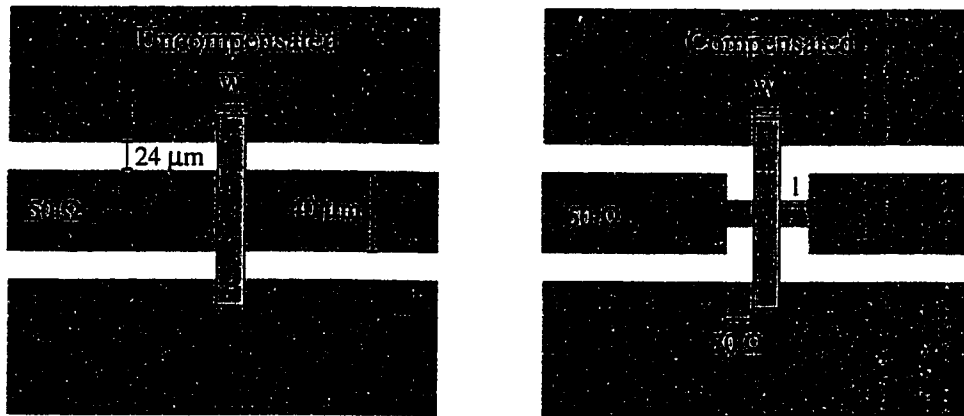
Figure A.4: Schematic of air bridge with and without compensation.
