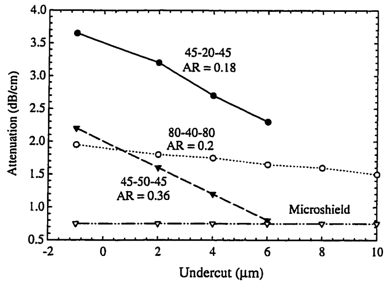
Figure 2.13: Measured loss versus undercut at 94 GHz.
