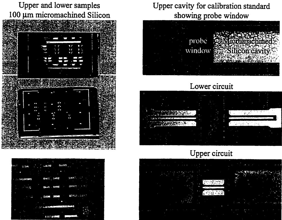
Figure 4.8: Photos of fabricated circuits.
