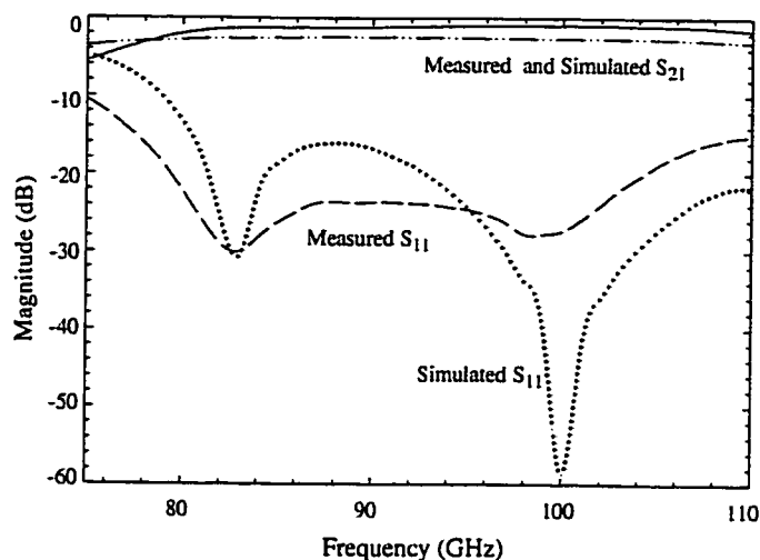
Figure 3.18: Measured S-parameters of back-to-back vertical interconnect transition compared with Libra model.
