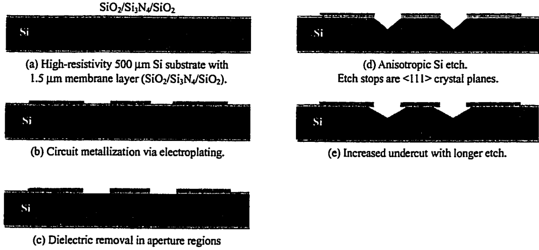
Figure 2.7: MFGC process flow.
