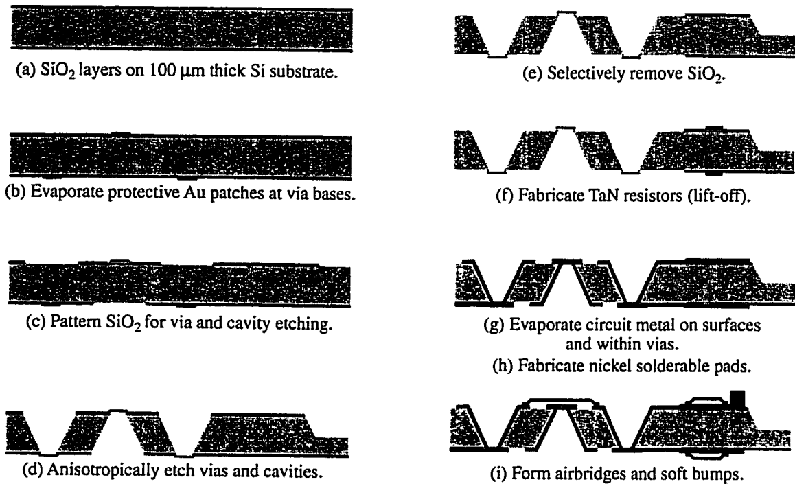
Figure 6.15: Revised fabrication flow.
