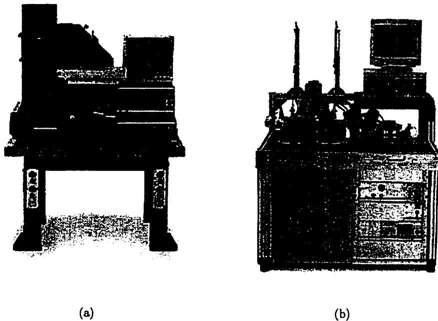
Figure 4.10: Electronics Visions Align and Bond Equipment [116].
