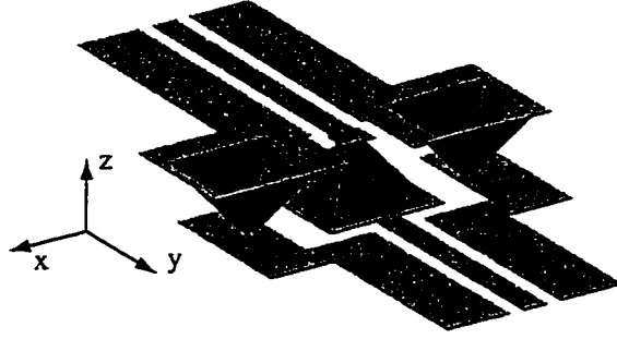
Figure 3.1: A vertical interconnect employing three micromachined pyramidal via holes. The vias permeate the Si substrate (not shown) to connect the upper and lower finite ground coplanar (FGC) transmission lines.
