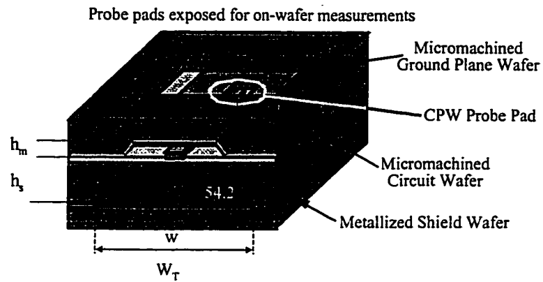
Figure 1.10: Membrane microstrip [92].
