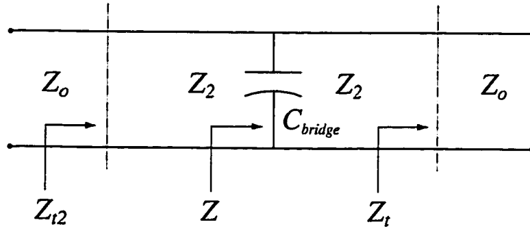
Figure A.2: Equivalent circuit model for air bridge with high impedance compensation.
