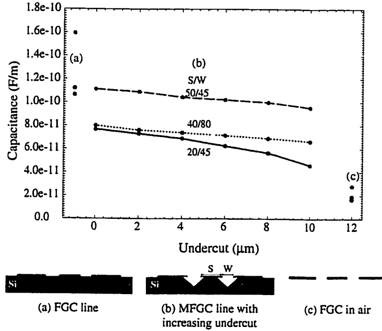
Figure 2.19: Capacitance versus undercut for three FGC lines with values for (a) a conventional FGC line (b) a micromachined FGC line with increasing lateral undercut (c) a FGC in air.
