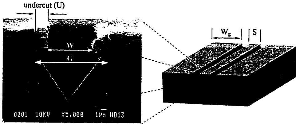
Figure 2.4: Isotropically etched Si.
