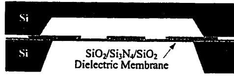
Figure 1.16: Microshield line.
