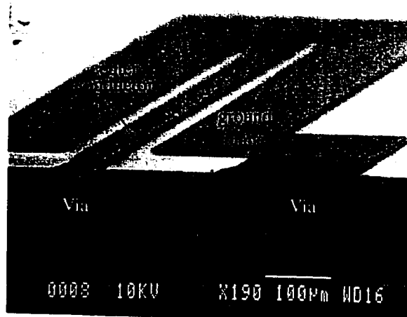
(a) Cross-section along width of three-via interconnect.
