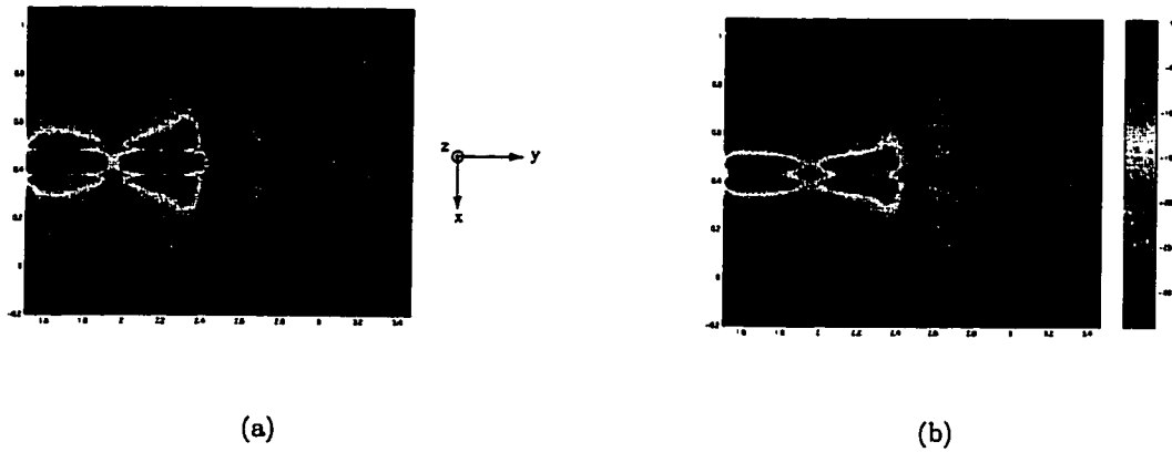
Figure 3.5: (a) Z-component of the electric field vector for the transition of Figure 3.2(a). (b) Total electric field distribution for the transition of Figure 3.2(a) showing launched horizontal electric field component.
