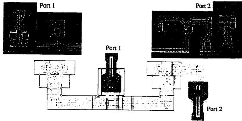
(a) Photo and schematic of passive component combination measurement of Figure 6.31(b).
