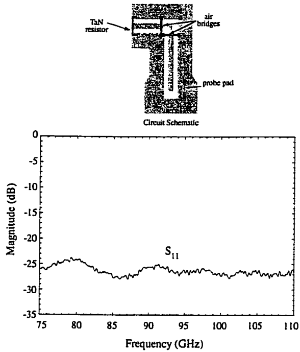
Figure 6.27: Measured right angle bend with 50\ \Omega termination.
