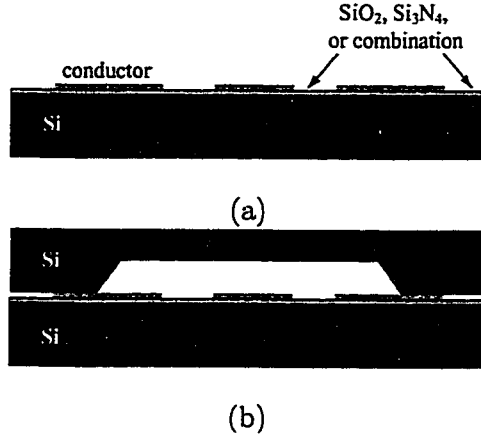
Figure 2.1: Finite Ground Coplanar Waveguide: (a) FGC on high-resistivity Si. (b) Packaged FGC.
