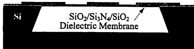
Figure D.2: Microshield low-pass filter cross-section.
