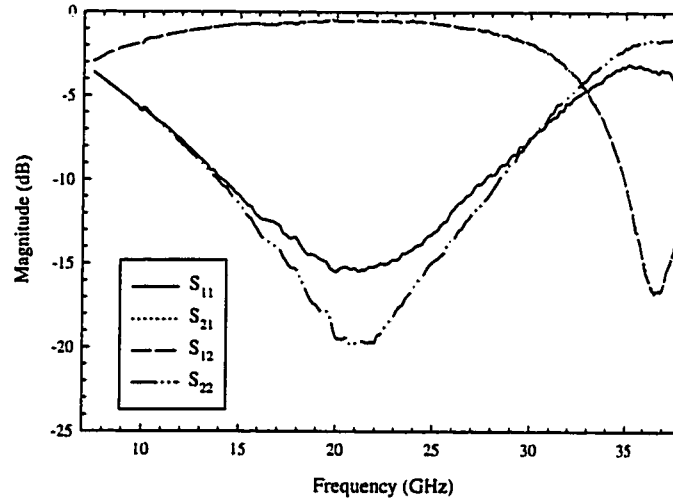
Figure D.8: Measured S-parameters for short stub.
