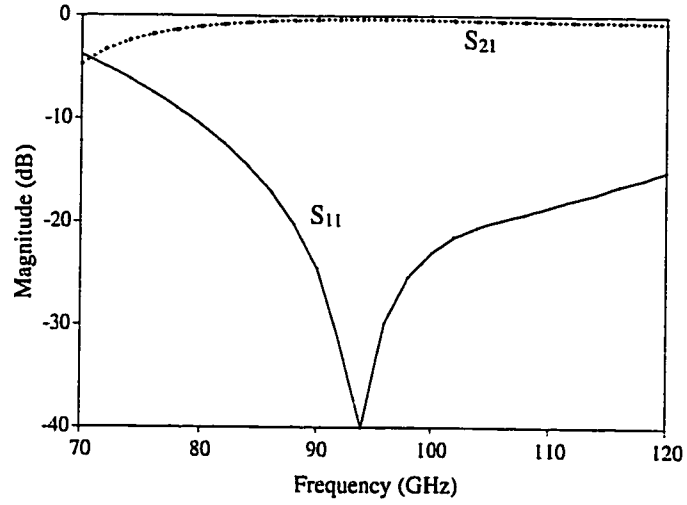
Figure 3.7: Simulated S-parameters for 3-via vertical interconnect.
