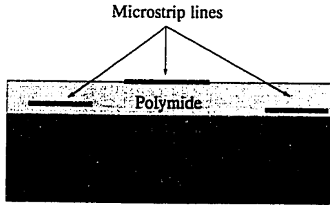
Figure 1.8: Schematic of high-density integration(HDI) as applied to microstrip.
