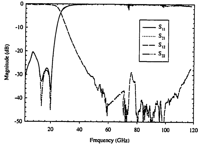
Figure D.4: S-parameters for low-pass filter measurement.
