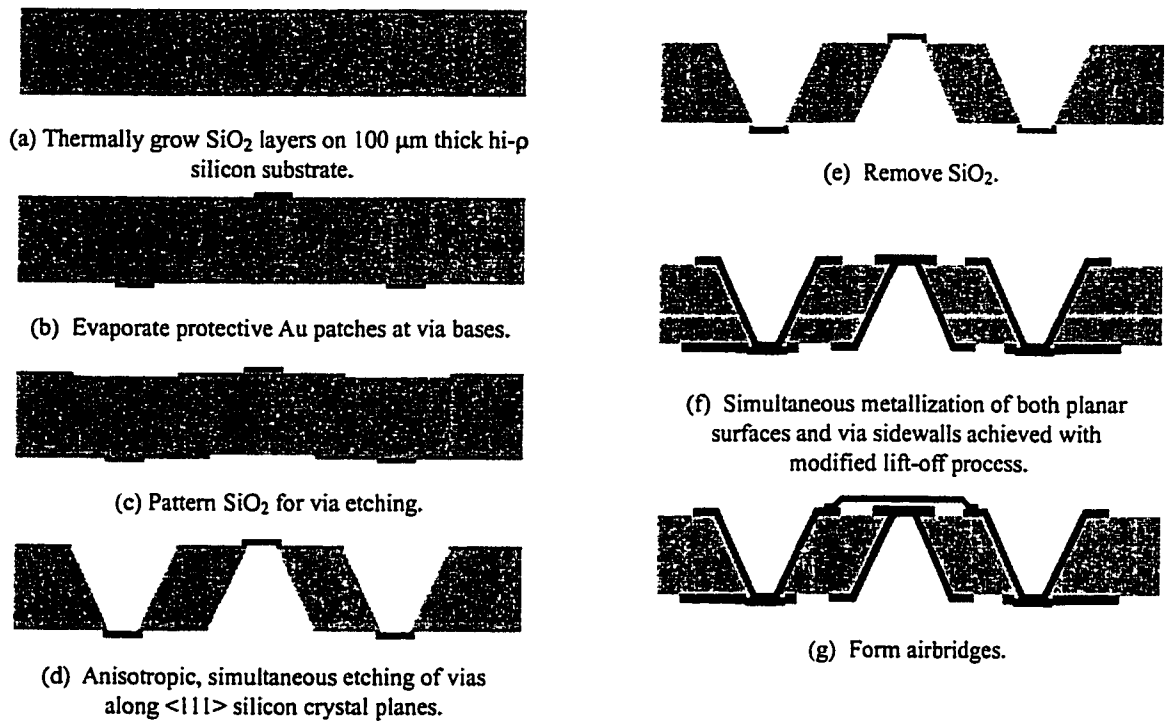
Figure 3.13: Final fabrication process for vertical interconnects.
