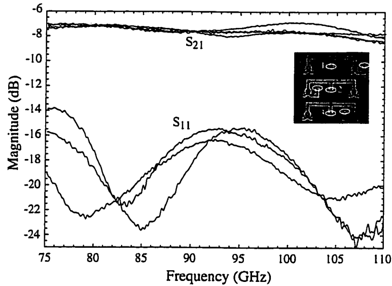
Figure 6.30: Measurements of distribution network.
