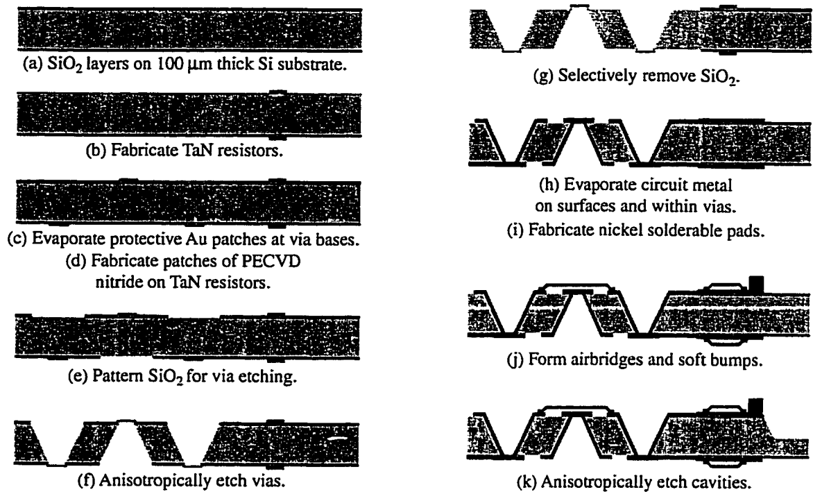
Figure 6.14: Fabrication flow.
