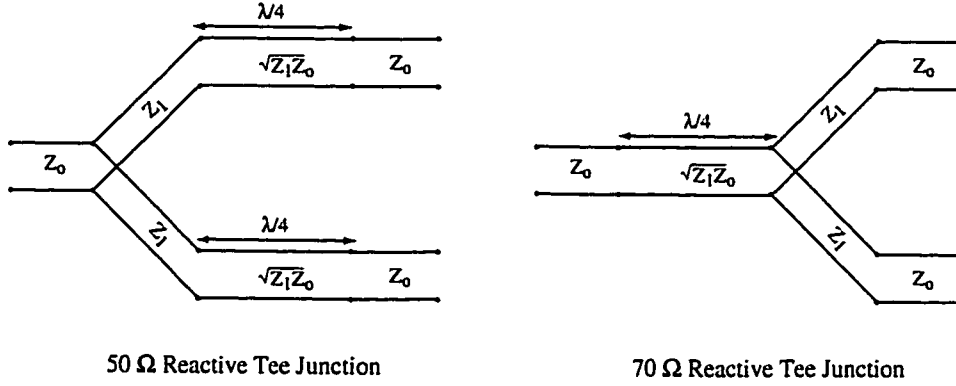
Figure 5.4: Equivalent transmission line circuit for reactive tee junction.
