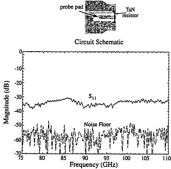
Figure 6.26: Measured 50 \Omega resistor.
