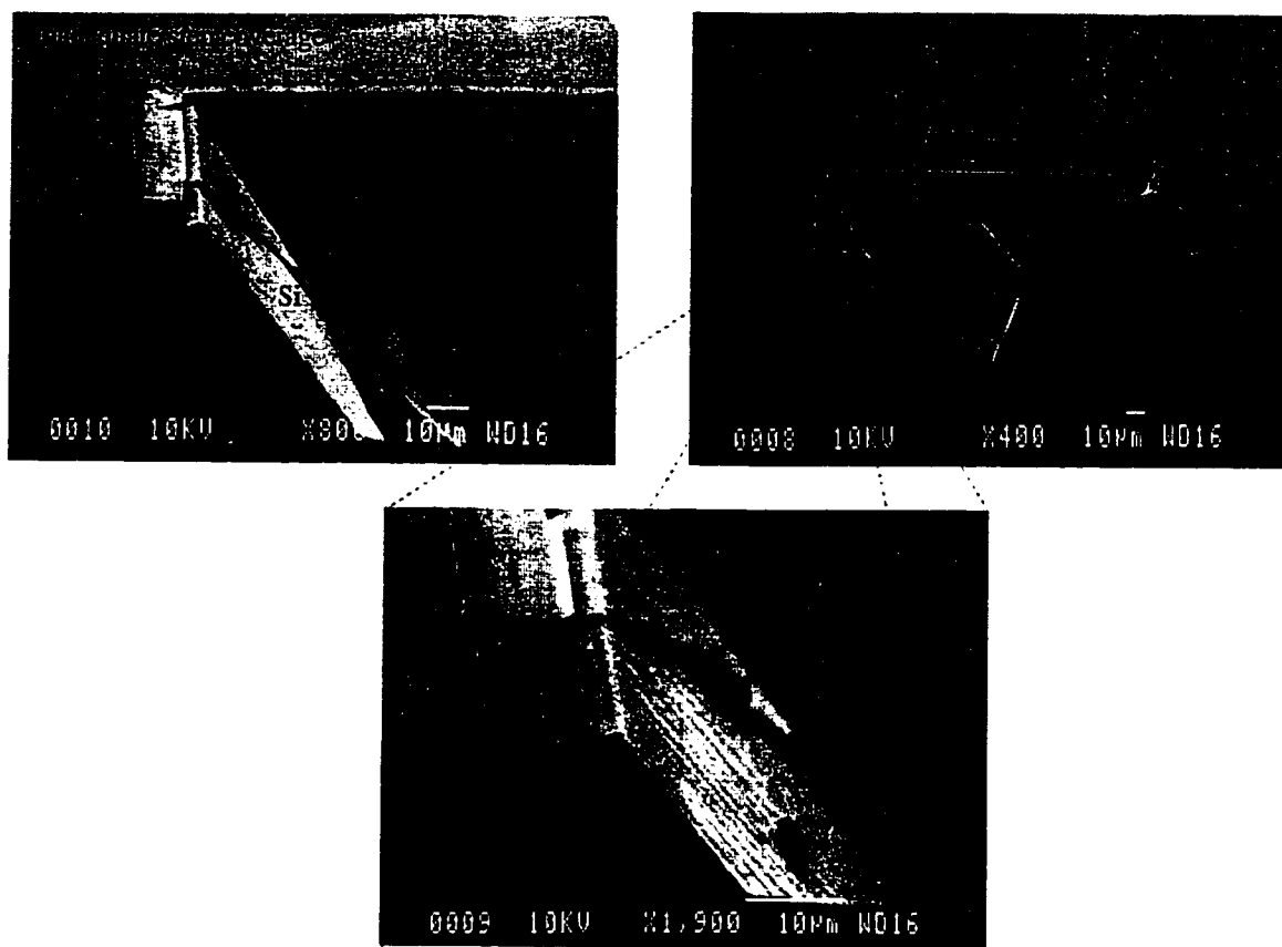
Figure 3.12: SEM photographs illustrating step coverage issues with shadow mask method of via metallization.
