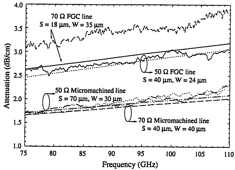
(b) Measured and modeled attenuation.
