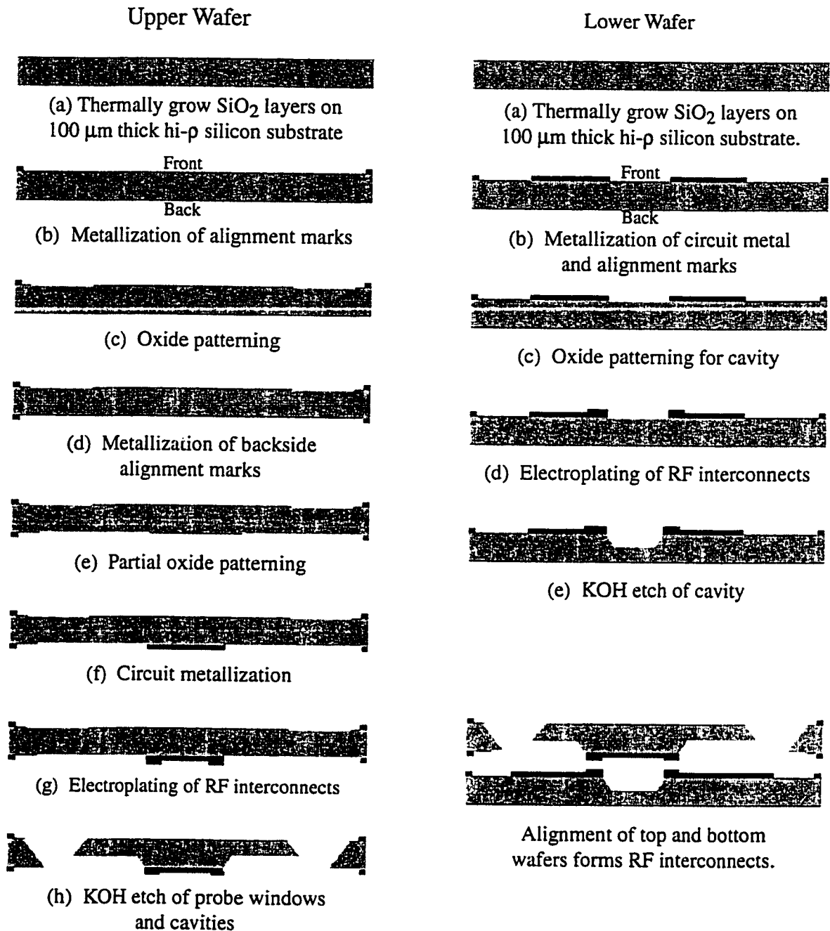
Figure 4.7: Fabrication of Upper and Lower 100\text{ }\mu\text{m} silicon wafers for RF interconnects
