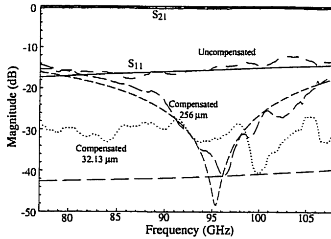
Figure A.10: Measured and modeled results for 40\ \mu\text{m} air bridges with L1 = 32.13\ \mu\text{m} and L2 = 256\ \mu\text{m} high impedance sections as compared to uncompensated. 50\ \Omega line dimensions 40\text{-}24\text{-}106\ \mu\text{m} . 70\ \Omega line dimensions 18\text{-}35\text{-}100\ \mu\text{m} .
