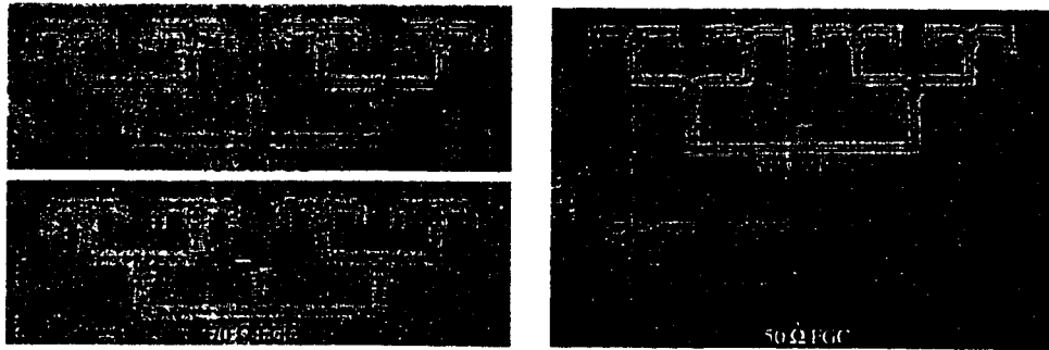
Figure 5.21: Photographs of fabricated 1:8 combining networks consisting of 1 reactive tee, 6 Wilkinsons, and 14 right angle bends.
