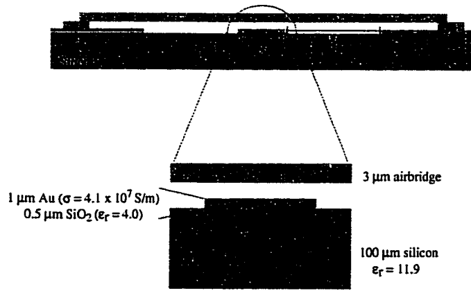
Figure 3.21: Cross section of air bridge over FGC line.
