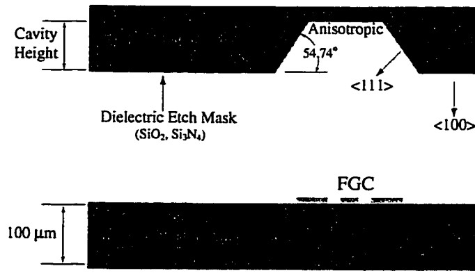
(a) Schematic of micromachined cavity over FGC line
