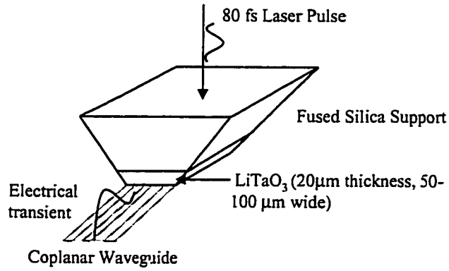
Figure D.9: Electro-optic crystal.
