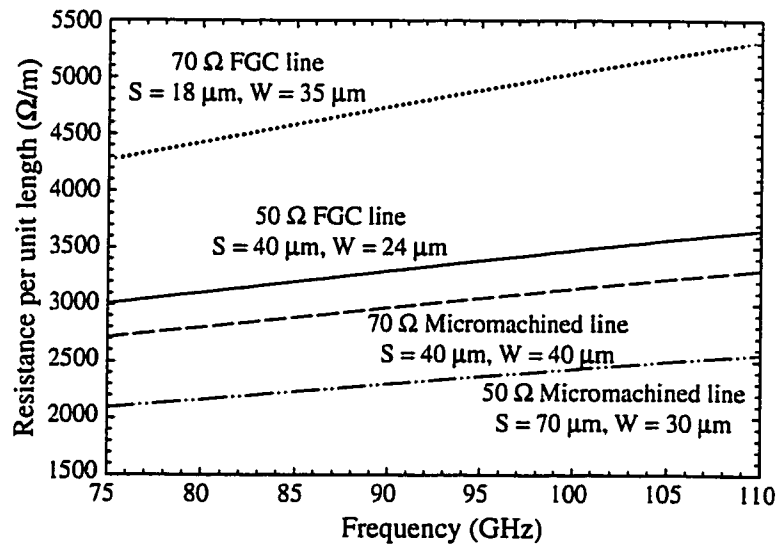
Figure 5.11: Modeled resistance per unit length versus frequency for four aspect ratios.
