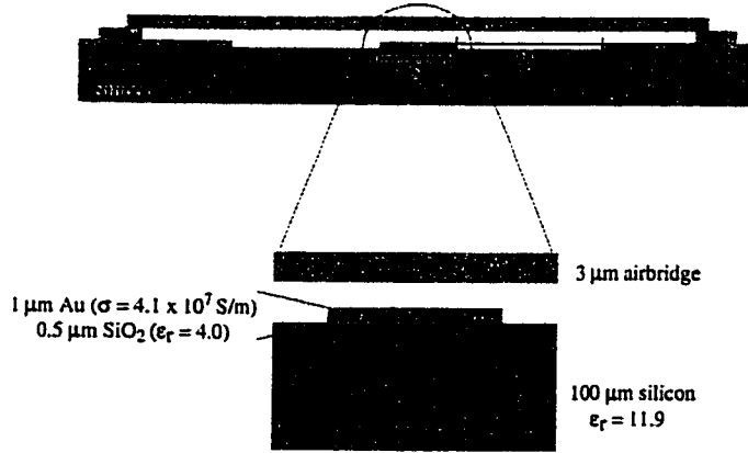
Figure A.3: Cross-section of FGC line with air bridge.
