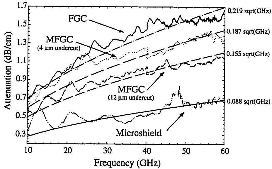
Figure 2.11: Attenuation vs. Frequency. All FGC lines have W=80 \mu\text{m} , S=40 \mu\text{m} . The micromachined lines have undercut of 4 and 12 \mu\text{m} , and the microshield line has a 75 \Omega characteristic impedance with 250 \mu\text{m} center conductor and 25 \mu\text{m} apertures.
