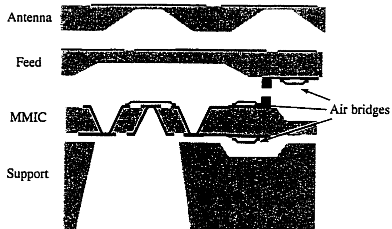
Figure 6.23: Illustration showing relative placement of air bridges on power cube layers.
