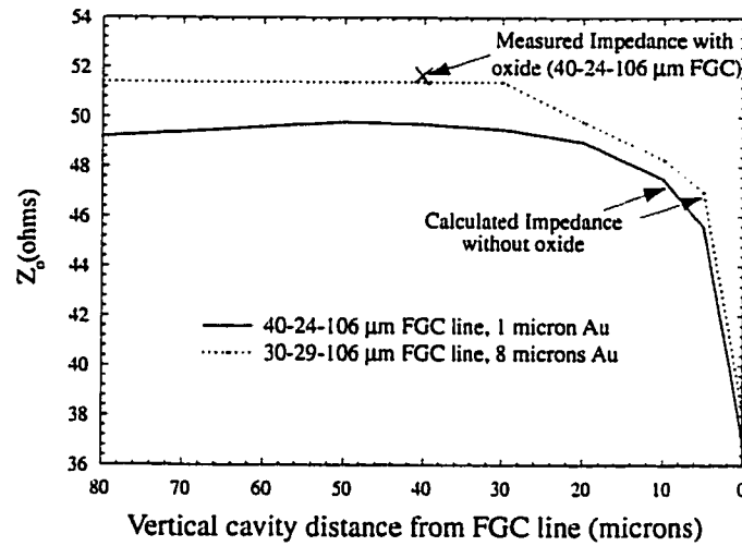
(b) Effect of cavity height on FGC line.
