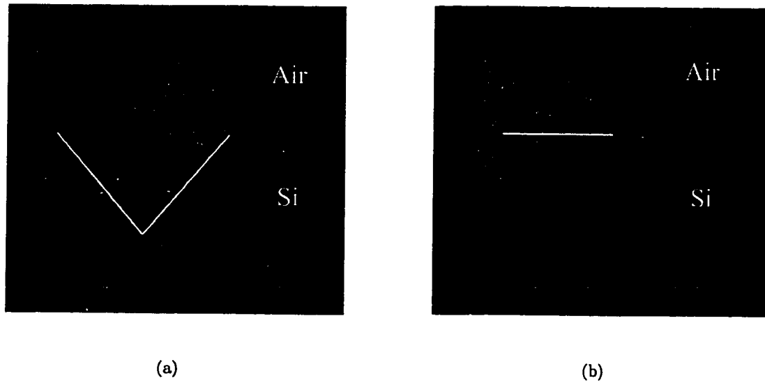
Figure 2.9: Simulated electric field distribution of (a) MFGC line (b) conventional FGC.
