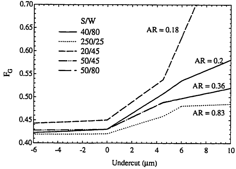
Figure 2.6: F_G versus Undercut( \mu\text{m} ) for five different aspect ratios( \text{AR}=\text{S}/(\text{S}+2\text{W}) ), where S is the center conductor width and W is the aperture width.
