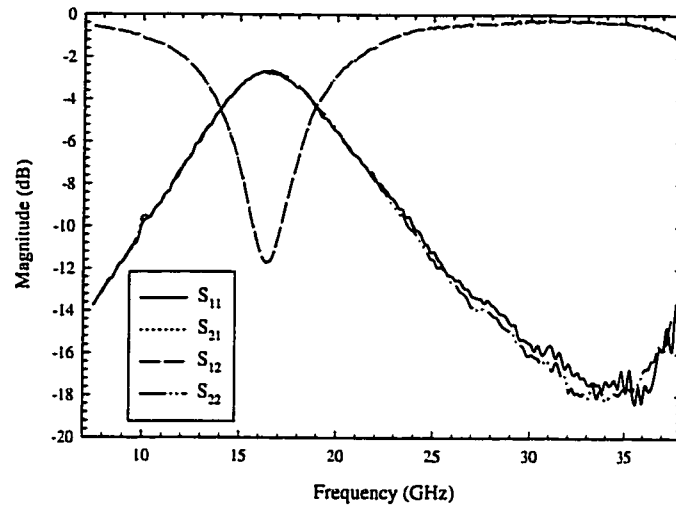
Figure D.7: Measured S-parameters for open stub.
