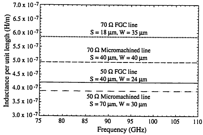
Figure 5.12: Modeled inductance per unit length versus frequency for four aspect ratios.
