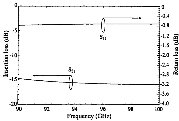
Figure 4.21: S-parameter simulations of RF wafer-to-wafer transition with 2 \mu\text{m} vertical separation.
