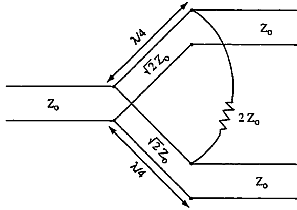
Figure 5.1: Equivalent transmission line circuit for Wilkinson power divider.
