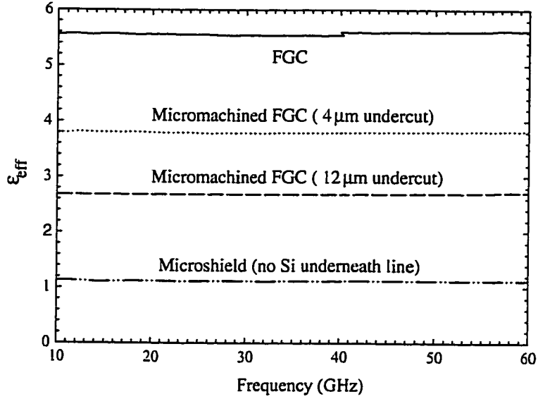
Figure 2.8: \epsilon_{eff} vs. frequency for a 80-40-80 \mu\text{m} MFGC with 4 and 12 \mu\text{m} undercut. Comparison with conventional FGC of same dimensions and 75 \Omega microshield with S/W of 250/25 \mu\text{m} .
