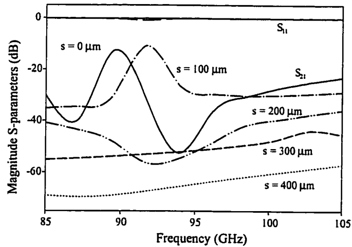
(b) Simulated S-parameters
