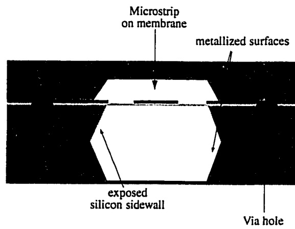
Figure 1.11: Alternative version of membrane microstrip [11].
