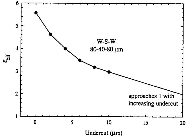
Figure 2.14: Effective dielectric constant versus. undercut for MFGC with W-S-W equal to 80-40-80 \mu\text{m} .
