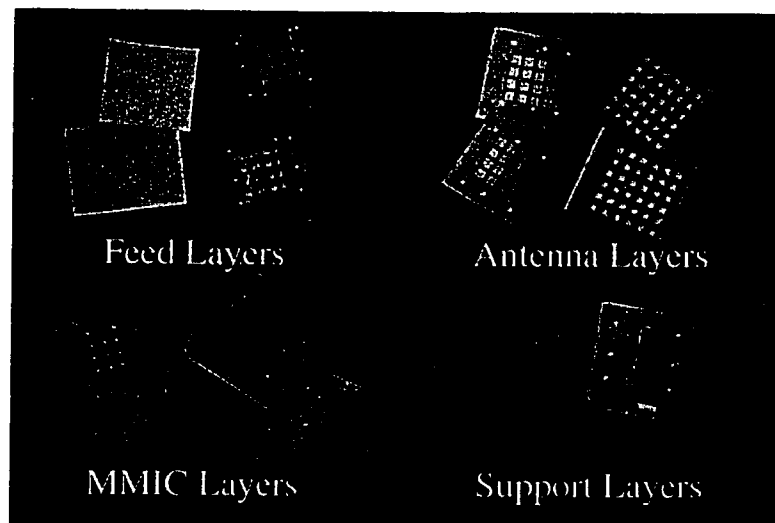
Figure 6.16: Photos of fabricated power cube layers.
