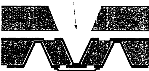
(g) Metallization of vias on other side using shadow mask (1 \mu\text{m} evaporated Au).
