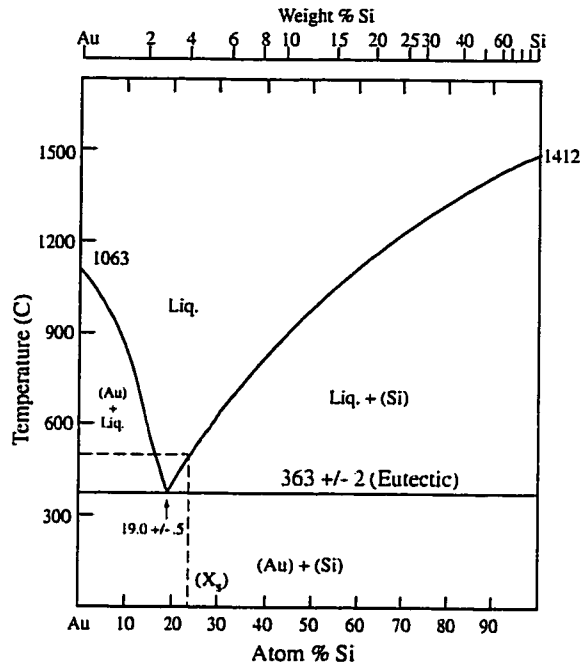
Figure 4.9: Phase diagram for Au-Si [37]
