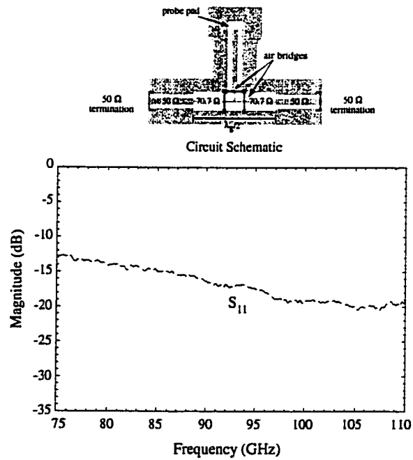
Figure 6.28: Measured tee with 50\ \Omega terminations.
