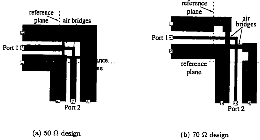
Figure 5.7: Schematics of right angle bends as simulated in IE3D [132]: a) 50 \Omega b) 70 \Omega .
