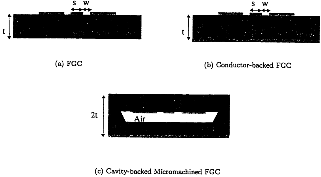
Figure 6.6: Line architectures for multilayer circuits.
