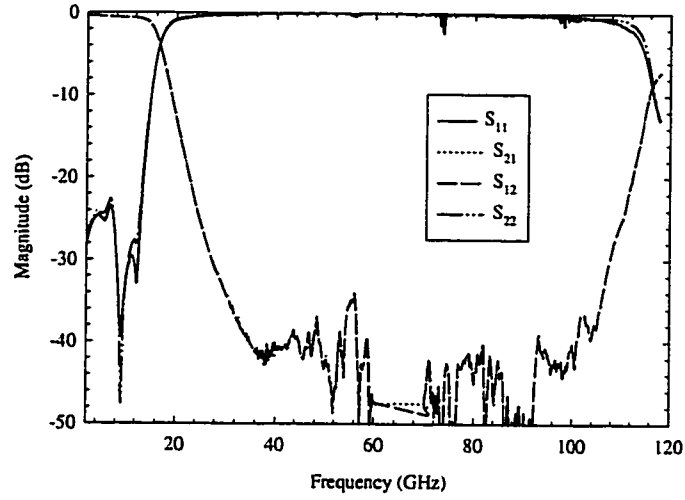
Figure D.3: S-parameters for low-pass filter measurement.
