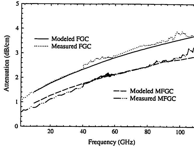
Figure 2.22: Attenuation vs. frequency for 45-20-45 \mu\text{m} line comparing measured and modeled data.
