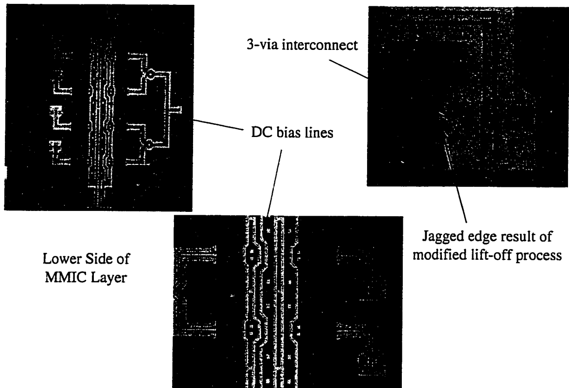
Figure 6.19: Photos of lower side MMIC layer.
