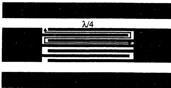
Figure D.6: Double-folded short-end series stub.
