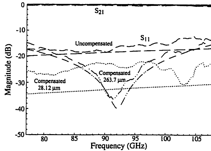
Figure A.9: Measured and modeled results for 30 \mu\text{m} air bridges with L1 = 28.12 \mu\text{m} and L2 = 263.7 \mu\text{m} high impedance sections as compared to uncompensated. 50 \Omega line dimensions 40\text{-}24\text{-}106 \mu\text{m} . 70 \Omega line dimensions 26\text{-}52\text{-}100 \mu\text{m} .
