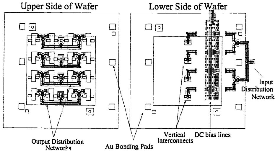
Figure 6.13: Upper and lower sides of MMIC layer, illustrating complexity of fabrication.
