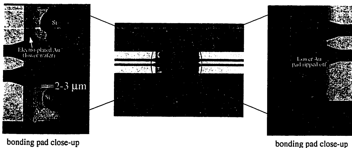
Figure 4.16: Photograph of bonded sample after wafers pulled apart showing bonding and alignment.
