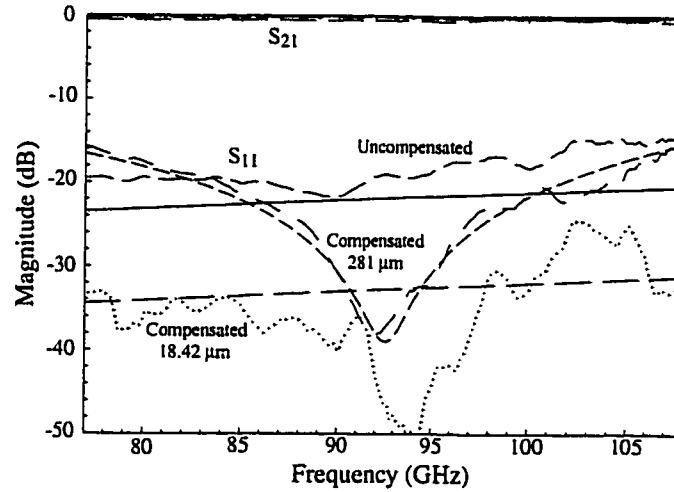
Figure A.7: Measured and modeled results for 20 \mu\text{m} air bridges with L1 = 18.42 \mu\text{m} and L2 = 281 \mu\text{m} high impedance sections as compared to uncompensated. 50 \Omega line dimensions 40\text{-}24\text{-}106 \mu\text{m} . 70 \Omega line dimensions 26\text{-}52\text{-}100 \mu\text{m} .
