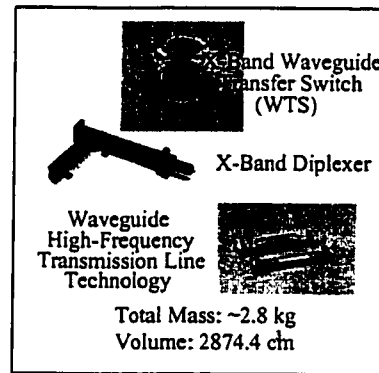
Figure 1.1: Traditional waveguide components for satellite communications at X-band (8-12 GHz).
