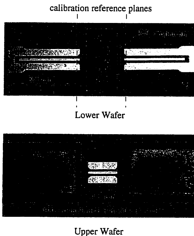
Figure 4.13: Photograph of RF wafer-to-wafer transition showing placement of calibration reference planes.
