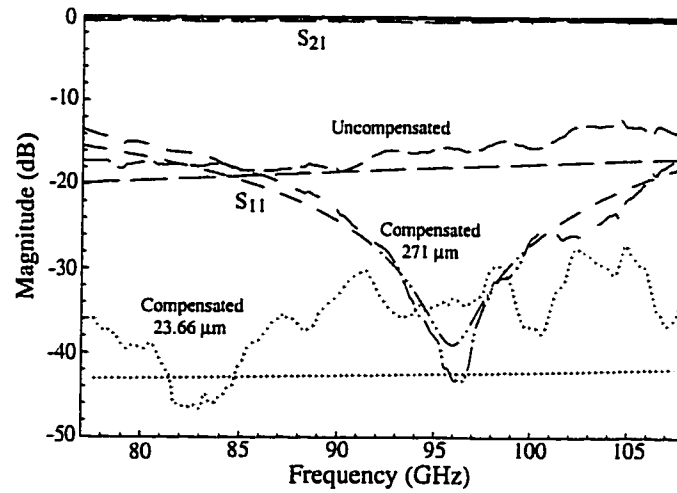
Figure A.8: Measured and modeled results for 30\ \mu\text{m} air bridges with L1 = 23.66\ \mu\text{m} and L2 = 271\ \mu\text{m} high impedance sections as compared to uncompensated. 50\ \Omega line dimensions 40-24-106 \mu\text{m} . 70\ \Omega line dimensions 18-35-100 \mu\text{m} .
