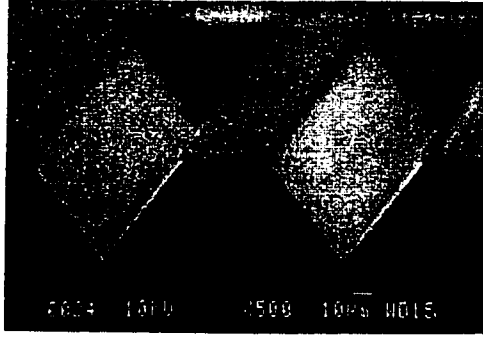
Figure 2.3: Anisotropically etched Si.
