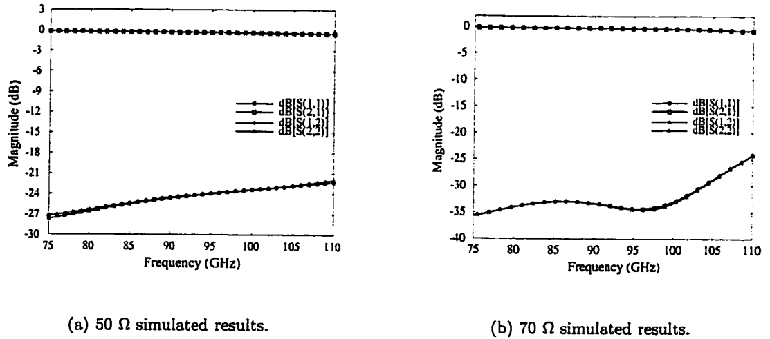
Figure 5.8: S-parameters of right angle bends as simulated in IE3D [132]: a) 50 \Omega b) 70 \Omega .
