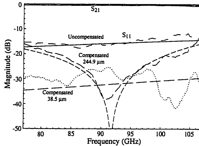
Figure A.11: Measured and modeled results for 40 \mu\text{m} air bridges with L1 = 38.5 \mu\text{m} and L2 = 244.9 \mu\text{m} high impedance sections as compared to uncompensated. 50 \Omega line dimensions 40\text{-}24\text{-}106 \mu\text{m} . 70 \Omega line dimensions 26\text{-}52\text{-}100 \mu\text{m} .
