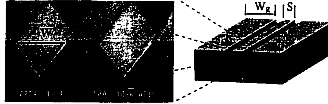
Figure 5.10: MFGC geometry.
