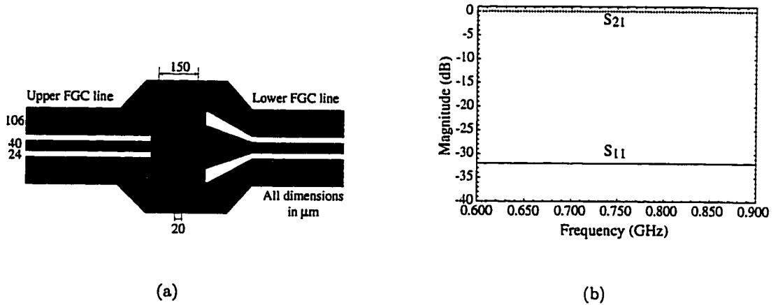
Figure 3.2: (a) Schematic. (b) Simulated S-parameters for a single 3-via interconnect from 600-900 MHz.
