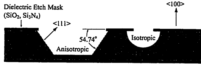
Figure 1.5: Cross-section of micromachined Si wafer.
