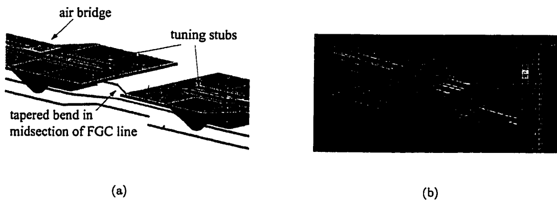
Figure 3.6: (a) Schematic of improved design with tuning stub, air bridge, and tapered bend. (b) IE3D plot of current distribution for 3-via interconnect.
