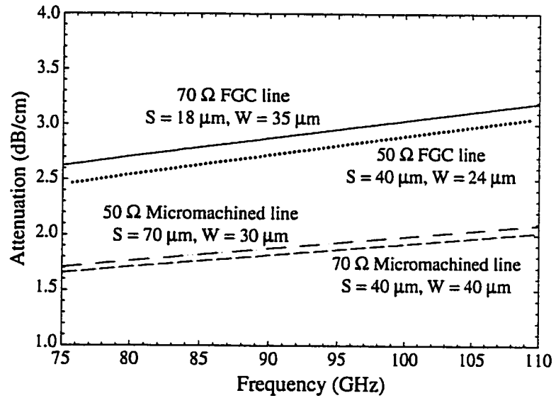
Figure 5.13: Modeled attenuation versus frequency showing expected loss improvement utilizing silicon micromachining.
