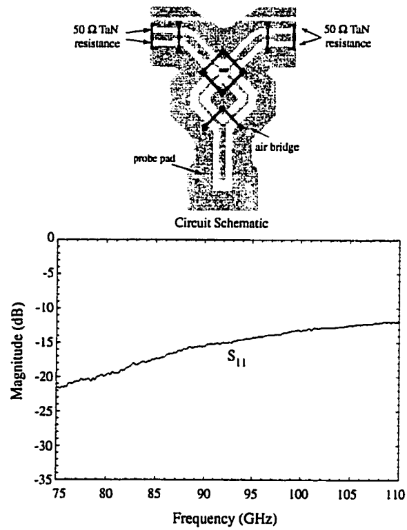
Figure 6.29: Measured input reflection coefficient of Wilkinson power divider with 50\ \Omega terminations.
