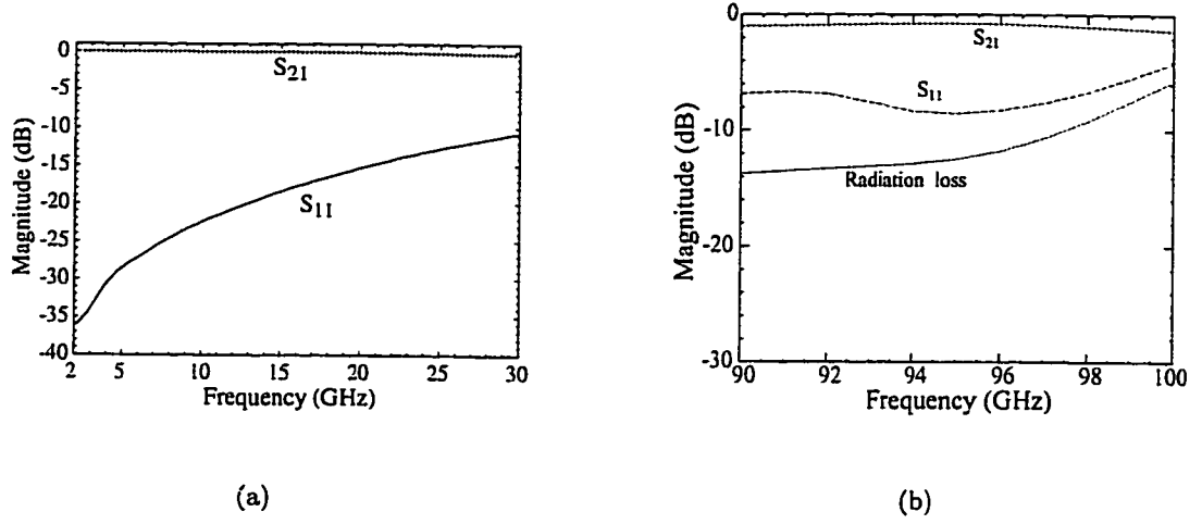
Figure 3.3: Simulated S-parameters for single three-via interconnect: (a) 2-30 GHz (b) 90-105 GHz.
