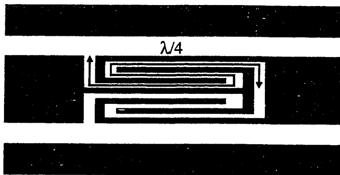
Figure D.5: Double-folded open-end series stub.
