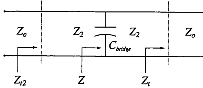
Figure 5.9: Equivalent circuit for air bridge.
