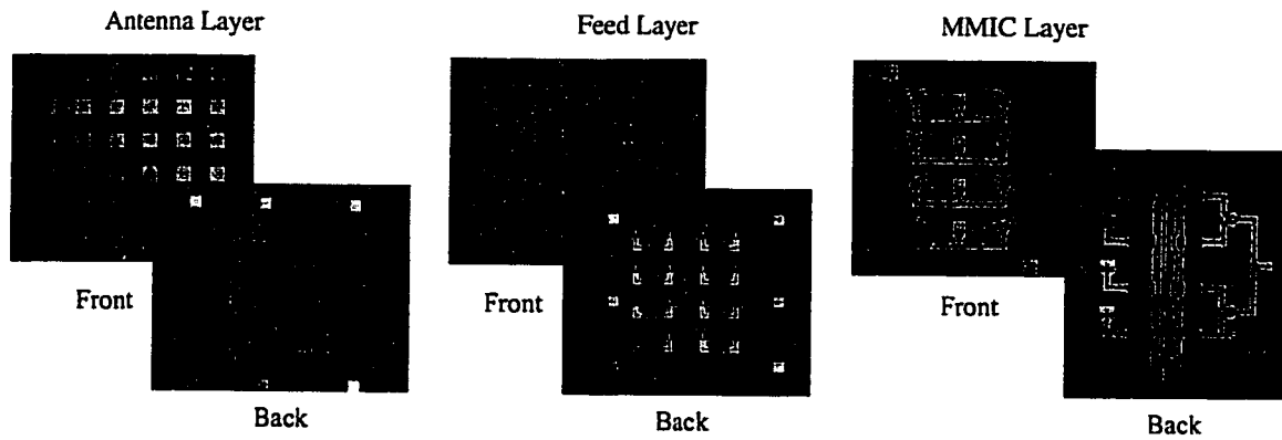
Figure 6.17: Photos of fabricated power cube layers.
