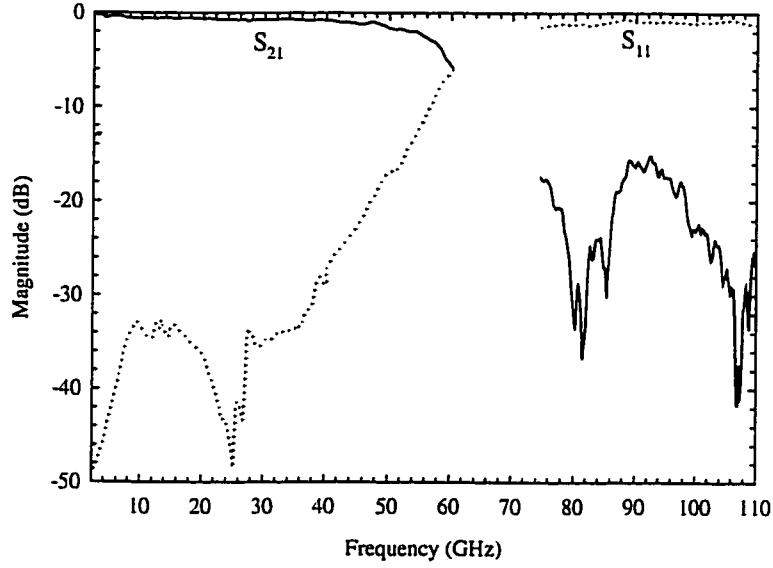
Figure 2.17: Measured scattering parameters for the micromachined low pass filter of Figure 2.16.
