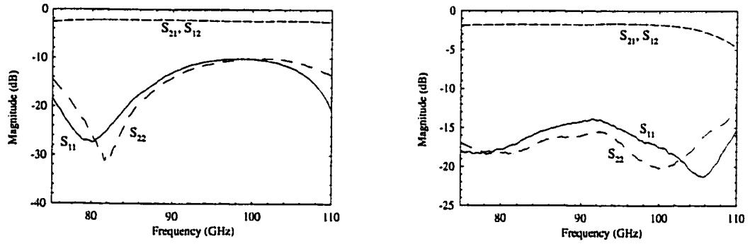
Figure 3.20: Measured S-parameters of back-to-back vertical interconnects: a) 934 \mu\text{m} midsection, 230 \mu\text{m} stub, and 100 \mu\text{m} air bridge. b) 734 \mu\text{m} midsection, 240 \mu\text{m} stub, and 130 \mu\text{m} air bridge.
