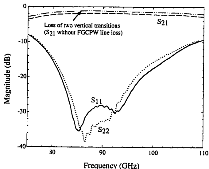
Figure 3.17: Measured S-parameters of back-to-back vertical interconnect transition.
