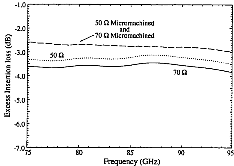
Figure 5.22: Modeled insertion loss for 1:8 combining networks.
