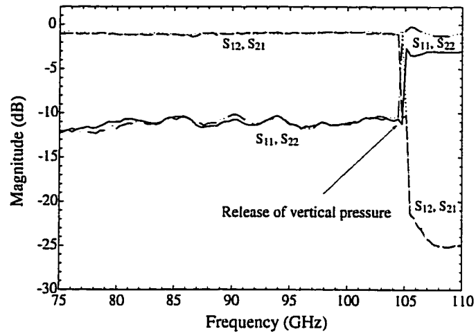
Figure 4.20: S-parameter measurements of unbonded RF wafer-to-wafer transition.
