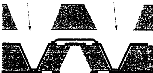
(f) Metallization of vias by evaporation using shadow mask.
