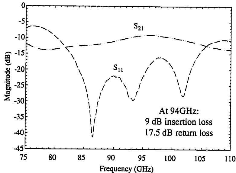
(b) Measured passive component combination: via-distribution network-via.
