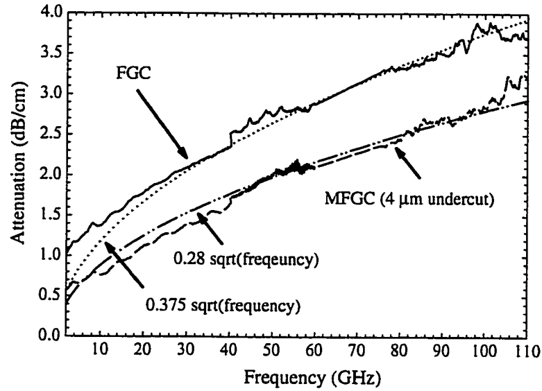
Figure 2.10: Attenuation vs. Frequency for FGC line with 20 \mu\text{m} center conductor and 45 \mu\text{m} apertures compared with micromachined line of same geometry.
