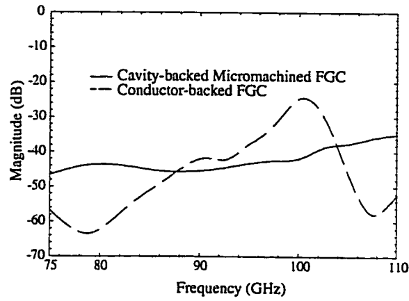
Figure 6.10: Simulation of architectures of Figure 6.9.
