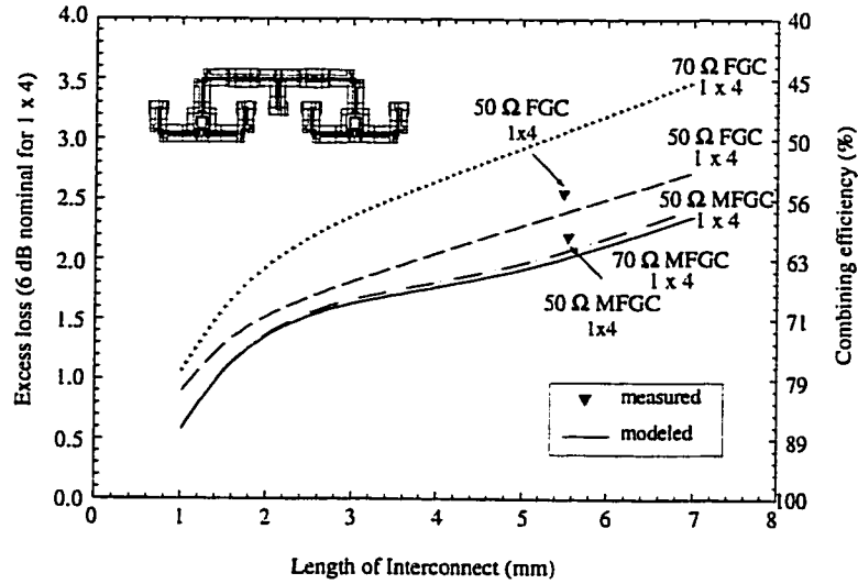
Figure 5.19: Excess loss and combining efficiency versus signal path length for micromachined and unmicromachined FGC lines.
