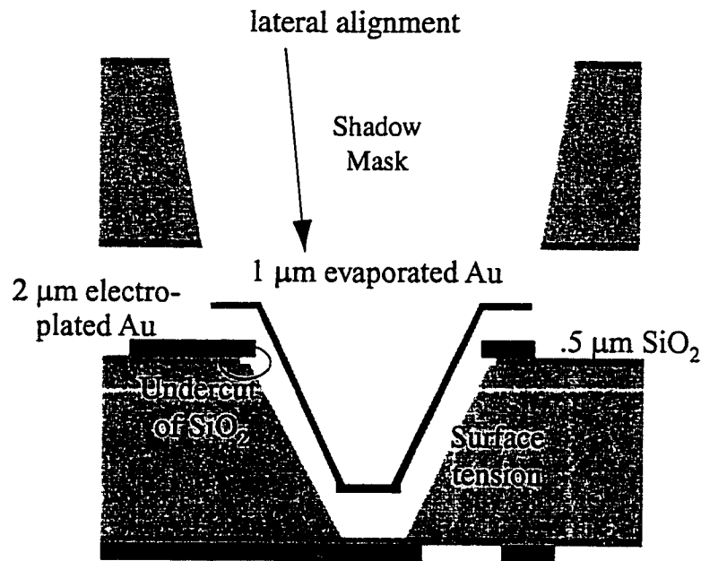
Figure 3.10: Illustration of fabrication problems.
