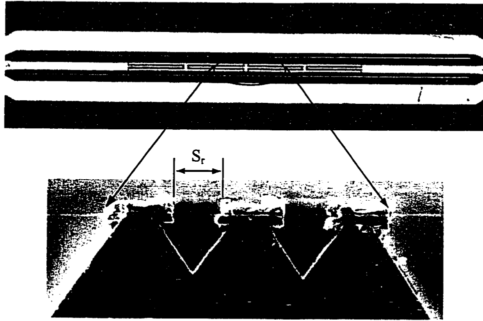
Figure 2.16: Micromachined four resonator band-pass filter with W = 45 \mu\text{m} , S = 50 \mu\text{m} , and 4 \mu\text{m} undercut.
