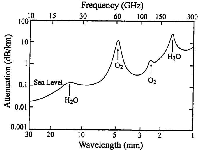
Figure 1.4: Average atmospheric absorption as a function of frequency and wavelength [7].
