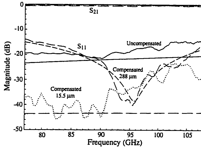
Figure A.6: Measured and modeled results for 20 \mu\text{m} air bridges with L_1 = 15.5 \mu\text{m} and L_2 = 288 \mu\text{m} high impedance sections as compared to uncompensated. 50 \Omega line dimensions 40-24-106 \mu\text{m} . 70 \Omega line dimensions 18-35-100 \mu\text{m} .
