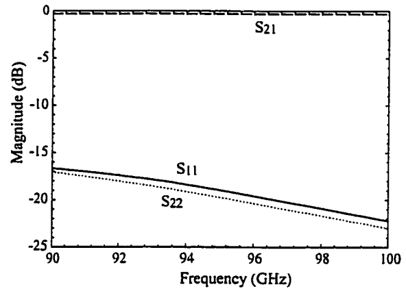
(b) HFSS Simulation
