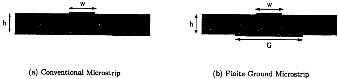
Figure 1.7: Microstrip
