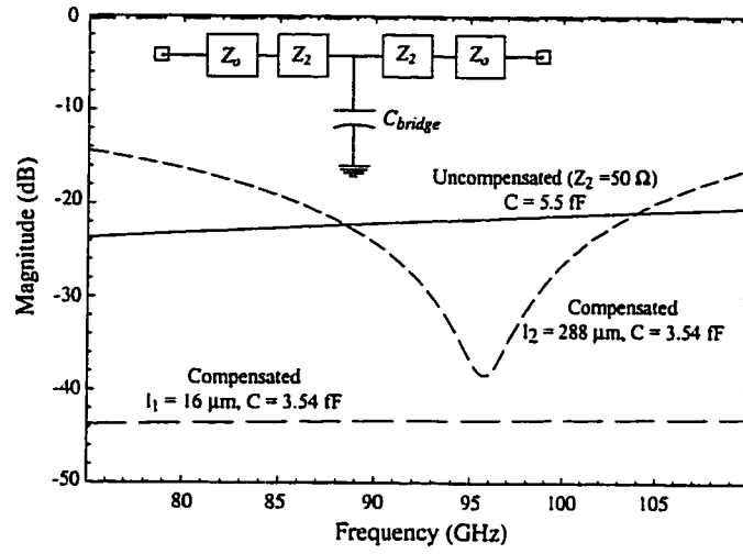
Figure A.5: Libra simulation of uncompensated air bridge and compensated air bridge with two different high impedance section lengths.
