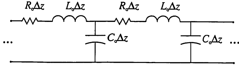
Figure 2.18: Lumped-element equivalent circuit for an incremental length of transmission line.
