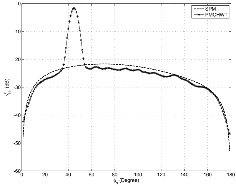
(b) \sigma_{f_2} = 0.05
