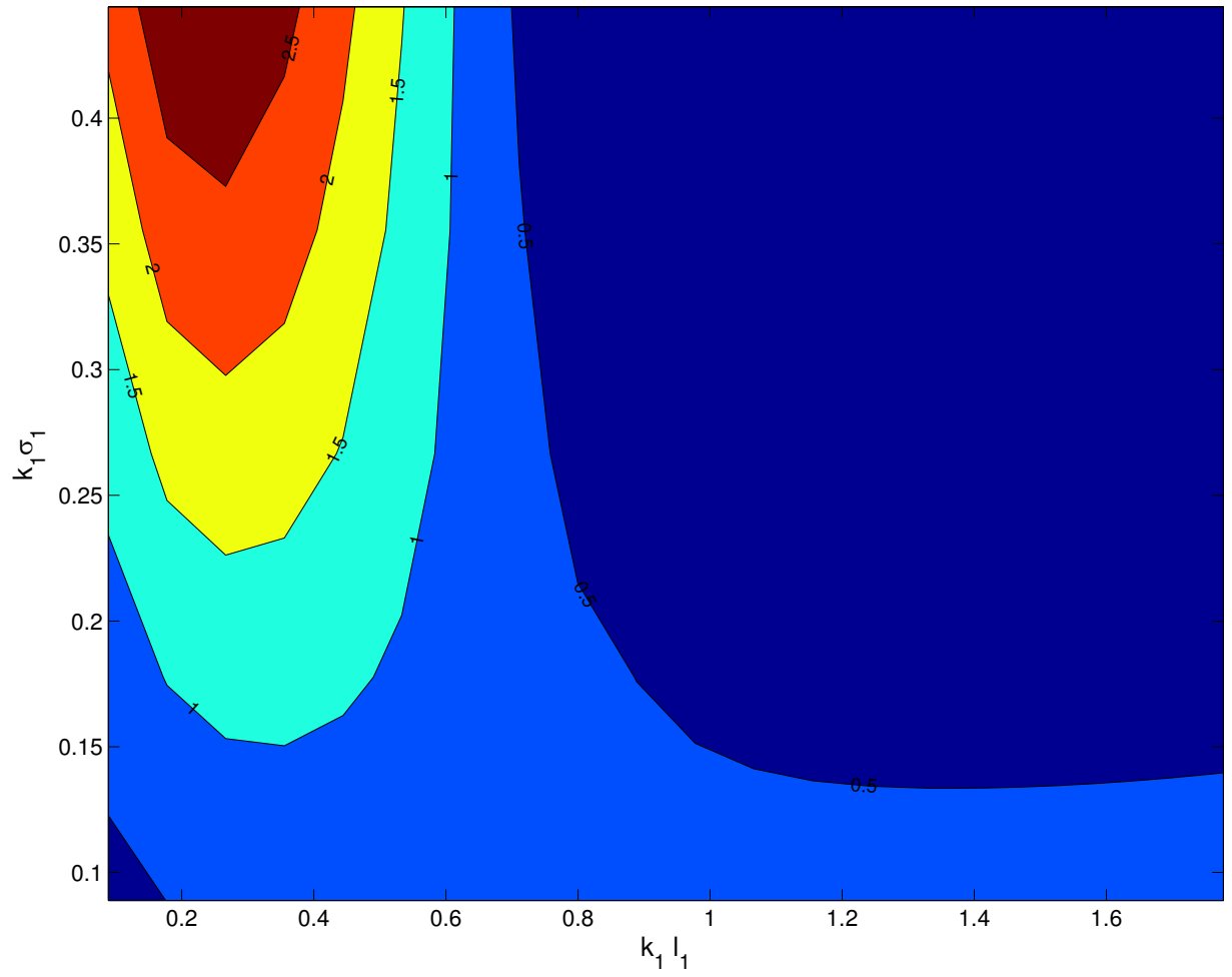
Figure 3.16: Contour plot of |\gamma_{\text{MoM}} - \gamma_{\text{SPM}}| for Case 2. Both of the parameters \gamma_{\text{MoM}} and \gamma_{\text{SPM}} are expressed in dB.
