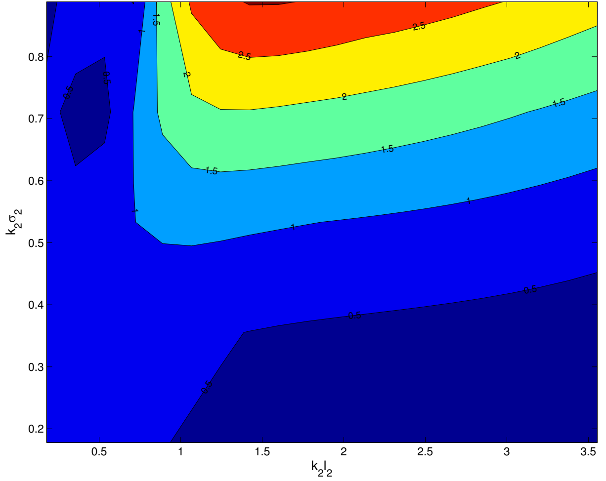
Figure 3.19: Contour plot of |\gamma_{\text{MoM}} - \gamma_{\text{SPM}}| for Case 5. Both of the parameters \gamma_{\text{MoM}} and \gamma_{\text{SPM}} are expressed in dB. This case shows how the multiple scattering processes between the layers could lead to counter intuitive results for the region of validity.
