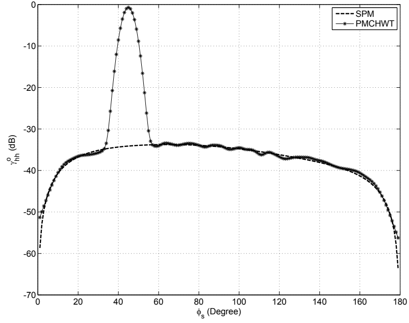
(a) \sigma_{f_2} = 0.01
