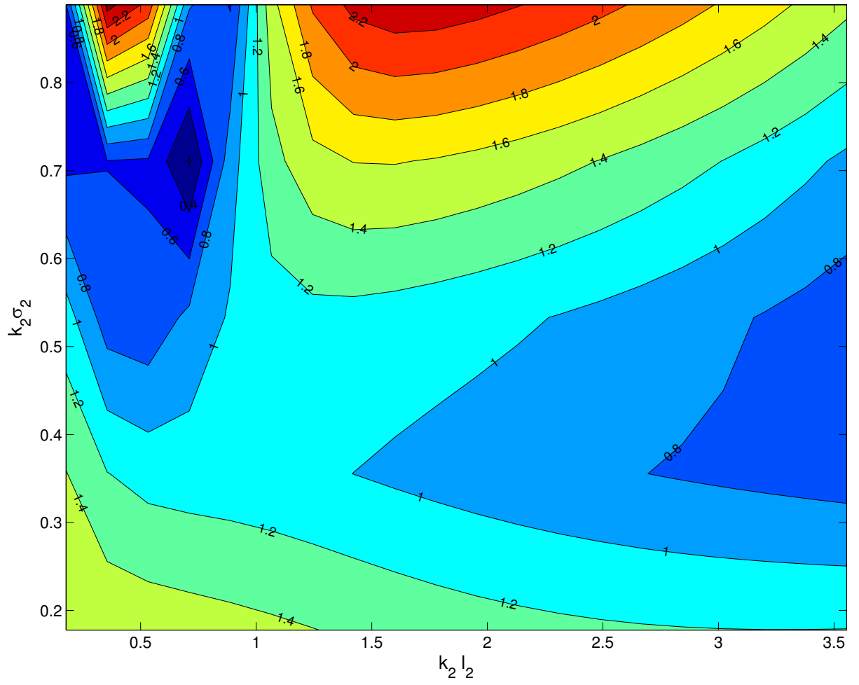
Figure 3.17: Contour plot of |\gamma_{\text{MoM}} - \gamma_{\text{SPM}}| for Case 3. Both of the parameters \gamma_{\text{MoM}} and \gamma_{\text{SPM}} are expressed in dB.
