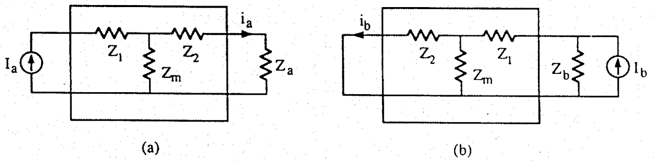
Fig. 2. Two complementary T-networks.
