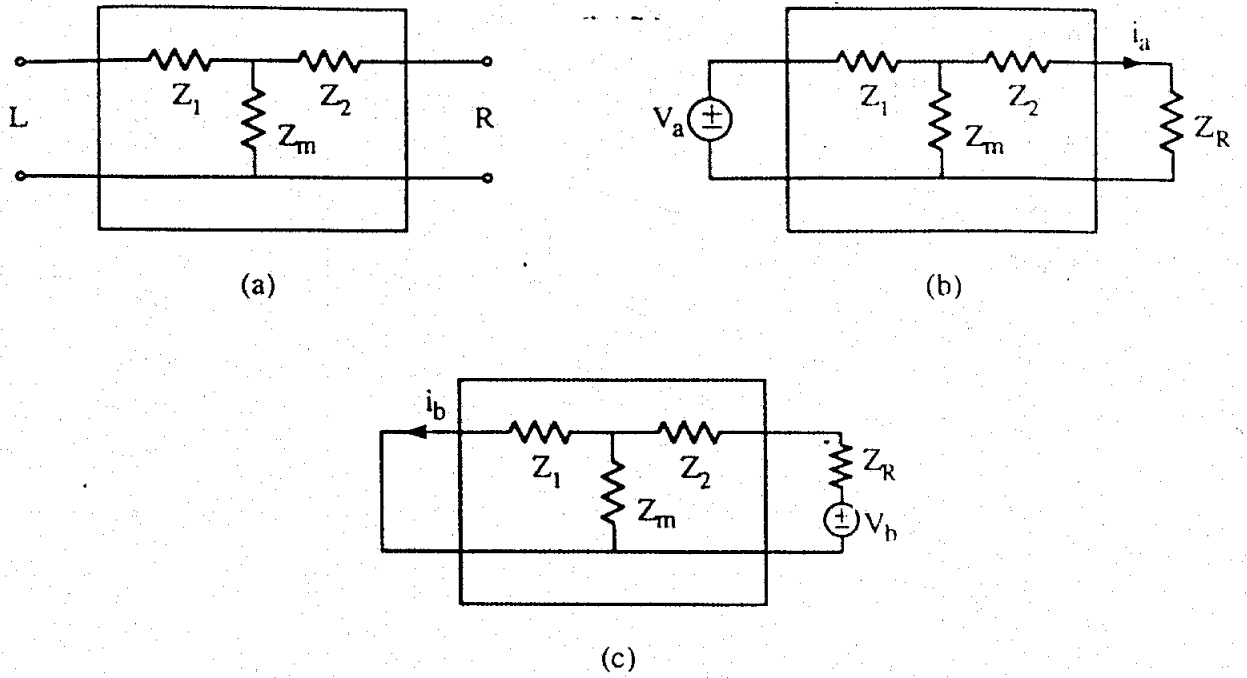
Fig. 1. A two-port T-network with two different driving conditions.
