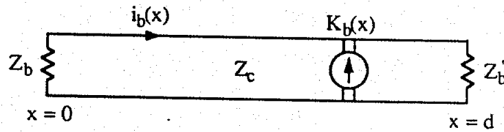
(b) An identical section of line terminated by two load impedances Z_b and Z'_b .
