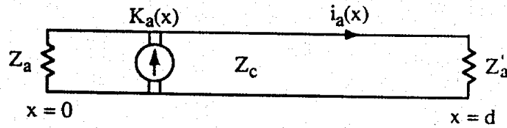
(a) A section of transmission line terminated by two load impedances Z_a and Z'_a .
