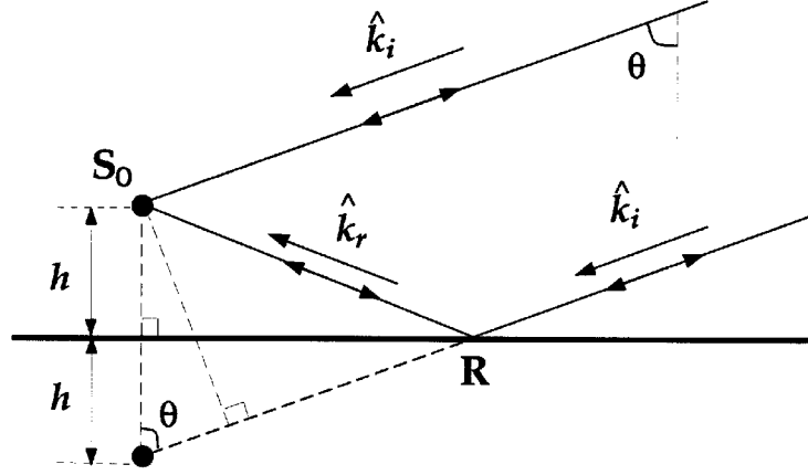
Figure 5.2: An object above a ground plane illuminated by a \Delta k -radar.
