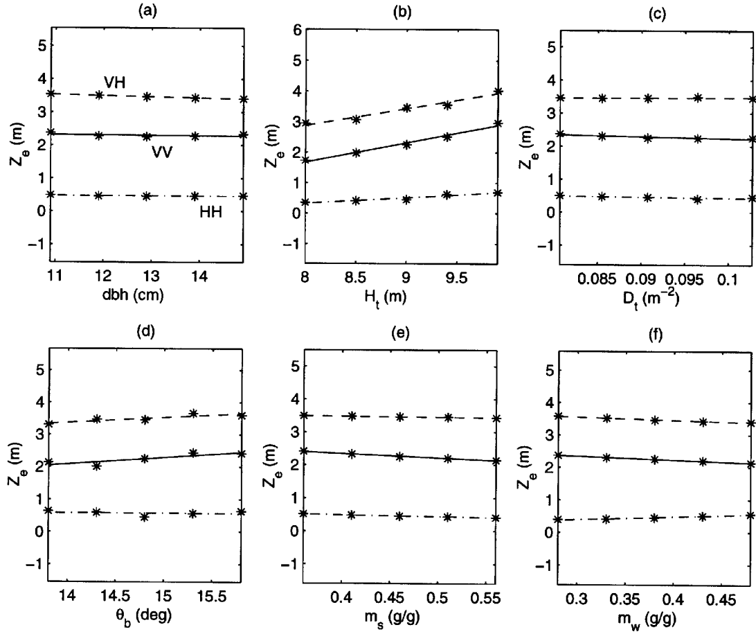
Figure 6.1: The sensitivity analysis of the C-band polarimetric scattering phase center height as a function of the physical parameters: (a) trunk diameter, (b) tree height, (c) tree density, (d) branching angle, (e) soil moisture, and (f) wood moisture, simulated at incidence angle \theta = 25^\circ .
