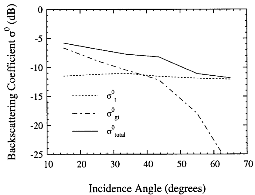
Figure 4.8: Contribution of different scattering components ( \sigma_t^0 and \sigma_{gt}^0 ) to the overall backscattering coefficient ( \sigma_{total}^0 ) as a function of incidence angle.
