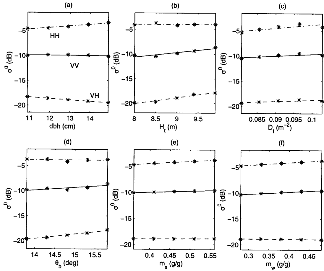
Figure 6.2: The sensitivity analysis of the C-band polarimetric backscattering coefficient as a function of the physical parameters: (a) trunk diameter, (b) tree height, (c) tree density, (d) branching angle, (e) soil moisture, and (f) wood moisture, simulated at incidence angle \theta = 25^\circ .
