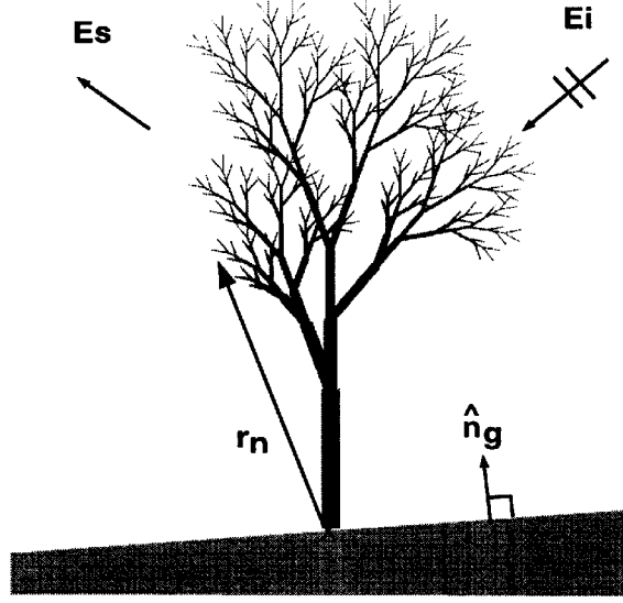
Figure 4.1: Scattering from a cluster of scatterers above a tilted ground plane.
