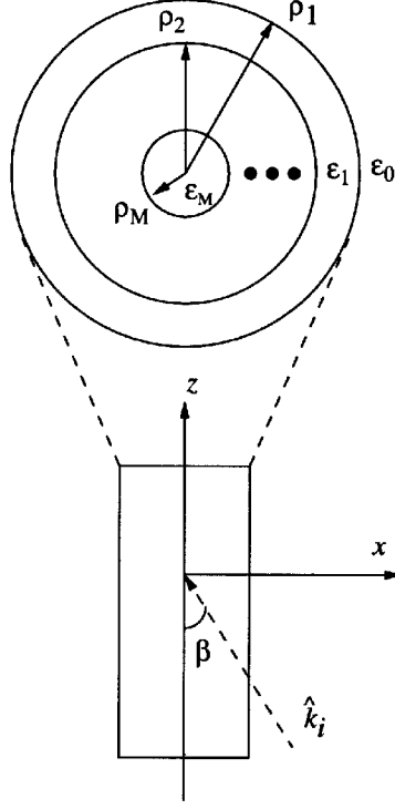
Figure 3.3: Geometry and composition of a finite stratified cylinder (top-view and side-view).
