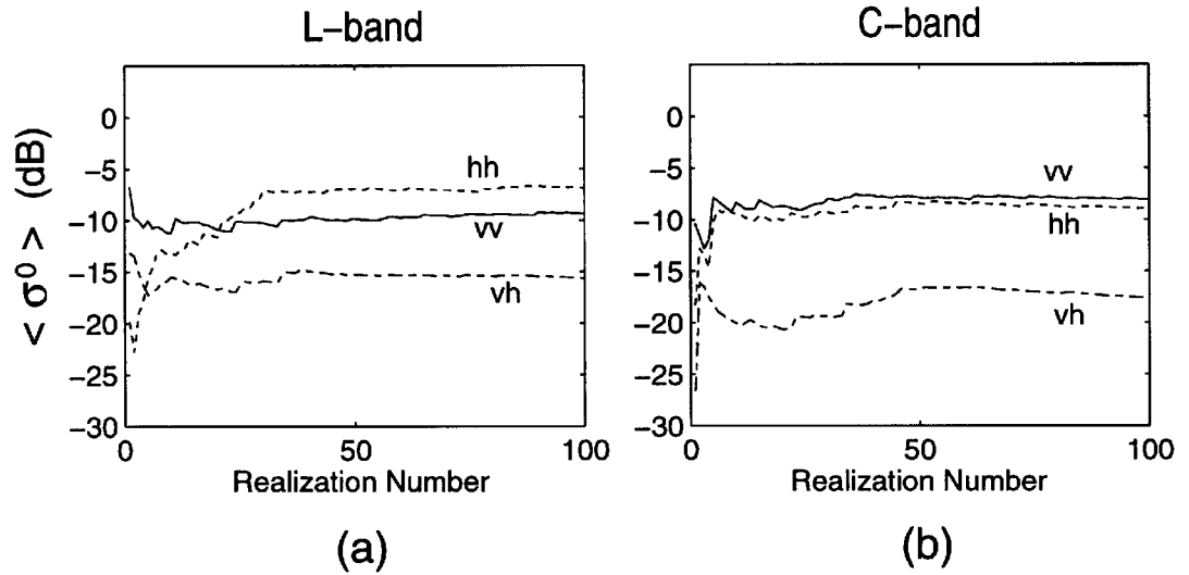
Figure 4.6: Convergence behavior of the Monte Carlo simulation for Stand 31 at L-band(a) and C-band (b) at incidence angle \theta_i = 30^\circ .
