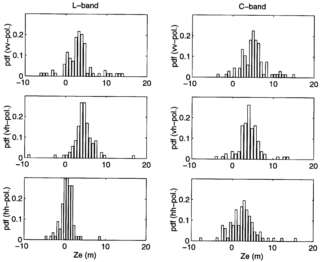
Figure 5.11: PDF of the scattering phase center height of Stand 22 (red pine) at \theta_i = 45^\circ as a function of frequency and polarization.
