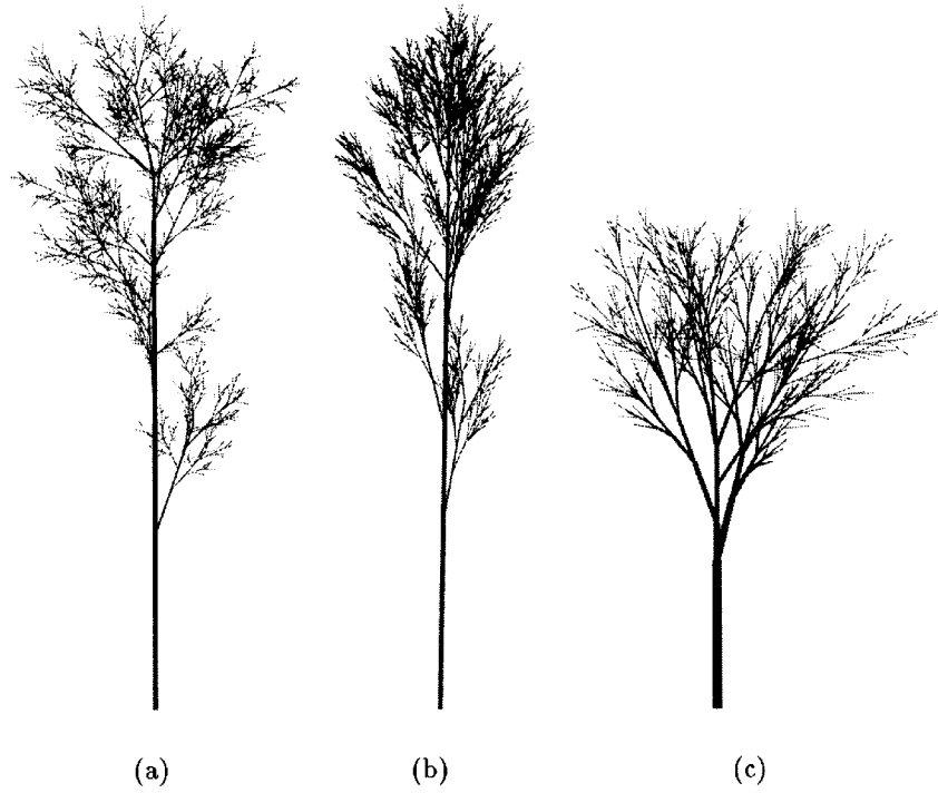
Figure 4.13: Tree structures generated for (a) Stand 31, (b) Case 1, and (c) Case 2.
