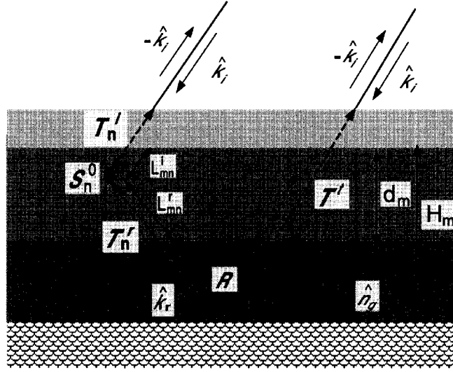
Figure 4.3: Extinction of a coherent wave in random media.
