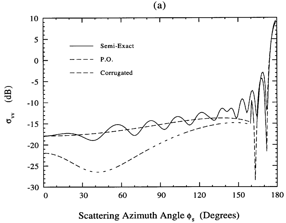
Figure 3.8: The normalized bistatic \sigma_{vv} (a) and \sigma_{hh} (b) as a function of the scattering azimuth angle \phi_s . The backscattered and forward-scattered directions are shown at \phi_s = 0^\circ and \phi_s = 180^\circ respectively. Other parameters are : \theta_i = 120^\circ, \phi_i = 180^\circ, \theta_s = 60^\circ, \theta_g = \theta_c = 0^\circ, b = 20\lambda_0, a_1 = 4\lambda_0, a_2 = 3.6\lambda_0 .
