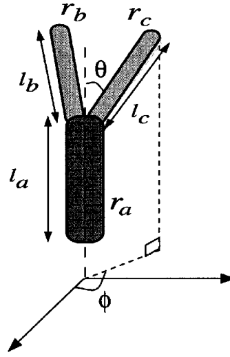
Figure 2.2: 3-D branching and branch tapering at a splitting node.
