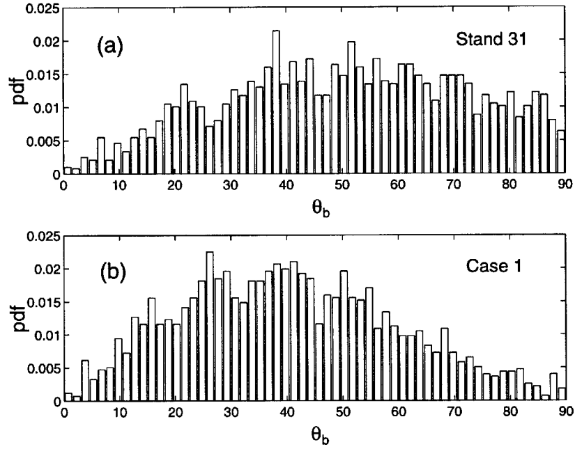
Figure 4.12: Histogram of branch orientation resulted from two branching angles : (a) \Delta\theta_b = 22^\circ \pm 5^\circ (Stand 31); (b) \Delta\theta_b = 15^\circ \pm 3^\circ (Case 1).
