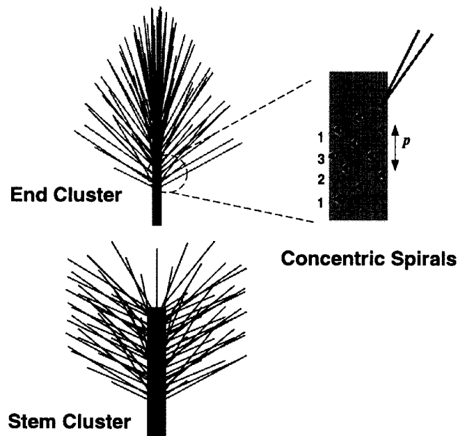
Figure 2.5: Leaf attachment schemes for the red pine: the end cluster, the stem cluster, and the leaflet on the leaf bud along three concentric spirals.
