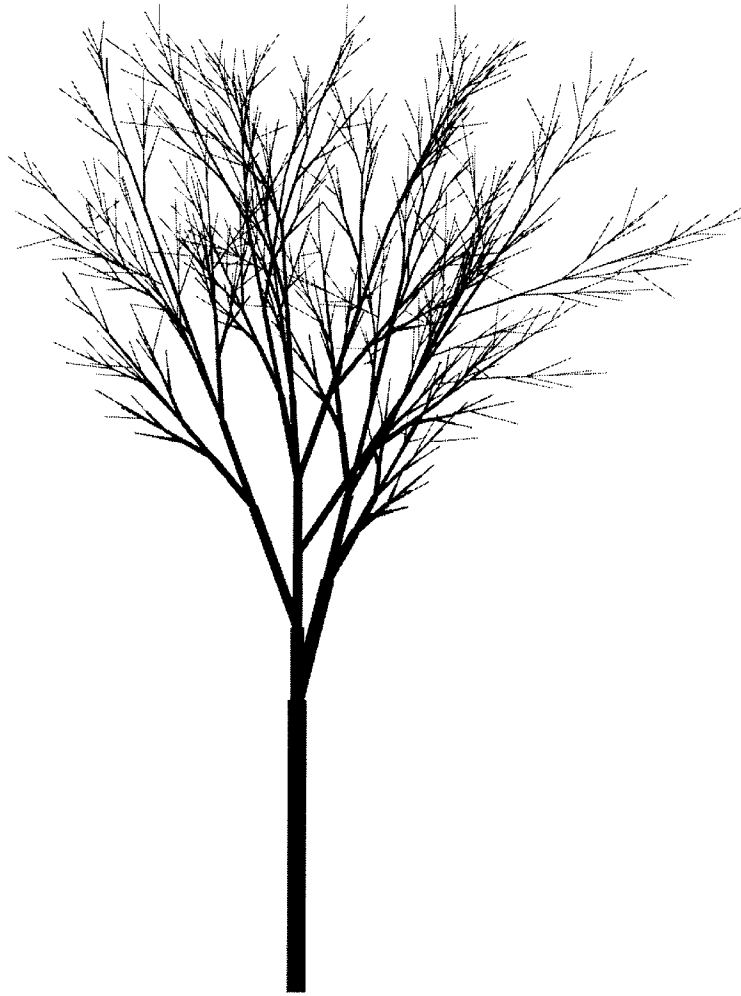
Figure 2.3: A fractal tree structure of deciduous type.
