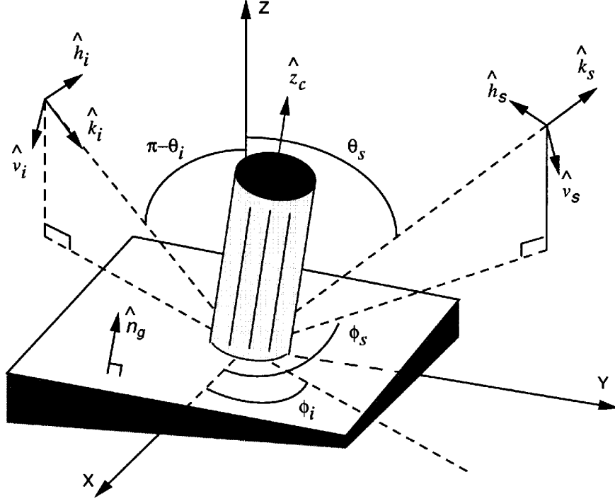
Figure 3.1: Global coordinate system and notations.
