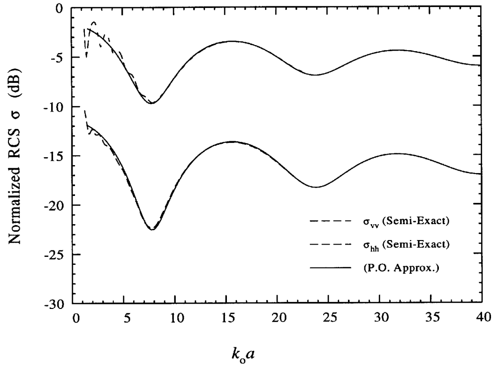
Figure 3.5: Comparison of the PO approximation with the semi-exact solution. The ratio of the interior radius a_2 and the exterior radius a_1(=a) is kept constant ( a_2/a_1 = 0.9 ). Other parameters are : b = 20\lambda_0 , \epsilon_1 = 4 + i1 , \epsilon_2 = \epsilon_g = 10 + i5 , \theta_i = 120^\circ , \phi_i = 180^\circ , \theta_s = 60^\circ , \phi_s = 0^\circ , \theta_g = \theta_c = 0^\circ .
