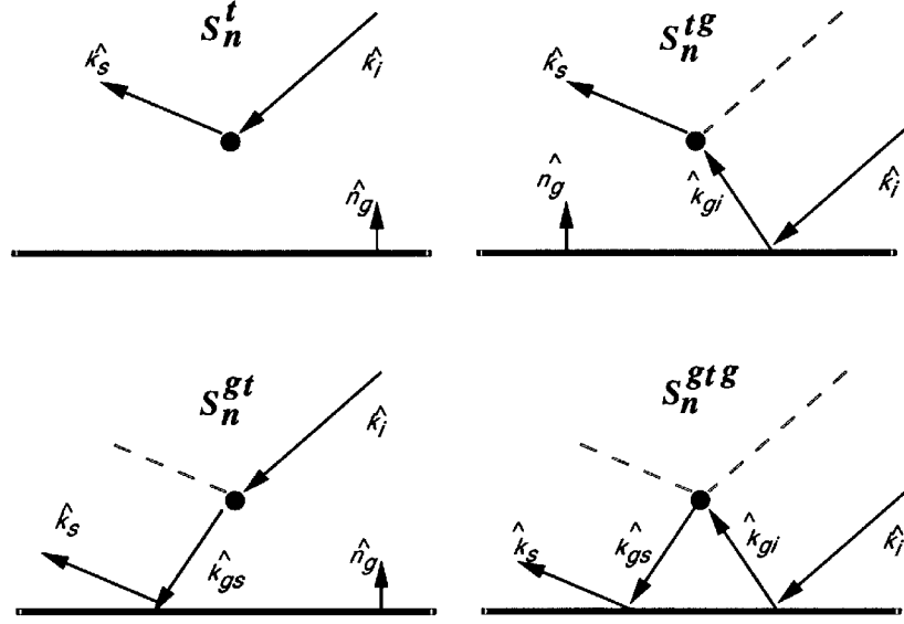
Figure 4.2: Four scattering components from an object above a tilted ground plane.
