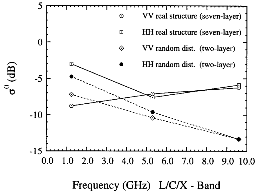
Figure 4.15: Comparison of the polarimetric backscattering coefficients at different frequency bands (L, C, and X).
