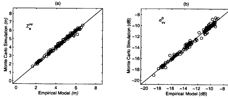
Figure 6.4: A comparison between the empirical model and the Monte Carlo coherent scattering model for a red pine stand at vv polarization configuration.
