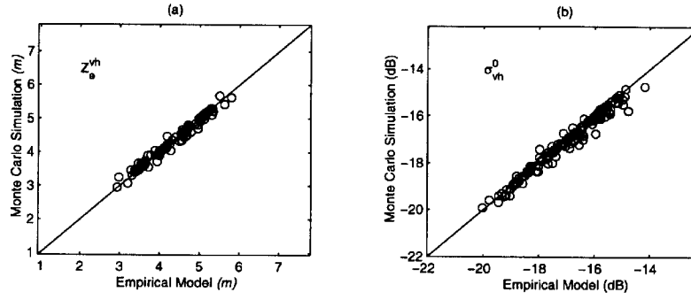
Figure 6.5: A comparison between the empirical model and the Monte Carlo coherent scattering model for a red pine stand at vh polarization configuration.
