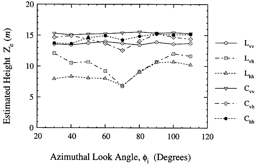
Figure 5.10: The estimated scattering phase center height of Stand 31 (red maple) over a tilted ground with tilt angle \theta_g = 10^\circ , at \theta_i = 25.4^\circ .
