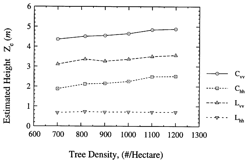
Figure 5.8: The estimated scattering phase center height of Stand 22 (red pine) as a function of tree density, simulated at \theta_i = 45^\circ .
