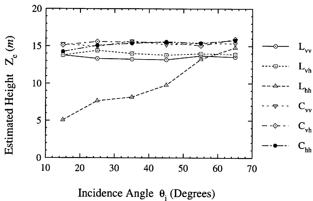
Figure 5.9: The estimated scattering phase center height of Stand 31 (red maple) as a function of incidence angle, with fully-polarimetric L- and C-and response.
