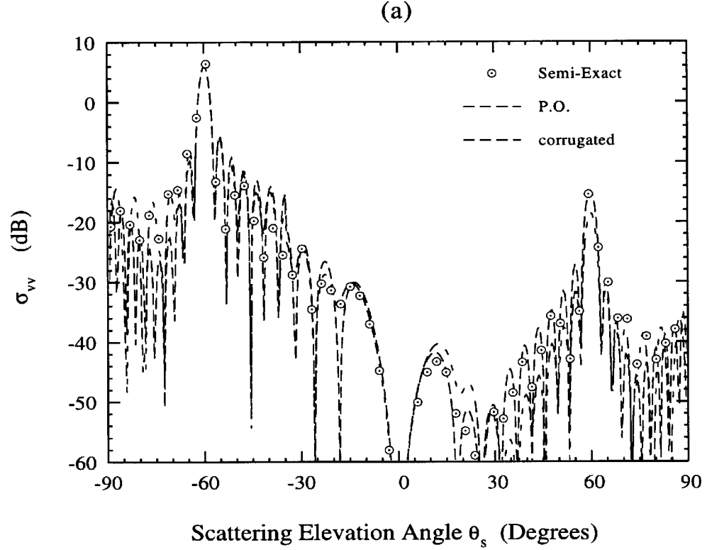
Figure 3.7: The normalized bistatic \sigma_{vv} (a) and \sigma_{hh} (b) as a function of the scattering elevation angle \theta_s in X-Z plane ( \theta_s > 0 when \phi_s = 0^\circ ; \theta_s < 0 when \phi_s = 180^\circ ). The backscattered and the specular directions are shown at \theta_s = 60^\circ and \theta_s = -60^\circ respectively. Other parameters are : \theta_i = 120^\circ , \phi_i = 180^\circ , \theta_g = \theta_c = 0^\circ , b = 10\lambda_0 , a_1 = 2\lambda_0 , a_2 = 1.8\lambda_0 .
