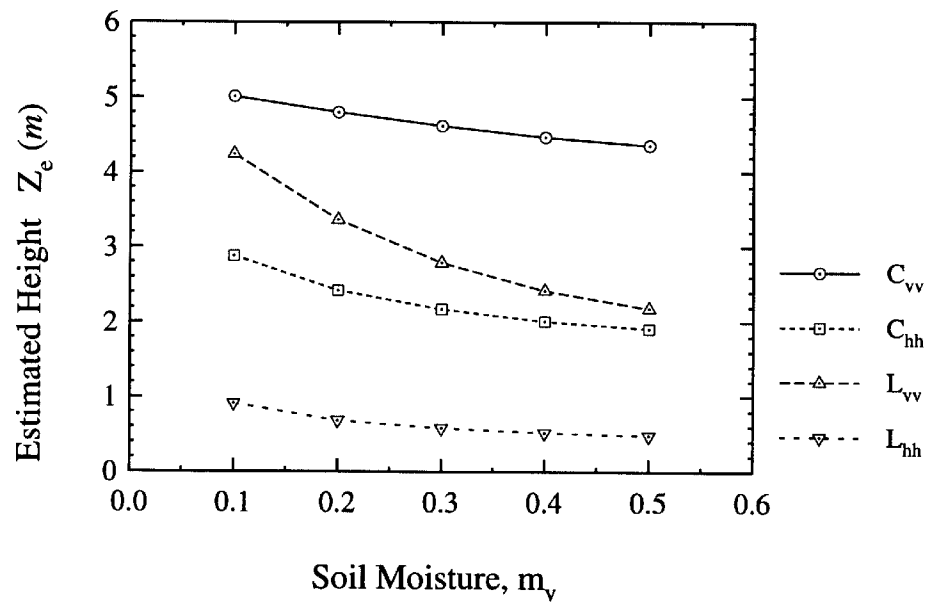
Figure 5.7: The estimated scattering phase center height of Stand 22 (red pine) as a function of soil moisture, simulated at \theta_i = 45^\circ .
