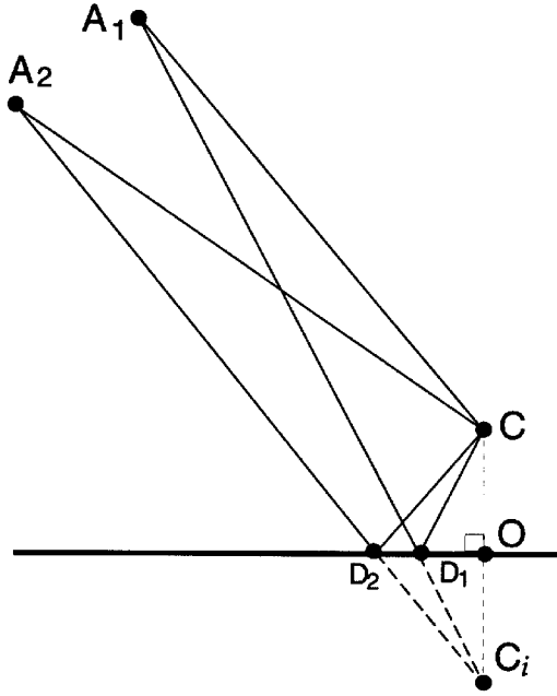
Figure 5.1: Multipath scattering mechanisms of an object (at C with projection at O and image at C_i ) above a ground plane observed by an interferometer with two antennas at A_1 and A_2 .
