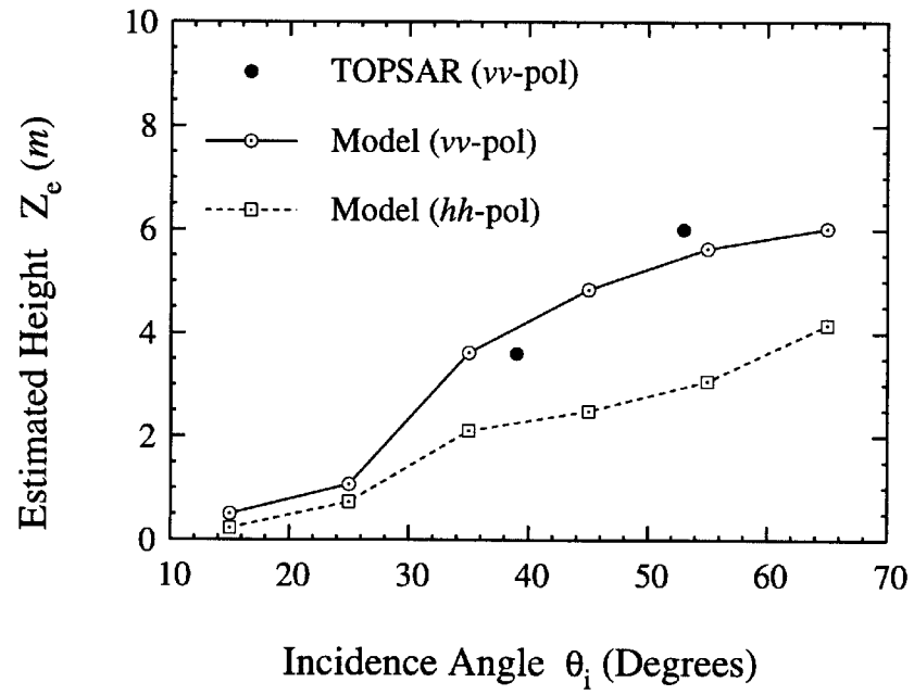
Figure 5.5: The estimated height of scattering phase center of Stand 22 (red pine), compared with the data extracted from two TOPSAR images ( \theta = 39^\circ and 53^\circ ) of the same stand.
