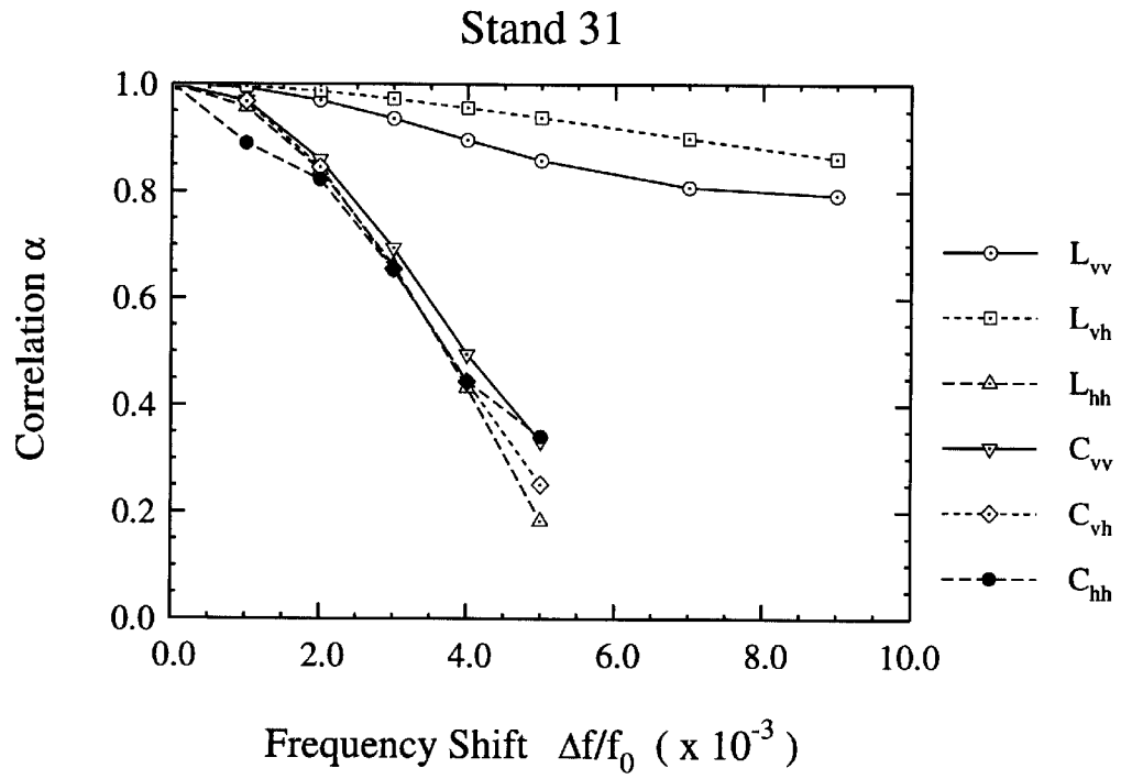
Figure 5.13: The correlation coefficient as a function of the frequency shift, simulated from Stand 31 (red maple).
