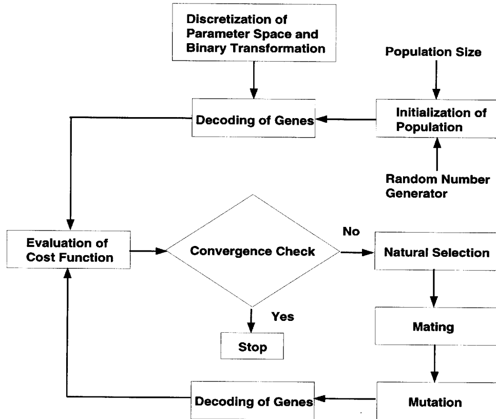
Figure 6.7: A flow chart of a genetic algorithm.
