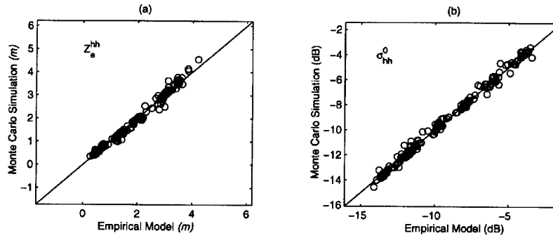
Figure 6.6: A comparison between the empirical model and the Monte Carlo coherent scattering model for a red pine stand at hh polarization configuration.
