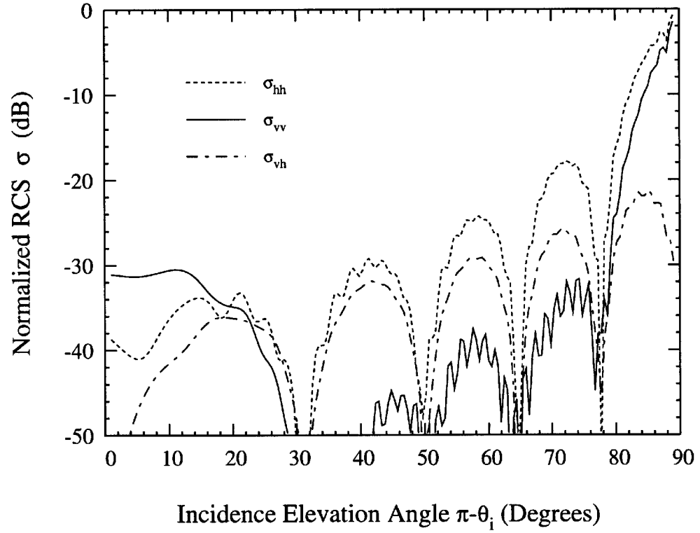
Figure 3.9: The normalized backscattering RCS as a function of the incidence angle \pi - \theta_i for a two-layer cylinder above a tilted ground plane. Other parameters are : \theta_g = 20^\circ , \phi_g = 90^\circ , \theta_c = 0^\circ , \phi_i = 180^\circ , \phi_s = 0^\circ , \theta_s = \pi - \theta_i , b = 20\lambda_0 , a_1 = 2\lambda_0 , a_2 = 1.8\lambda_0 .
