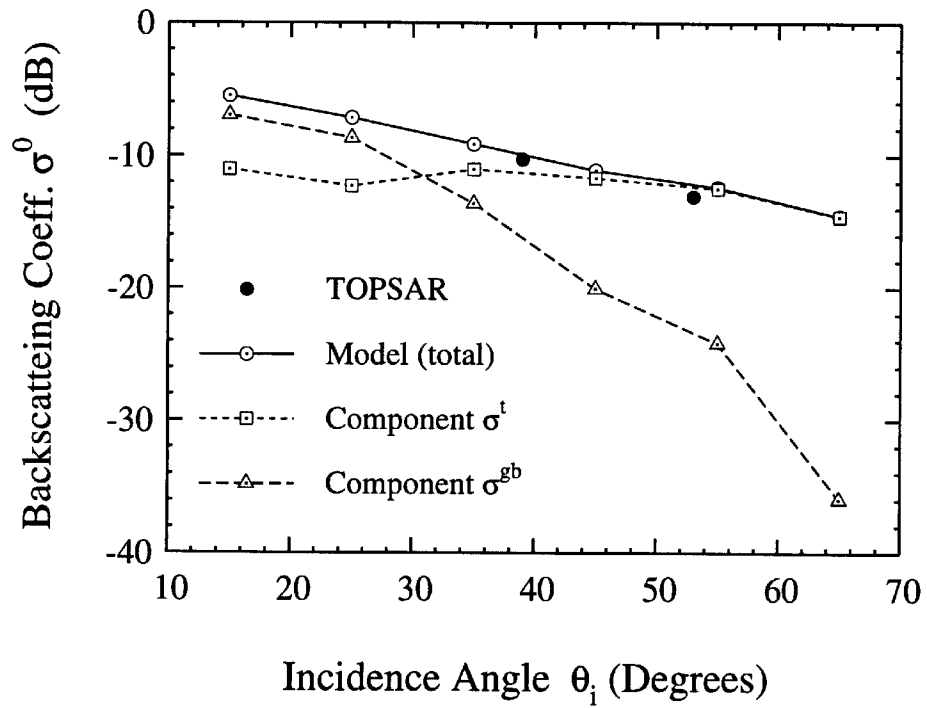
Figure 5.6: The simulated backscattering coefficient of Stand 22 (red pine), compared with the measured \sigma_{vv}^0 extracted from two TOPSAR images of the same stand.
