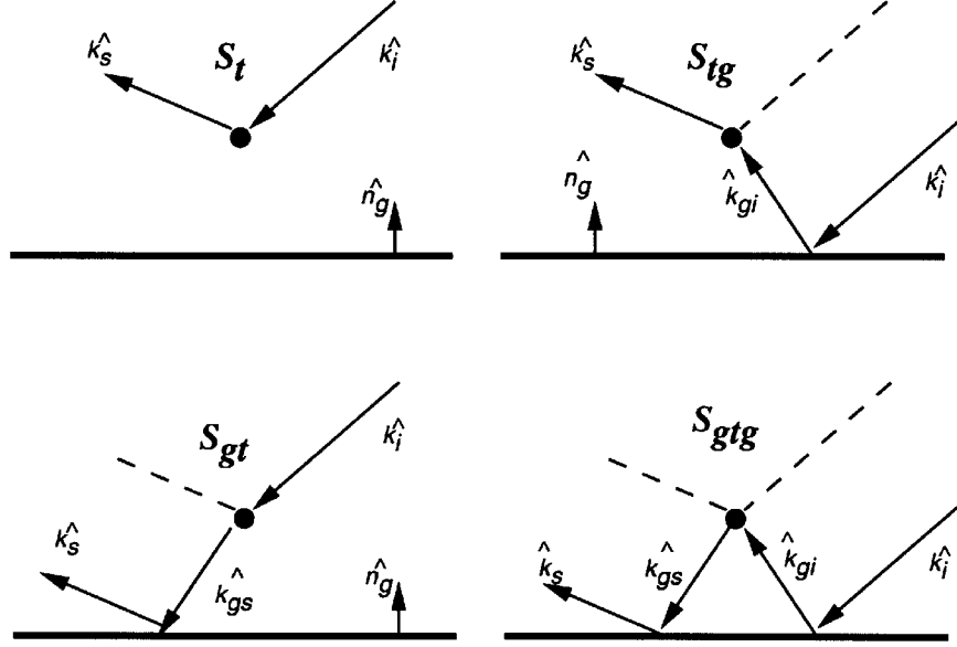
Figure 3.2: The first-order scattering components for scattering from an object above a ground plane.
