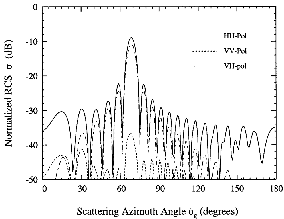
Figure 3.10: The normalized backscattering RCS as a function of the ground azimuth angle \phi_g . Other parameters are : \theta_g = 20^\circ, \theta_c = 0^\circ, \theta_i = 135^\circ, \phi_i = 180^\circ, \theta_s = 45^\circ, \phi_s = 0^\circ, b = 20\lambda_0, a_1 = 2\lambda_0, a_2 = 1.8\lambda_0 .
