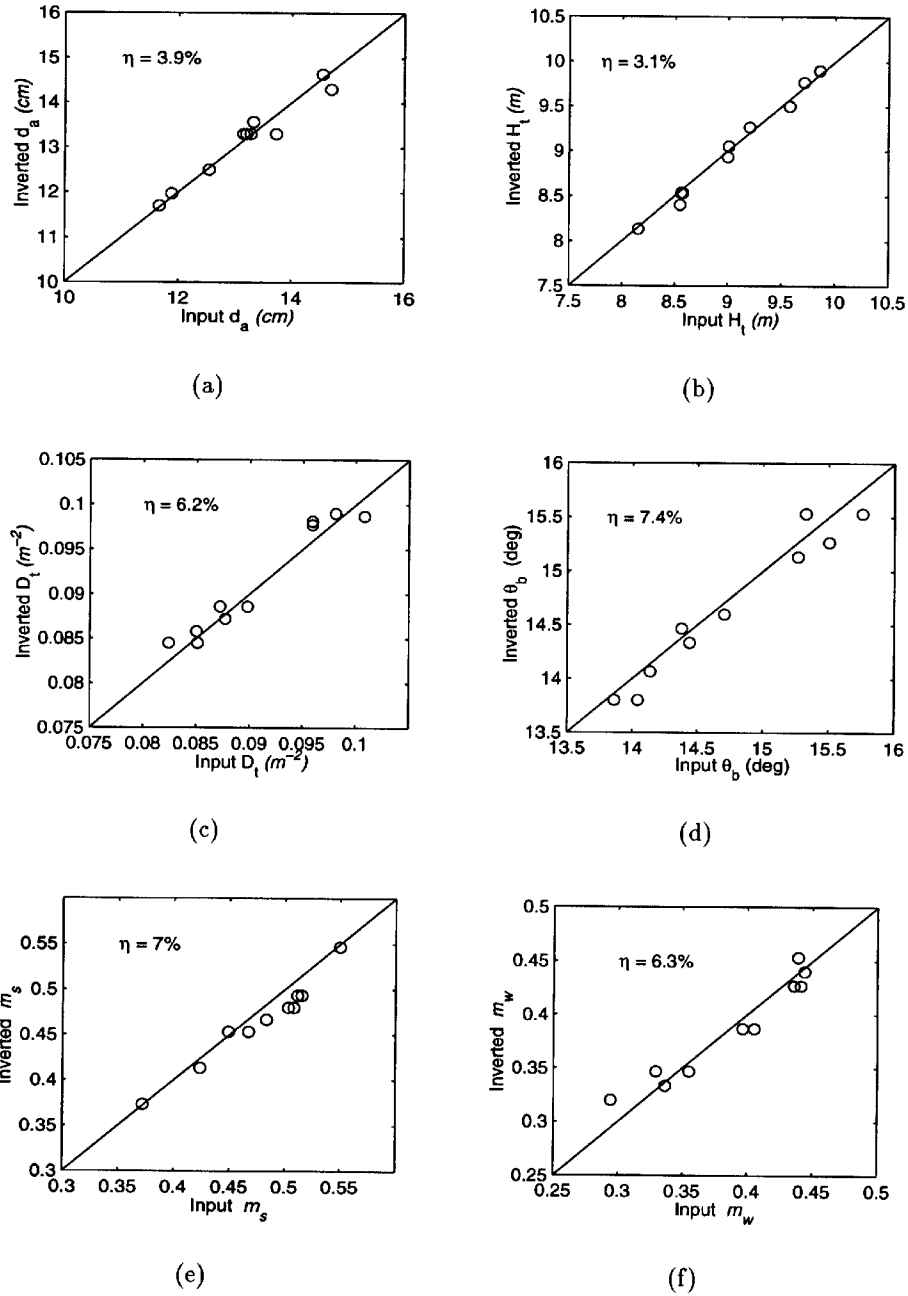
Figure 6.8: Comparison of the input parameters ( \mathbf{x} ) and the output of the inversion algorithm ( \mathbf{x}' ) using the synthetic data obtained from the Monte Carlo simulation, for (a) trunk diameter d_a , (b) tree height H_t , (c) tree density D_t , (d) branching angle \theta_b , (e) soil moisture m_s , and (f) vegetation moisture m_w . Here \eta is a measure of the average error in the inversion process defined by equation(6.15).
