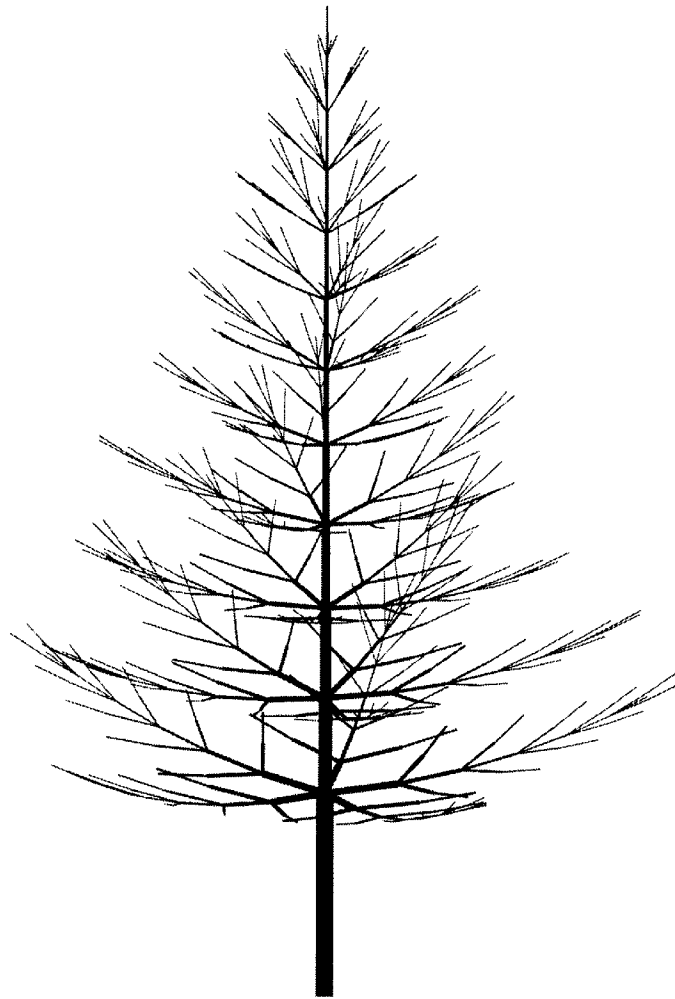
Figure 2.4: A fractal tree structure of coniferous type.
