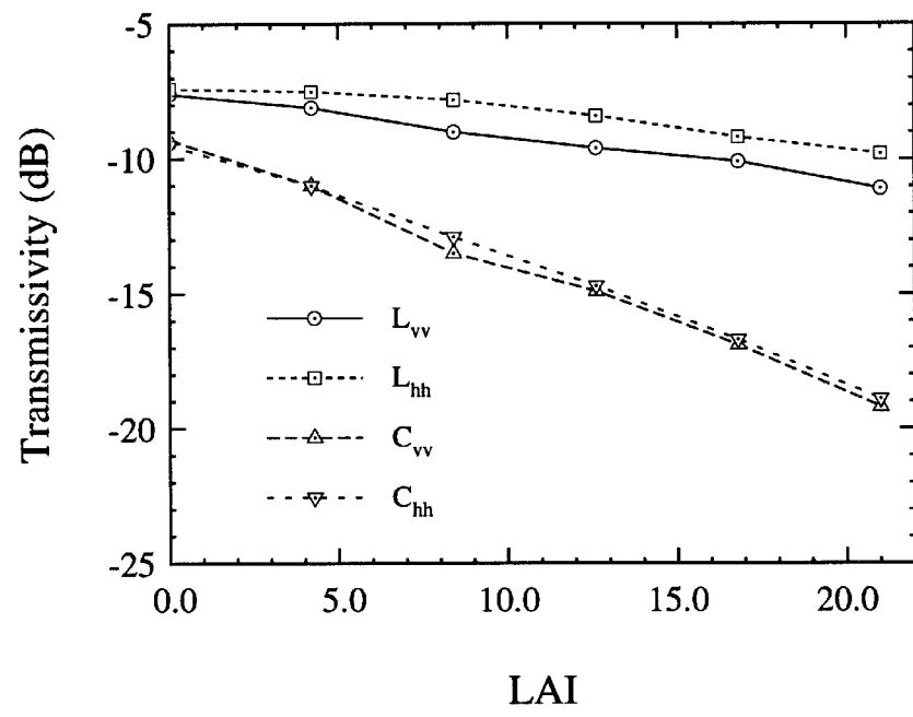
Figure 4.11: One-way transmissivity as a function of leaf area index (LAI).
