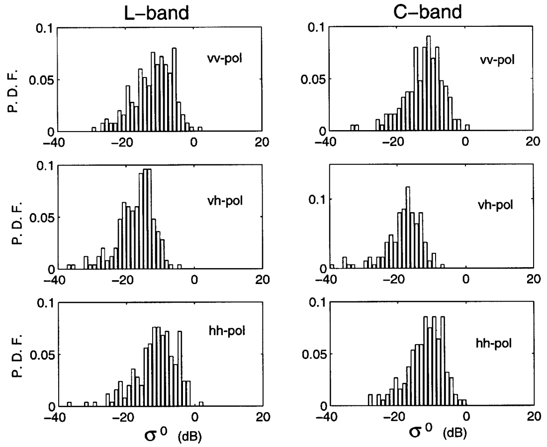
Figure 4.10: Histogram of the backscattering coefficients for Stand 31 at \theta_i = 43.6^\circ .
