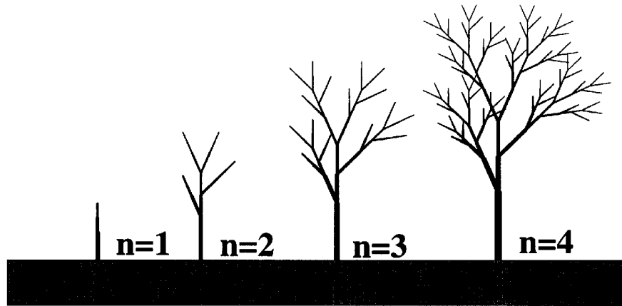
Figure 2.1: An example of the growing process of a fractal tree.
