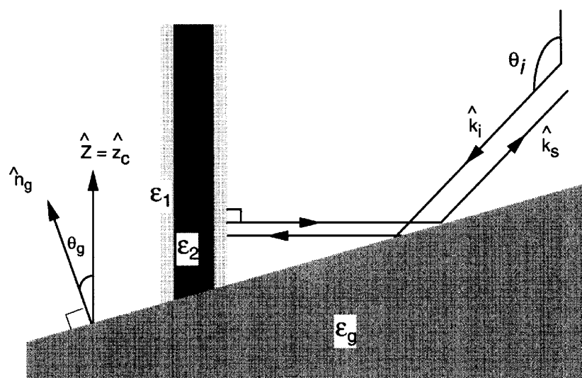
Figure 3.12: The geometry of the scattering configurations for a cylinder over a tilted ground where a strong backscatter can be observed.
