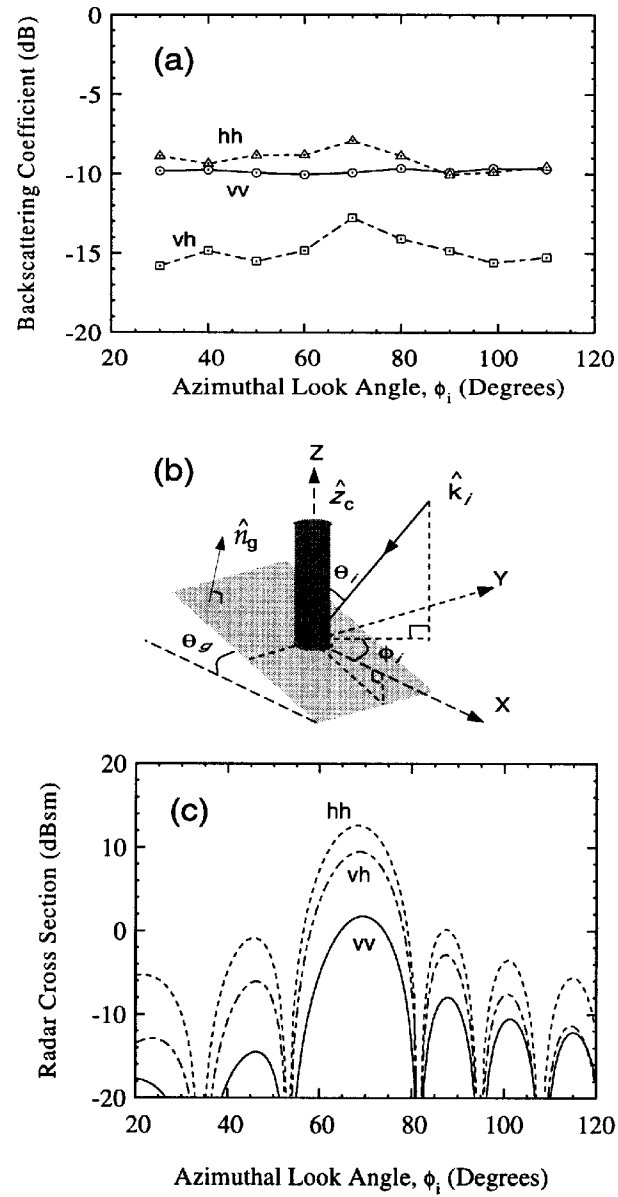
Figure 4.14: The effect of the ground tilt angle on radar backscatter: (a) backscattering coefficients for Stand 31 over a tilted ground with \theta_g = 10^\circ simulated at L-band with incidence angle \theta_i = 25.4^\circ , (b) a vertical cylinder on a tilted dielectric plane and the associated coordinates, (c) RCS simulation for (b).
