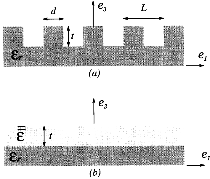
Figure 3.4: A corrugated layer (a) and its equivalent anisotropic layer (b).
