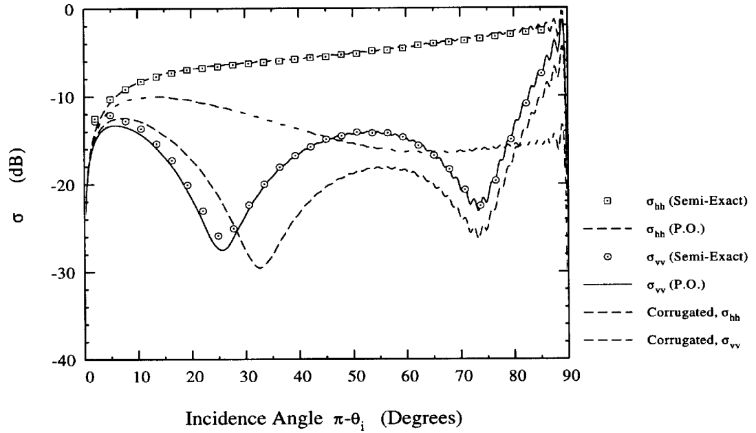
Figure 3.6: The normalized backscattering RCS as a function of the incidence angle \theta = \pi - \theta_i for a two-layer cylinder with and without the corrugation. Other parameters are : b = 20\lambda_0, a_1 = 2\lambda_0, a_2 = 1.8\lambda, t = 0.1\lambda_0, d/L = 0.7, \phi_i = 180^\circ, \phi_s = 0^\circ, \theta_g = \theta_c = 0^\circ .
