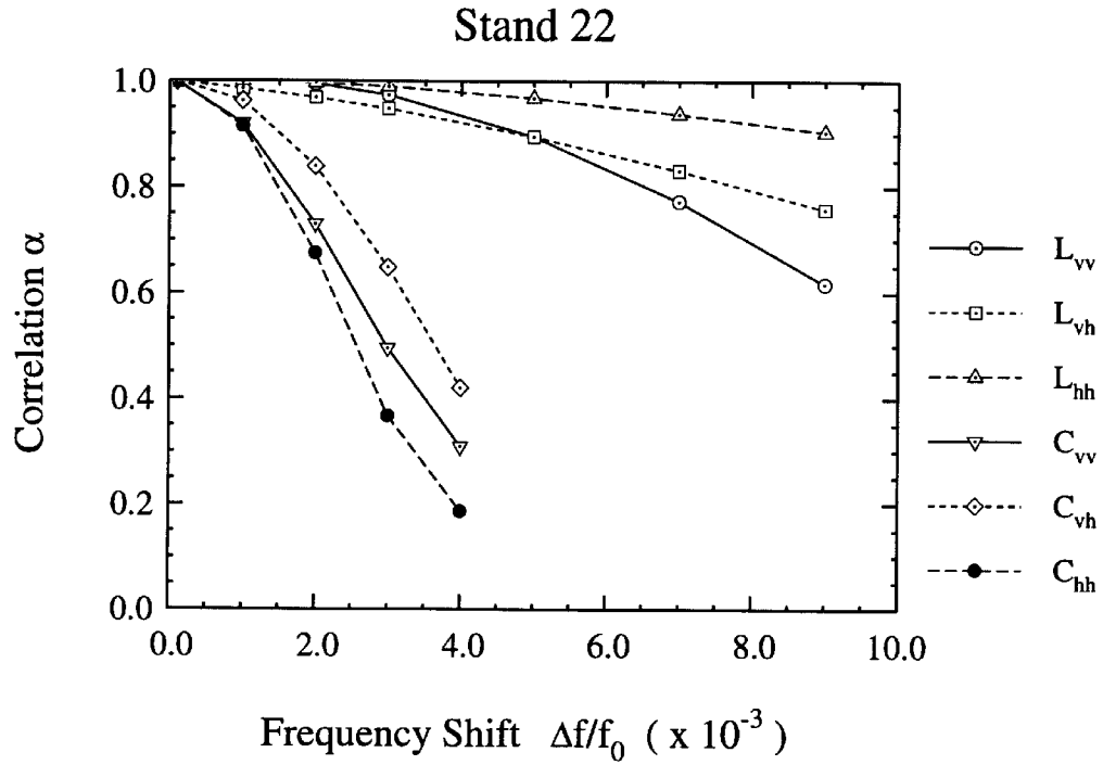
Figure 5.12: The correlation coefficient as a function of the frequency shift, simulated from Stand 22 (red pine).
