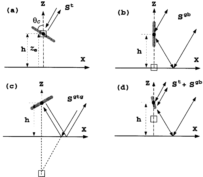
Figure 5.3: Four configurations for a cylinder above a ground plane with orientation angles: (a) \theta_c = 60^\circ, \phi_c = 180^\circ , (b) \theta_c = 0^\circ, \phi_c = 0^\circ , (c) \theta_c = 60^\circ, \phi_c = 0^\circ , (d) \theta_c = 45^\circ, \phi_c = 150^\circ , and their principal scattering mechanisms respectively. The center of the scatterer is denoted by ( \bullet ) and equivalent scattering phase center by ( \square ).
