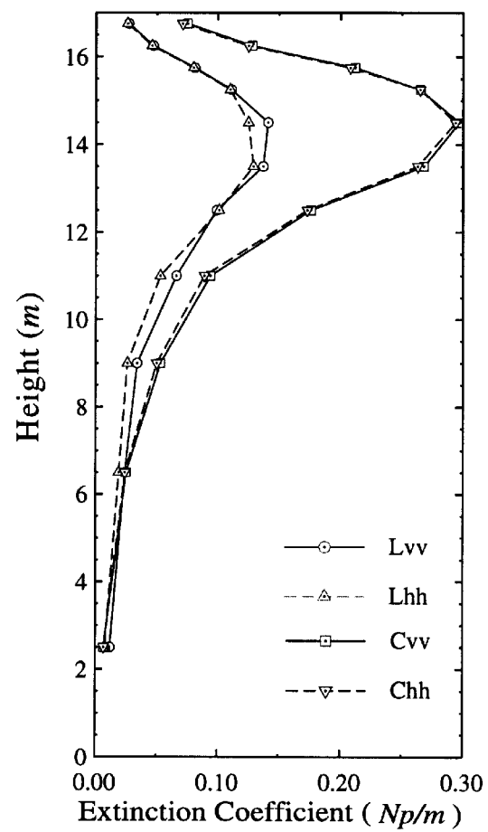
Figure 4.4: The extinction profile calculated for Stand 31.
