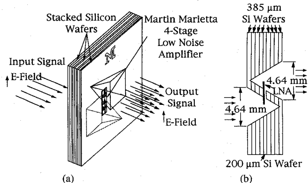
Fig. 1. Quasi-optical amplifier consisting of Martin Marietta Laboratories' low noise amplifier between two back-to-back pyramidal horns. A plane wave input signal is amplified and repeated on the opposite side with the same polarization. (a) Isogonal view. (b) Side view.
