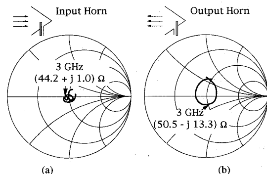
Fig. 2. Input impedance of a scaled monopole probe measured from 2.75 GHz to 3.25 GHz (equivalent to 86.5 GHz to 102 GHz) inside the (a) input pyramidal horn and (b) output pyramidal horn.
