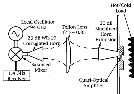
Fig. 6. Noise figure experiment using an LO frequency of 94 GHz and an IF of 1.4 GHz.
