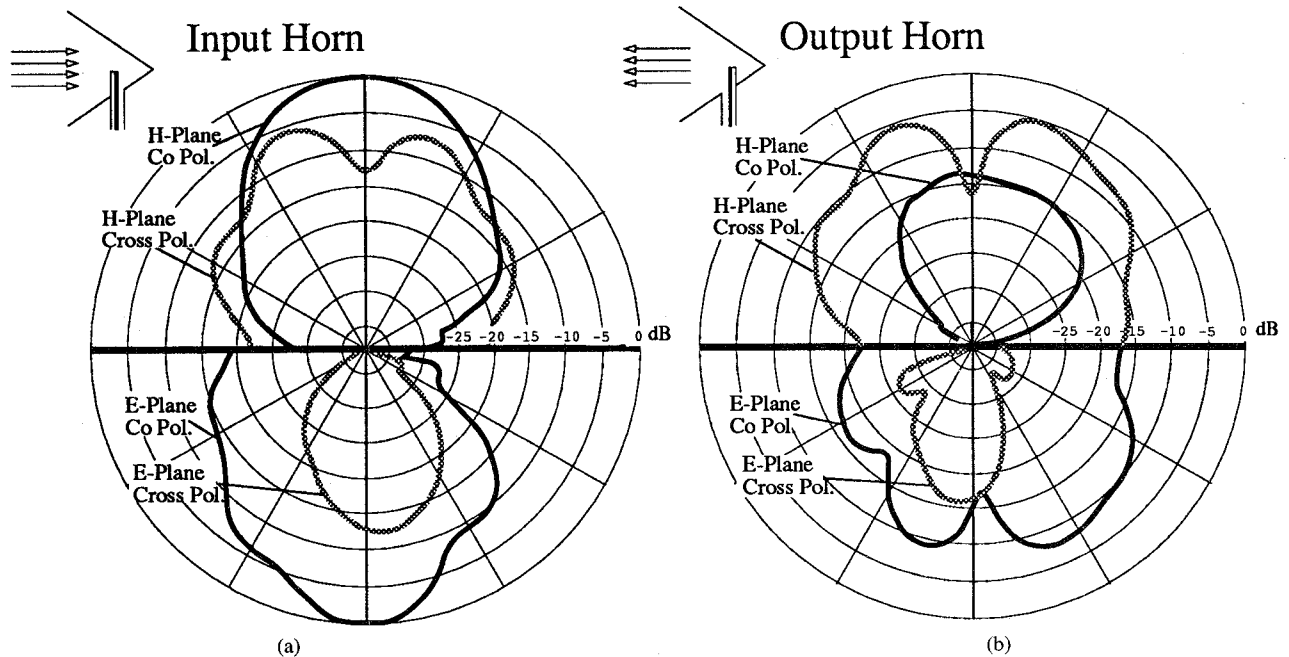
Fig. 4. Quasi-optical amplifier 3 GHz microwave model (equivalent to 94 GHz) antenna patterns. (a) Antenna patterns with monopole facing the interior of the horn. (b) Antenna patterns with monopole facing the exterior of the horn.
