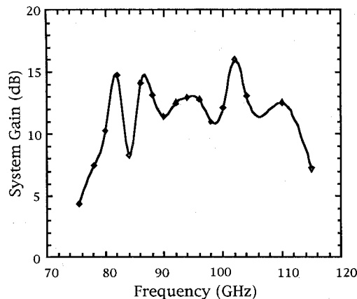
Fig. 5. Quasi-optical amplifier system gain versus frequency. The system gain includes loss due to input and output horn aperture efficiency (see text for more detail).
