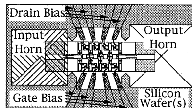
Fig. 3. Martin Marietta Laboratories' low noise amplifier (LNA) chip placed in a cavity between two horn openings. The LNA chip dimensions are 4.25 \text{ mm} by 1.25 \text{ mm} .
