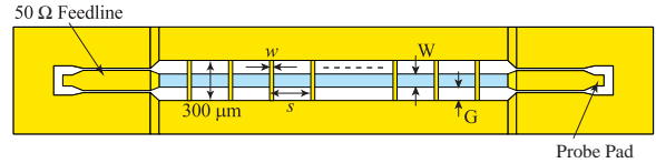
Fig. 1. Layout of a portion of a DMTL constructed of a CPW line with center conductor width W and total CPW width W+2G , and MEMS bridges with width w and spacing s .
