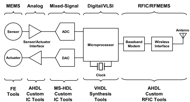
Fig. 1: The anatomy of a generalized wireless integrated microsystem. Key technologies and associated development tools are shown.
