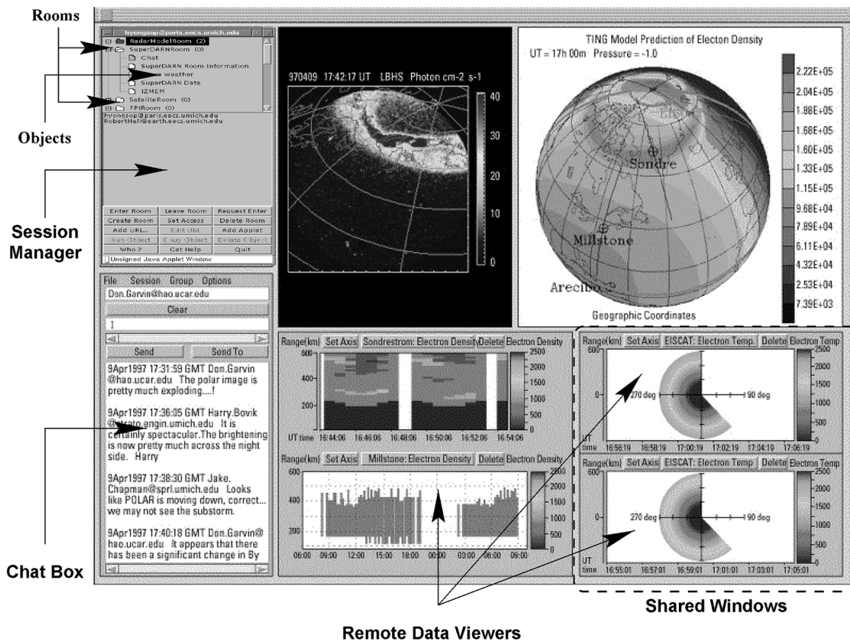
Fig. 2. UARC Collaborative Applications. Session Manager allows users to organize their collaborative and private work. The chat box allows users to exchange textual messages. A whiteboard (not shown) allows users to annotate images and brainstorm about their work. The remote data viewers receive atmospheric data from various instruments at remote locations and graphically display the data according to data types and user settings. Users may export CBE-compatible windows to each other, allowing synchronized views of data.
