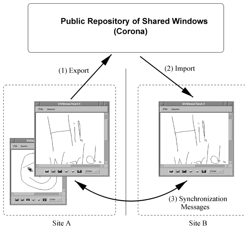
Fig. 4. Selective window sharing. A shared window is first exported to the public repository and then imported. An imported window is replicated and functionally equivalent to the exported window. The shared window displays a synchronized view of shared application data.
