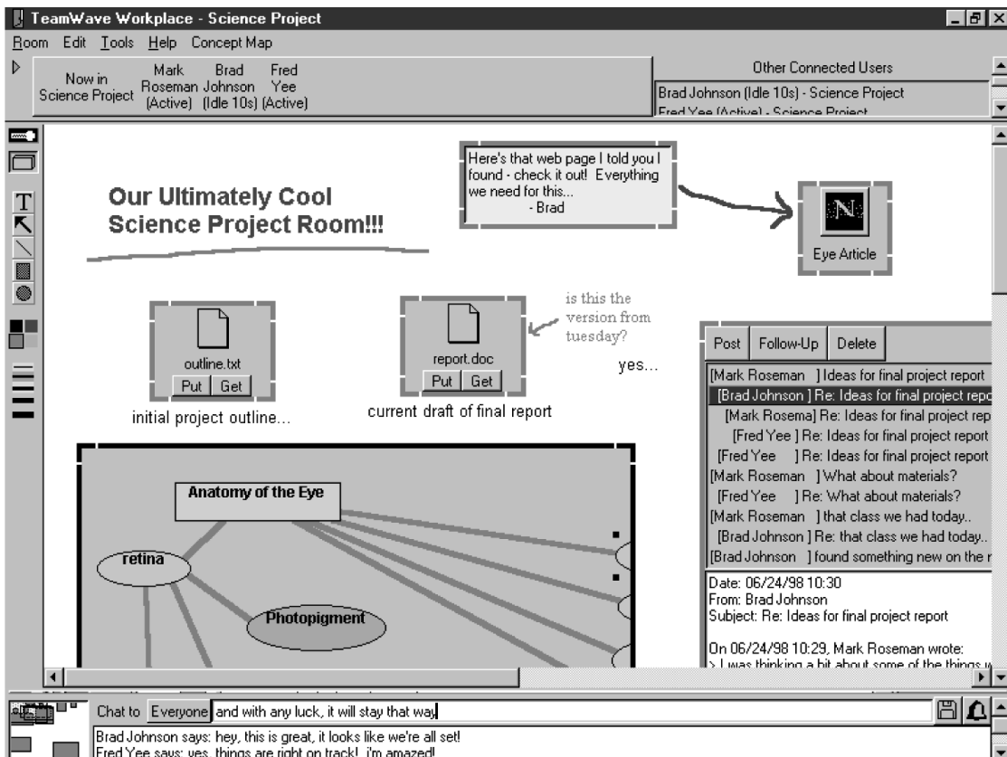
Fig. 5. A shared window manager in TeamWave.
