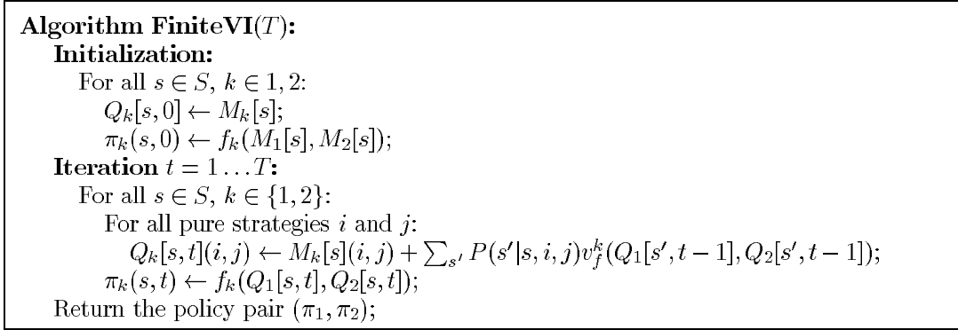
Figure 1: Algorithm FiniteVI for computing Nash equilibria in finite-horizon undiscounted stochastic games. Recall that f is an arbitrary Nash selection function, f_k extracts the mixed strategy selected by f for player k , and v_f^k extracts the value of the selected Nash to player k .
