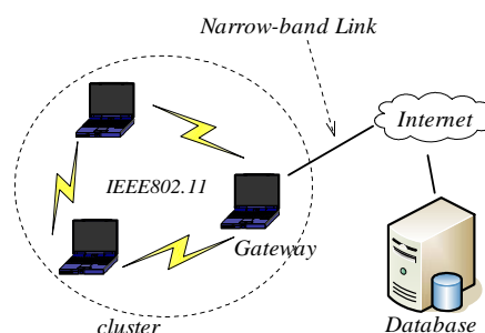
Figure 1.1: Network model
