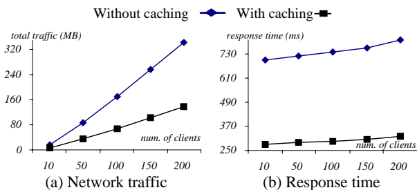
Figure 6.1: Effectiveness of caching
