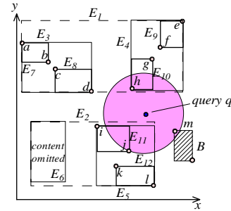
Figure 5.2: Exemplary k NN query
