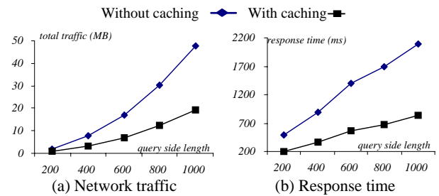
Figure 6.2: Impact of side length of range queries
