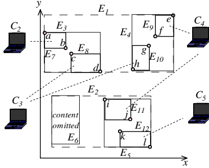
Figure 4.3: Cached regions
