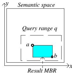
Figure 4.1: Cacheable region of a range query
