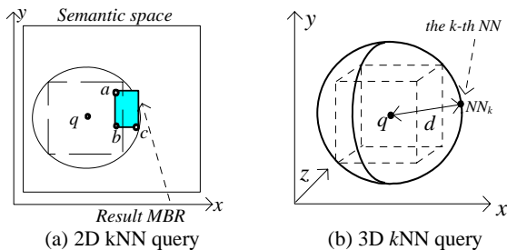
Figure 4.2: Cacheable region of a k NN query
