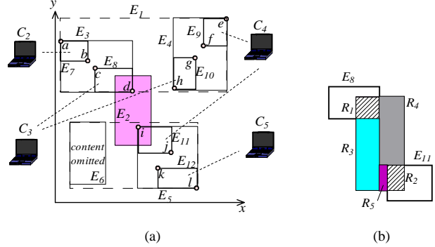
Figure 5.1: Range query and its remainder queries
