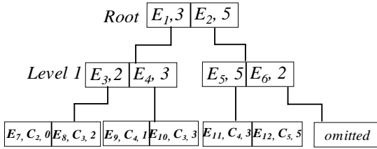
Figure 4.4: Corresponding CR-tree
