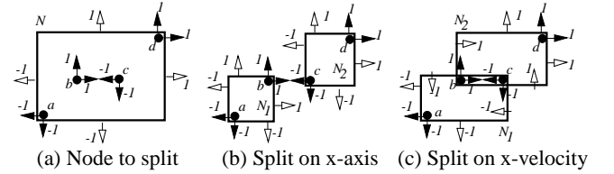
Figure 2.3: The split algorithm of the TPR*-tree
