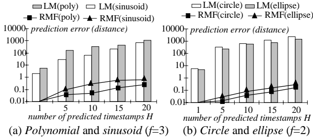
Figure 6.2: Prediction error for regular movements
