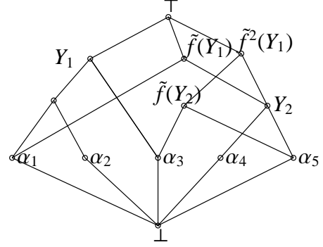
Fig. 2. Lattice (\chi, \leq) . We have \tilde{f}(Y_2) = \{\alpha_3, \alpha_5\} , \tilde{f}(Y_1) = \{\alpha_1, \alpha_4, \alpha_5\} , and \tilde{f}^2(Y_1) = \{\alpha_3, \alpha_4, \alpha_5\} .
