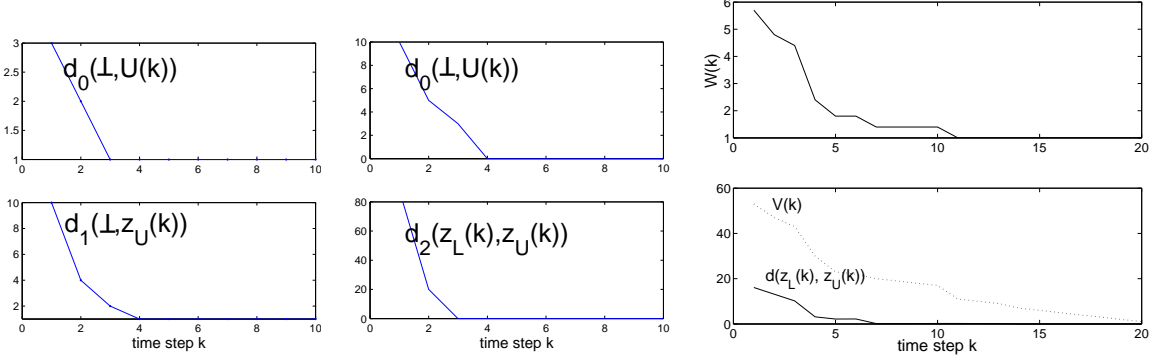
Fig. 3. Left: Estimator performance for Example 1. Middle: Estimator performance for Example 2. Right: Estimator performance for Example 3 with N = 10 robots per team. In the plots, d_0(\perp, U(k)) = \|\perp, U(k)\| .
