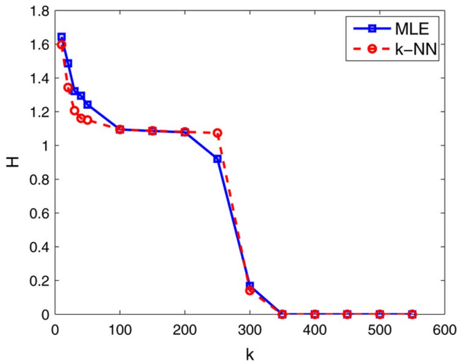
Fig. 12. The entropy of the local dimension estimates changes as a function of neighborhood size k .
