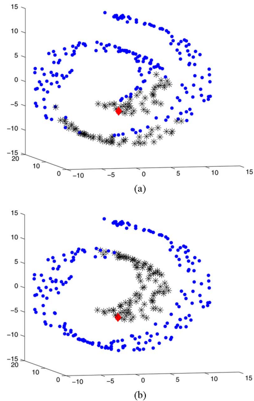
Fig. 1. Neighborhoods (*) of the sample in question (◇) defined by (a) Euclidean distance and (b) geodesic distance. (a) Spherical neighborhood and (b) adaptive neighborhood.
