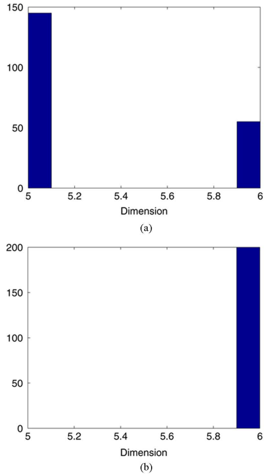
Fig. 5. Developing a debiased global dimension estimate by averaging over the 50% of points with the greatest depth on the manifold. (a) Biased results and (b) debiased results.
