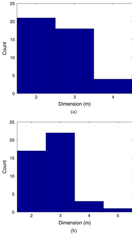
Fig. 8. Histogram of local dimension estimates for the statistical manifold defined by flow cytometry results of 43 patients with chronic lymphocytic leukemia or mantle cell lymphoma. (a) Local k -NN dimension estimates and (b) local MLE dimension estimates.
