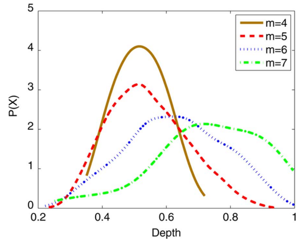
Fig. 4. PDFs of data depth based on estimated intrinsic dimension. Points with less depth estimate at a lower dimension, contributing to the overall negative bias.
