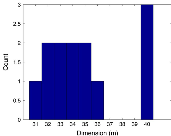
Fig. 3. Issues arise with neighborhood smoothing when estimating very large dimensions due to the variance of such estimates. In this example, smoothing would assign a dimension estimate of 40, although the more appropriate estimate would be 33 or 34.
