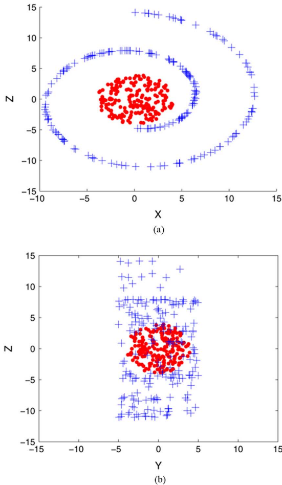
Fig. 14. Clustering based on local intrinsic dimensionality is useful for problems such as this, in which three-dimensional hypersphere ( \bullet ) is placed “inside” the two-dimensional “swiss roll” ( + ). Side and front angles of set shown. (a) Side and (b) front.
