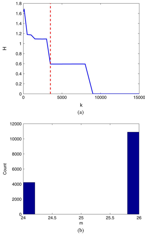
Fig. 15. Plotting the entropy of the dimension estimates suggests a neighborhood size of k = 3500 , denoted by the dotted line, which yields two significant clusters in the dimension estimates. (a) Entropy versus k and (b) histogram of dimension estimates.
