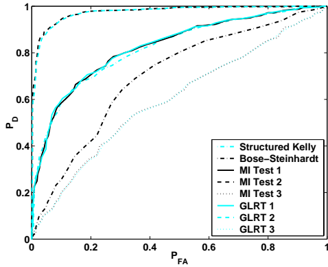
Fig. 7. ROC curves for Case 2 with SNR = 10dB ( m_A = 50, m_B = 50, n = 61 ).
