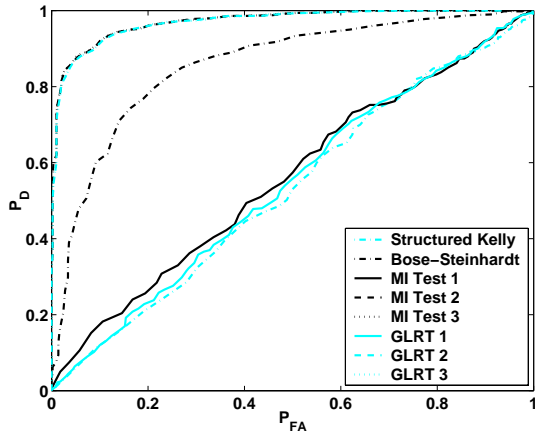
Fig. 4. ROC curves for Case 3 with SNR = 10dB ( m_A = 40, m_B = 60, n = 61 ).
