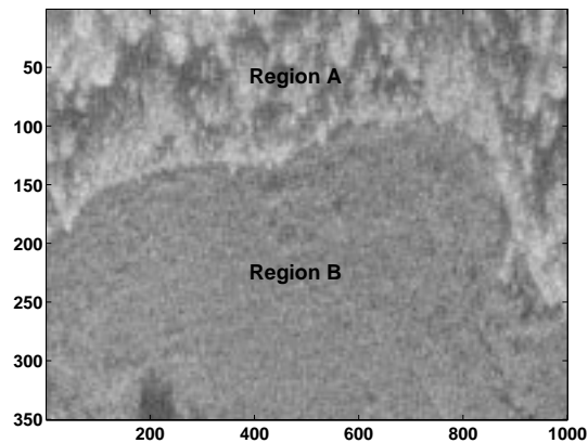
Fig. 1. SAR clutter image with SLICY target in the boundary at column 305.
