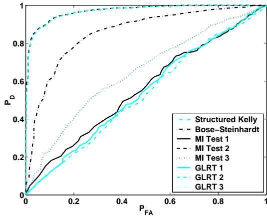
Fig. 3. ROC curves for Case 2 with SNR = 10dB ( m_A = 40, m_B = 60, n = 61 ).
