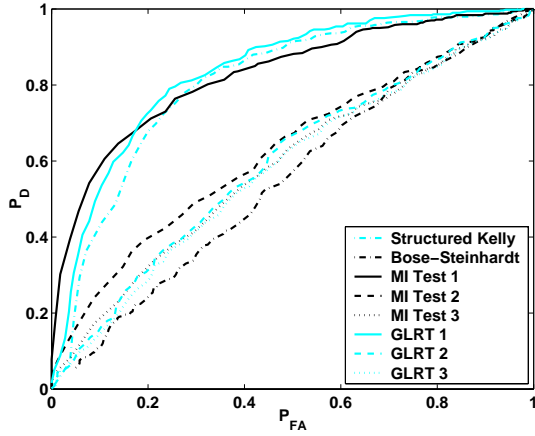
Fig. 2. ROC curves for Case 1 with SNR = 22dB ( m_A = 50, m_B = 50, n = 51 ).
