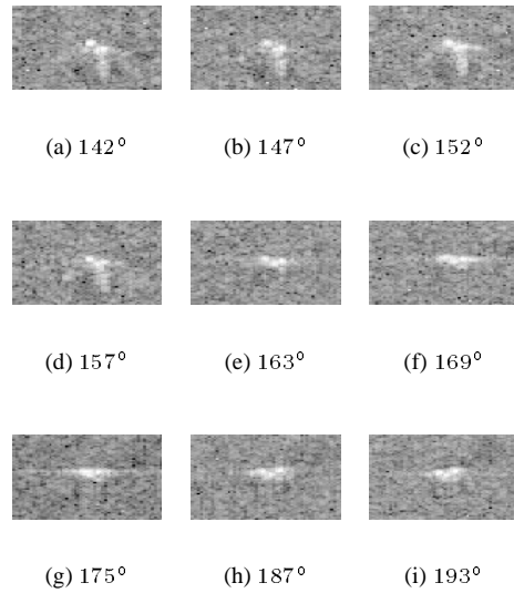
Fig. 9. SLICY canonical target images at elevation 39^\circ and different azimuth angles. Image in (e) is inserted in Fig. 1.
