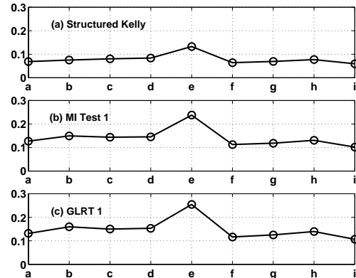
Fig. 11. Peak values obtained for 9 different target images.
