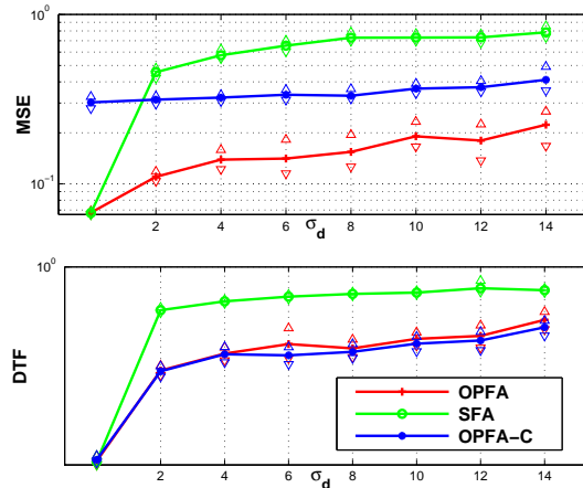
Fig. 6. MSE (top) and DTF (bottom) as a function of delay variance \sigma_d^2 for OPFA and Sparse Factor Analysis (SFA). These curves are plotted with 95% confidence intervals. For \sigma_d^2 > 0 , OPFA outperforms SFA both in MSE and DTF, maintaining its advantage as \sigma_d increases. For large \sigma_d , OPFA-C outperforms the other two.
