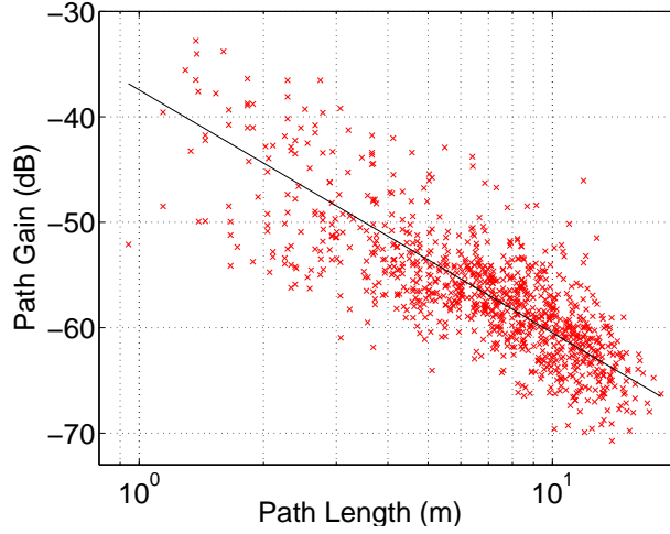
Fig. 5. Measured wideband path gain (x) as a function of path length. Linear fit (—) is with d_0 = 1\text{m} , n_p = 2.3 , and \sigma_{dB} = 3.92 .
