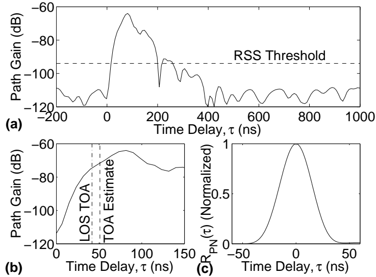
Fig. 4. (a) Measured PDP with TX at 1 and RX at 24 and threshold (- -) above which received power is integrated to calculate RSS. (b) Leading edge of same PDP showing LOS TOA = d_{1,24}/c (· · · ·) and estimated TOA (- - -). (c) Autocorrelation of PN signal R_{PN}(\tau) used in template-matching [23].
