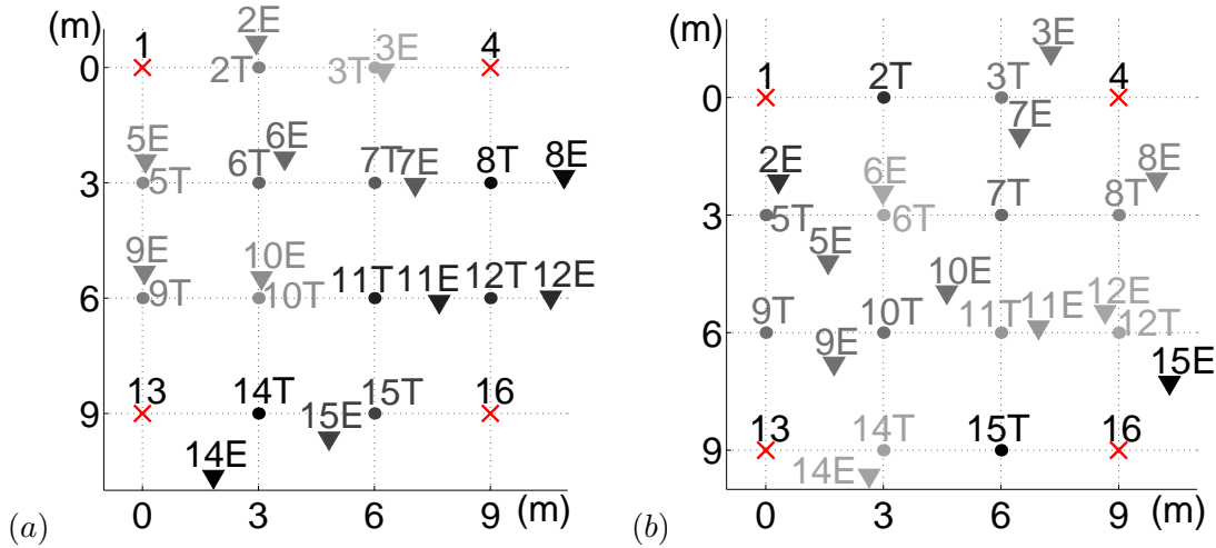
Fig. 11. True (●#T) and estimated (▼#E) location for the (a) parking lot and (b) residential home tests, using 4 reference devices (X#). Higher errors are indicated by darker text.
