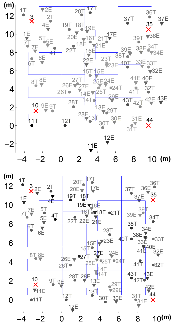
Fig. 7. True ( \bullet /#T) and estimated ( \blacktriangledown /#E) location using (a) RSS and (b) TOA data for measured network with 4 reference devices (X#). Higher errors are indicated by darker text.
