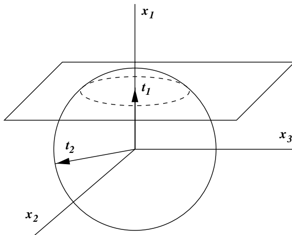
Figure 3.1: Sufficiency orbit is a circle in \mathbb{R}^3
