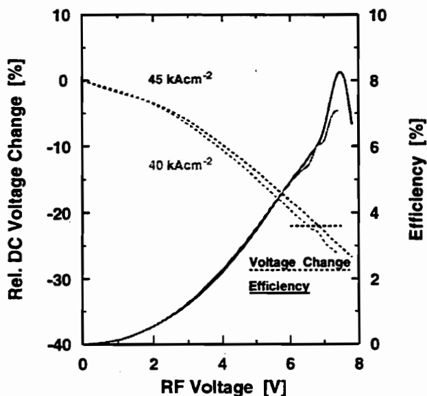
Figure 5: Predicted back bias effect and dc-to-RF conversion efficiency as a function of RF voltage amplitude for a GaAs TUNNETT diode in the fundamental mode at 107 GHz.
