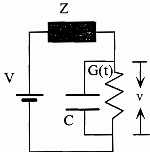
Fig.2. Equivalent circuit of the photoconductive antenna device.
