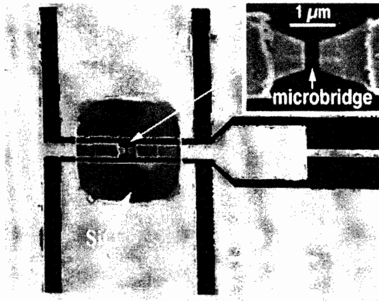
Broadband 1.5 - 2.5 THz HEB Mixer
