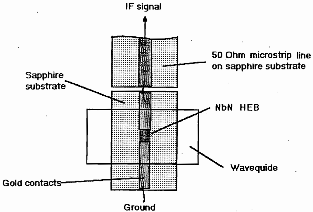
Fig.1 View of the mixer chip on the waveguide flange.
