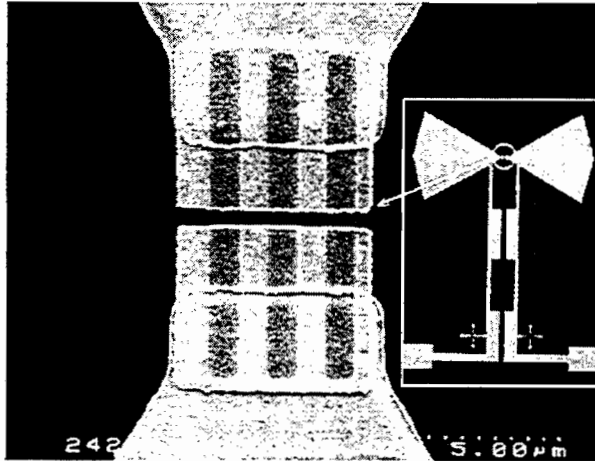
Figure 1: Microbridges integrated in the center of a dipole-antenna
