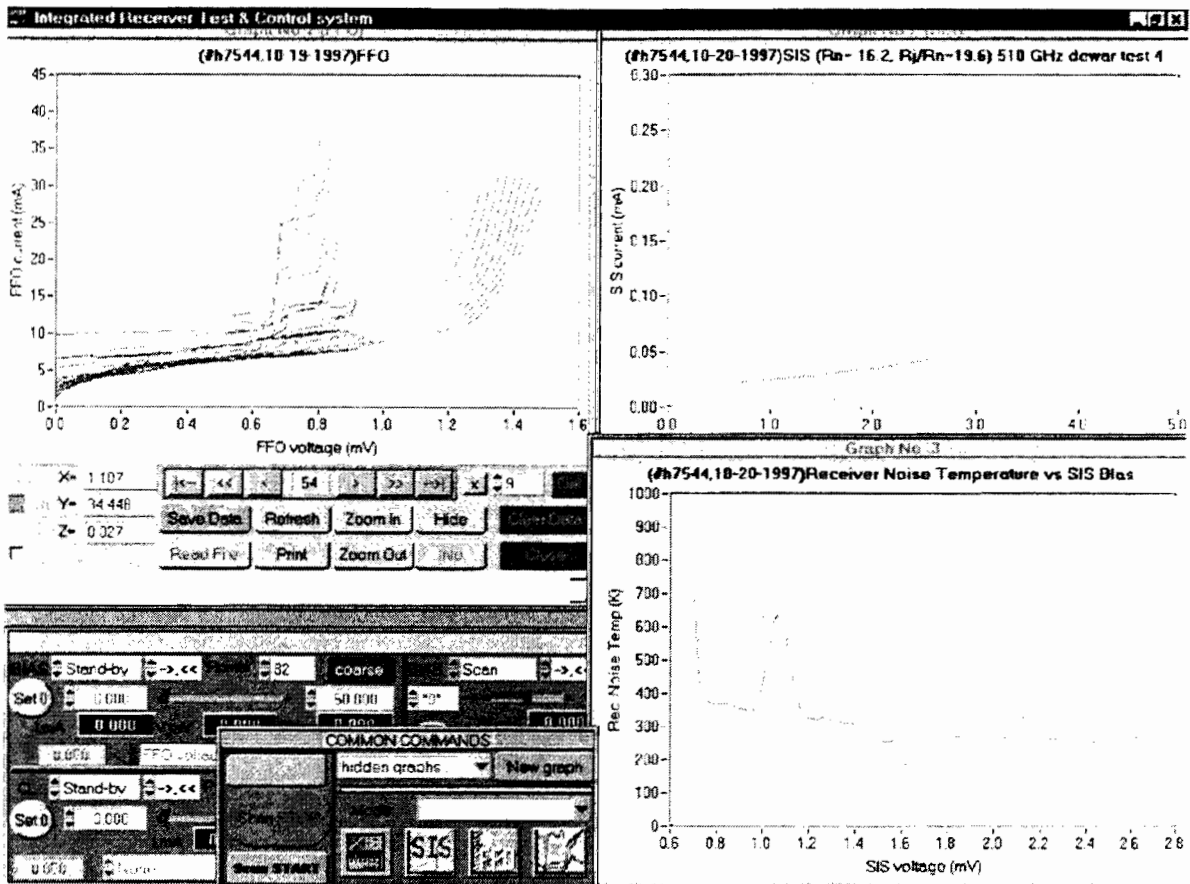
Fig. 7. Computer screen of "IRTECON" - Integrated Receiver Test & Control system: FFO IV-curves (top-left); un-pumped and pumped IV-curves of SIS mixer (top-right); receiver noise temperature vs. mixer bias voltage (bottom-right); receiver control panels (bottom-left).
