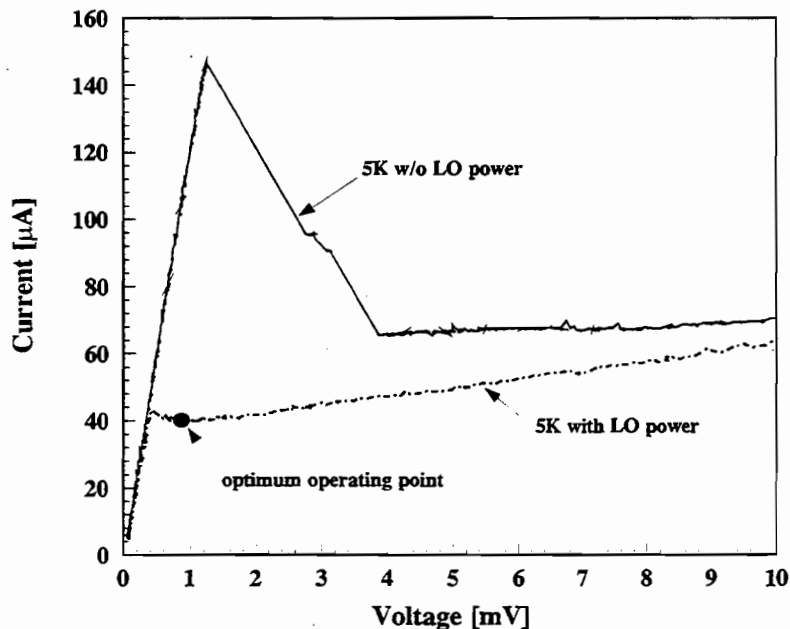
Figure 7: I-V curve for the device used in the 1.56 THz noise temperature measurement.
