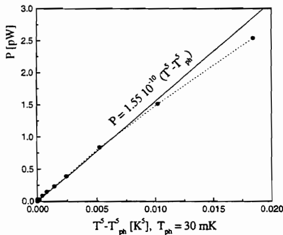
Fig. 5. Power dissipated in the absorber vs. (T^2 - T_{ph}^2) , where T is temperature of electrons deduced from measurements V(I_{bias}, T) , and T_{ph} = 30 mK is temperature of the lattice (measured temperature of the sample holder). Linear fit corresponds to the relation (2).
