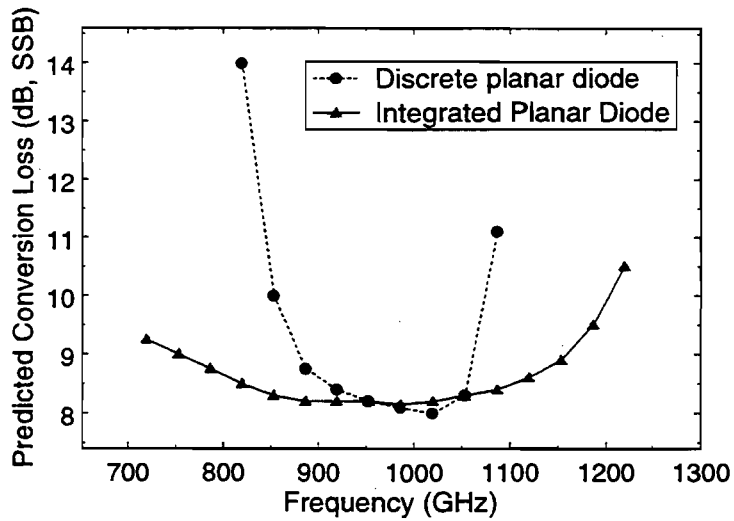
Figure 6: Simulated L_{conv} vs. frequency for integrated and discrete mixers
