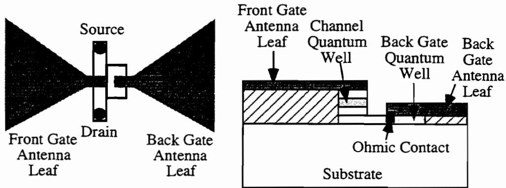
Figure 4: Top-down and cross-section views of a TACIT detector. Ohmic contacts electrically connect the back gate antenna leaf with the back gate quantum well, and the source and drain contacts to the channel quantum well. The active region of the device is defined by making the material outside, indicated by diagonal lines, electrically insulating.
