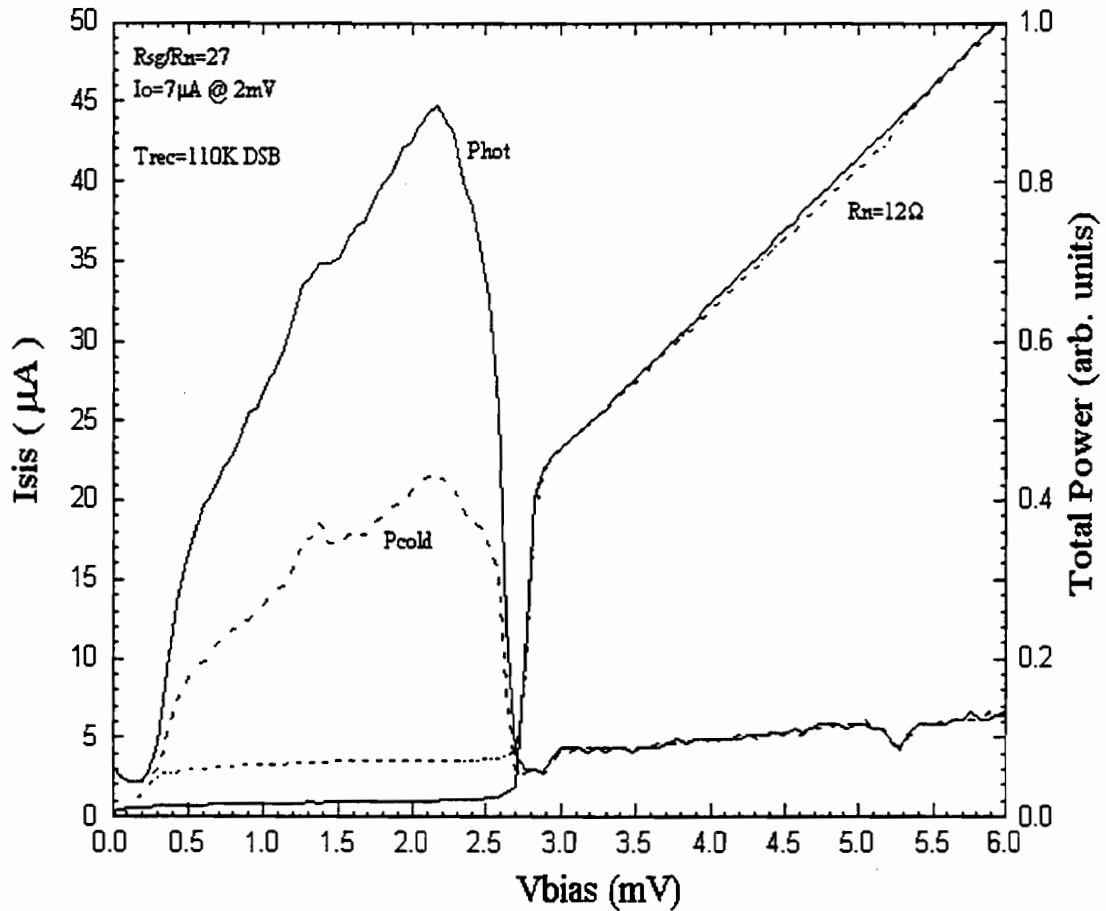
Fig. 3 Heterodyne response of a Nb/Al-O x /Nb junction with NbTiN groundplane at 639 GHz.
