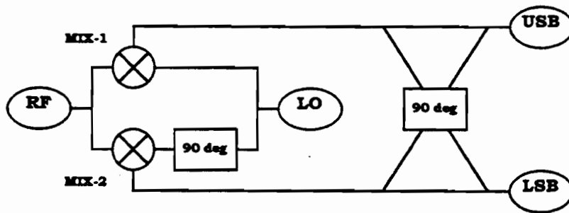
Fig.1 Principle of the conventional microwave image-rejection mixer circuit.
