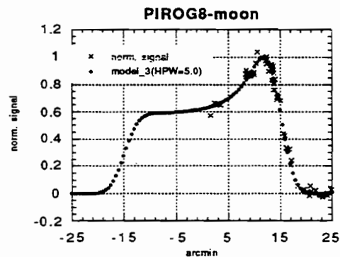
Fig. 10: Experimental and theoretical data of normalized brightness temperature of the moon versus moon position. Date agrees very well with observations.
