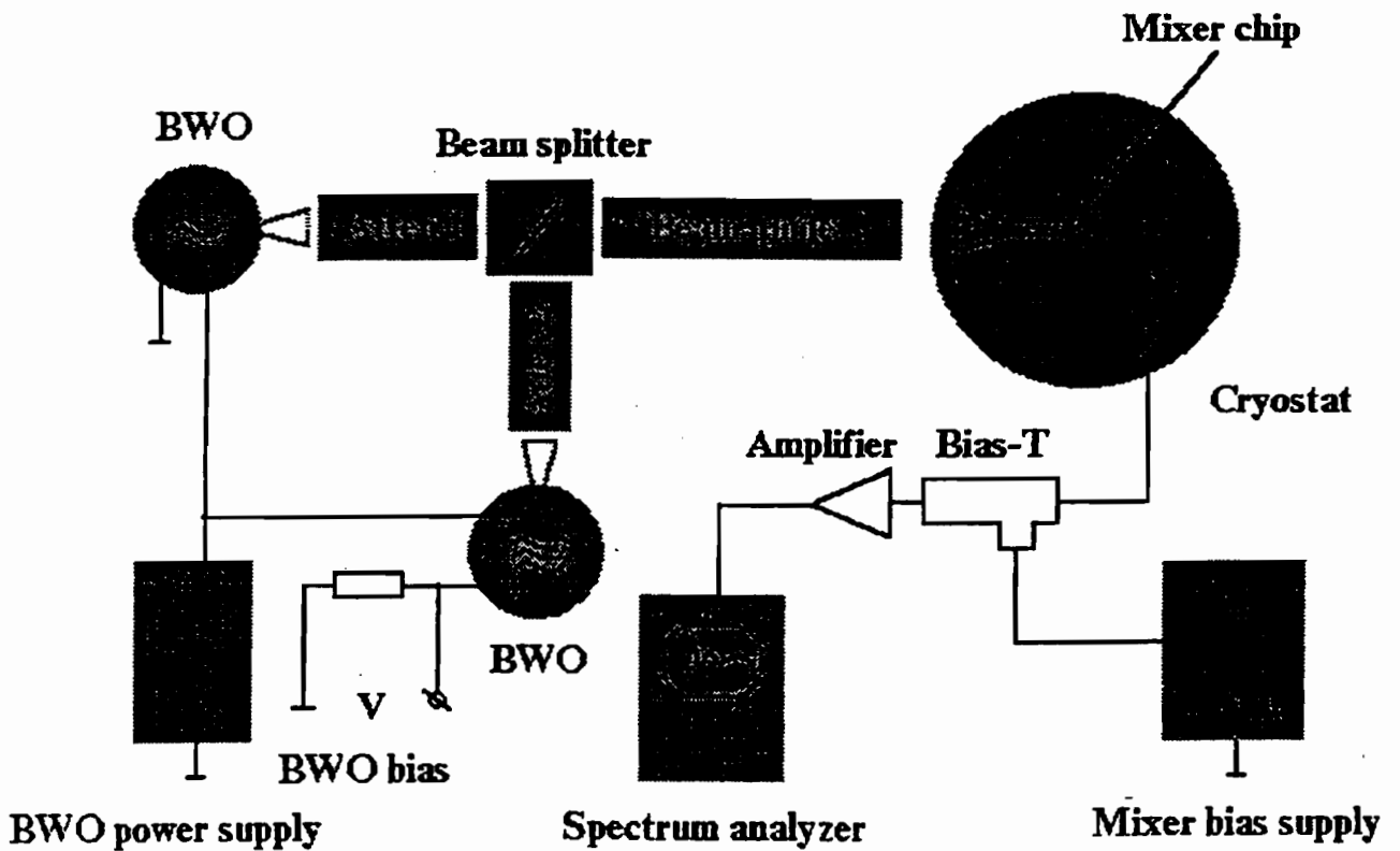
Fig.2 Set-up for bandwidth measurements.
