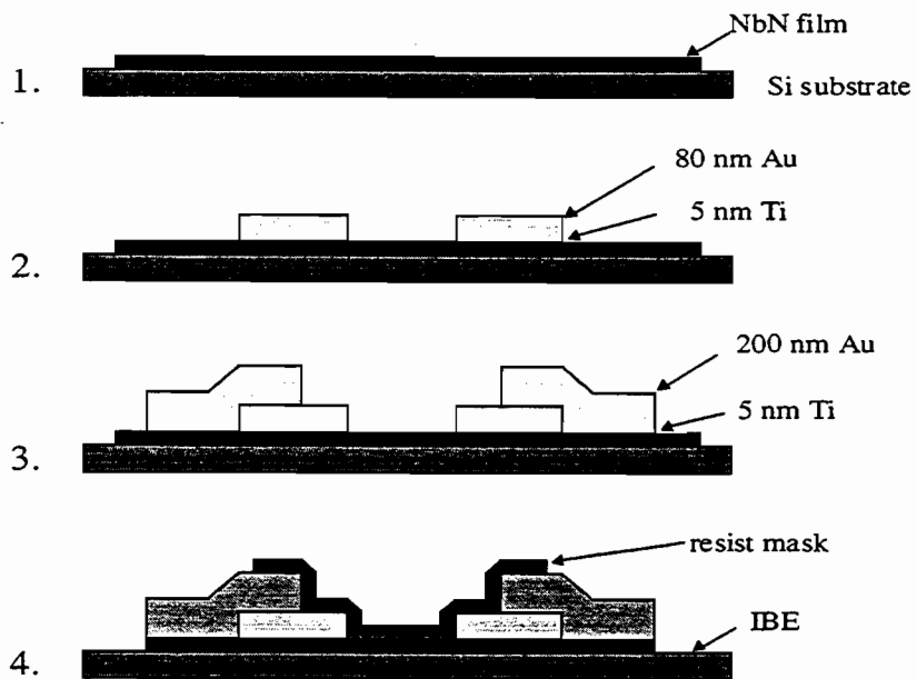
Fig.3. Schematic top of the fabrication process.
