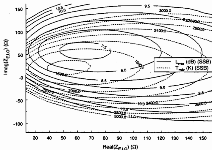
Figure 5: Contour plot of T_{\text{mix}} and L_{\text{conv}} based on simulations for diode SD1T7 with LO power of 1.2 mW
