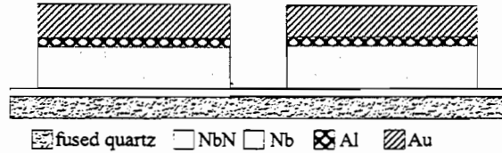
Figure 2: Sectional view of the microbolometer
