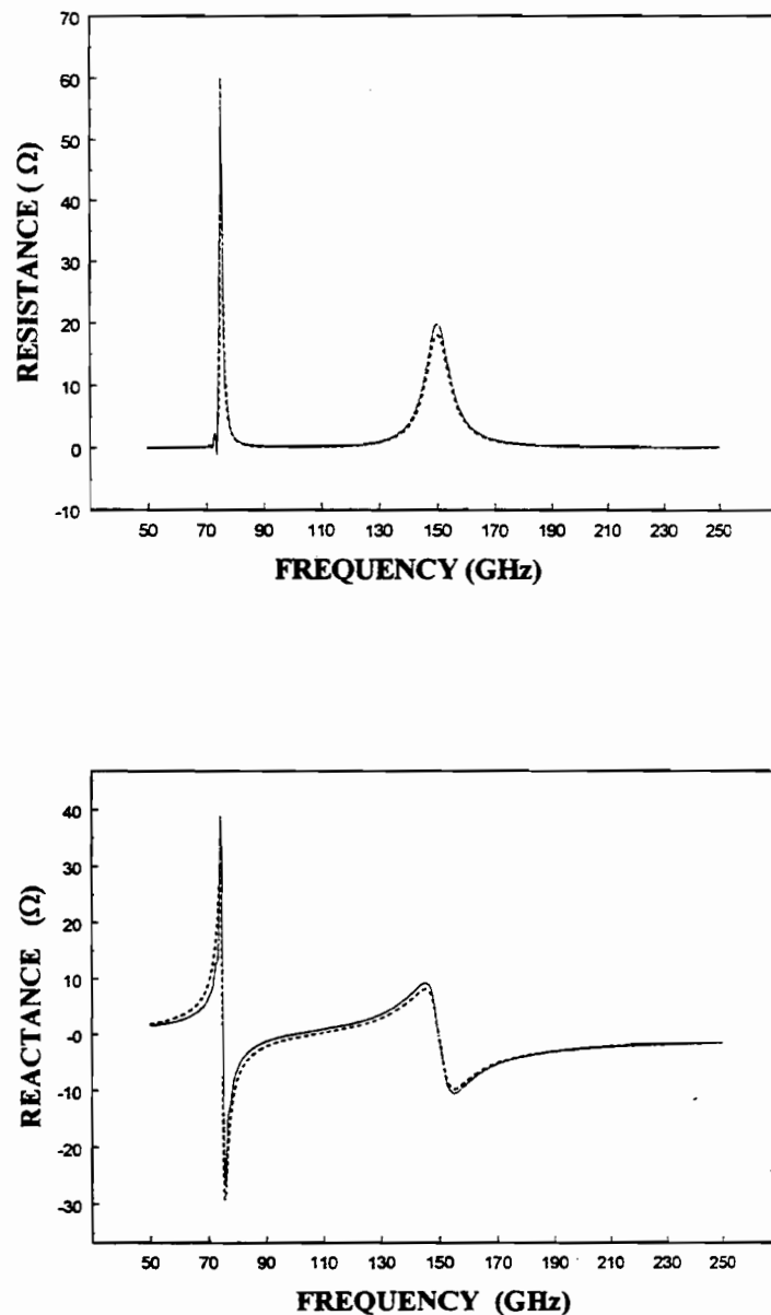
Figure 1. Reconstructed (solid line) and Original (dashed line) TE0 Circuit Impedances
