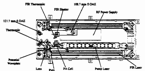
Figure 3: LLO optical path.
