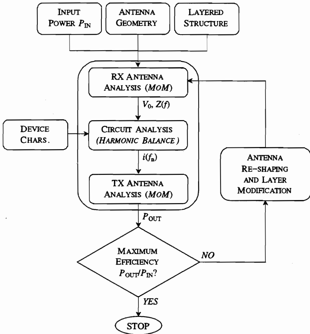
Fig. 8 – Block diagram of the computer code for the analysis and the optimization of the multiplier.
