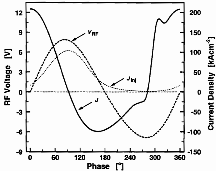
Figure 6: Waveforms of RF voltage V_{RF} , injected and total current densities J_{inj} and J of a GaAs TUNNETT diode as a function of time during one RF cycle at the fundamental frequency of 104 GHz.
