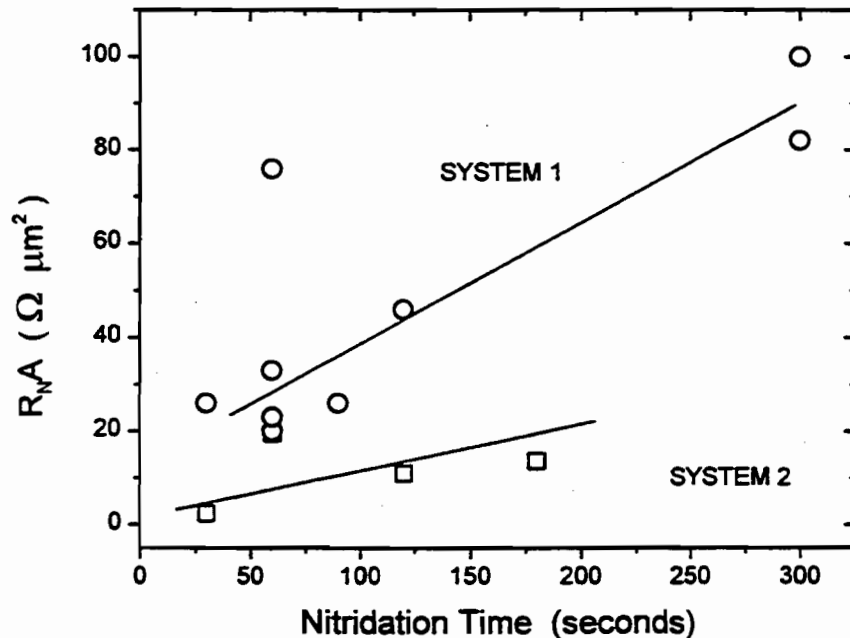
Figure 5. Junction R_{NA} vs plasma exposure time for (o) system #1 and (□) system #2, 20mTorr N_2 and approximately -30V.
