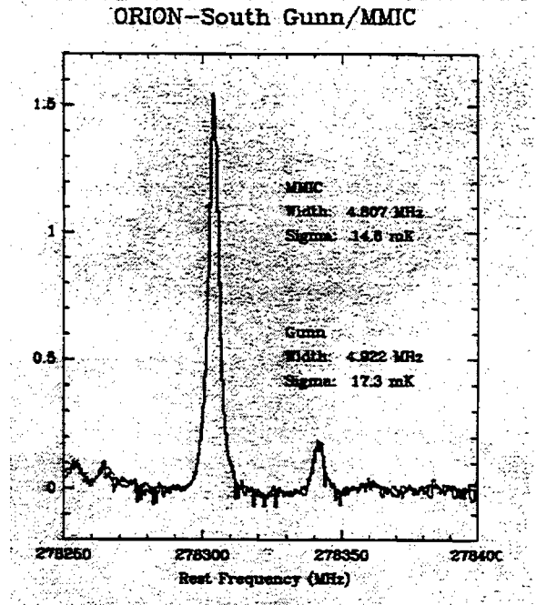
Figure 7: Observation of the Methanol line in the Orion Nebula with the two different LO chains as shown in Figure 6. Addition of the PA does not deteriorate the observation.
