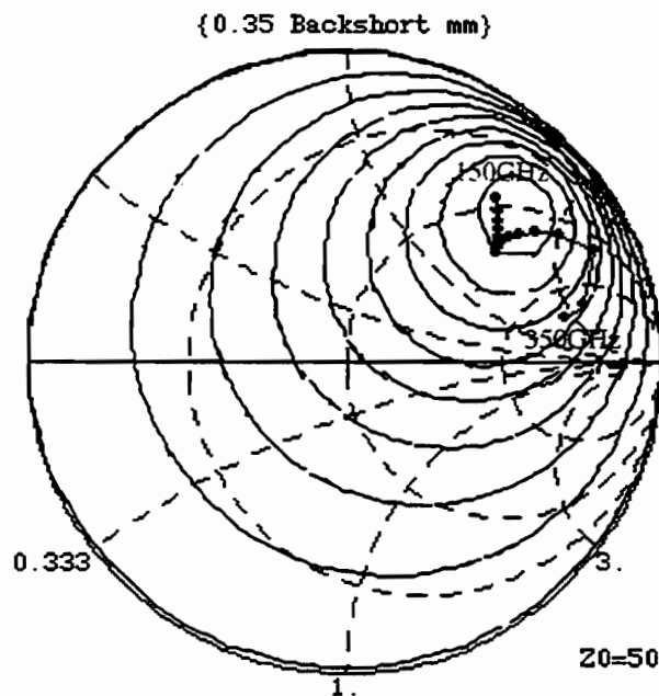
Figure 10: View of the contour plot for the 6 \mu\text{m} diode together with the E & K simulated response, for a = 1.35 mm, b = 0.1 mm, g = 0.035 mm and w = 0.1 mm.
