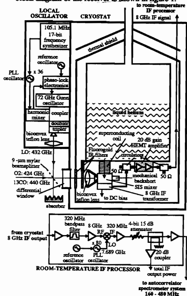
Fig. 1: General block diagram of the PIROG 8 receiver
