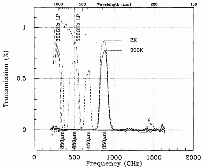
Fig. 6.— Transmission of resonant metal mesh bandpass and lowpass filters. All measurements but one are at 300K; the 350μm filter was also tested at 2K.
