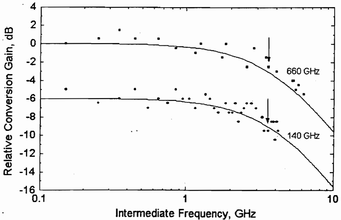
Fig. 3 Relative conversion gain for NbN device measured at 140 and 660 GHz under optimal LO and dc bias.
