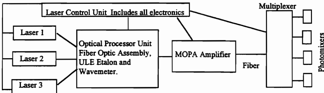
Figure 3. Laser photomixer LO source block diagram
