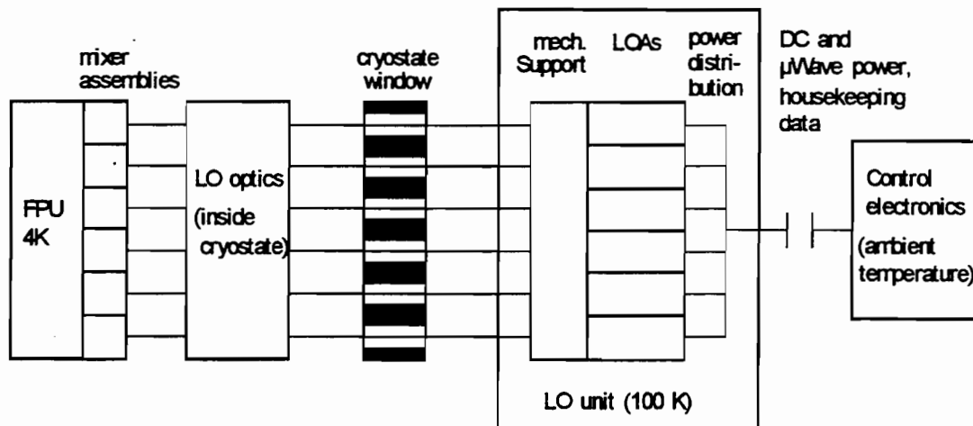
Figure 1: Schematics of the LO system with respect to the focal plane unit (FPU)
