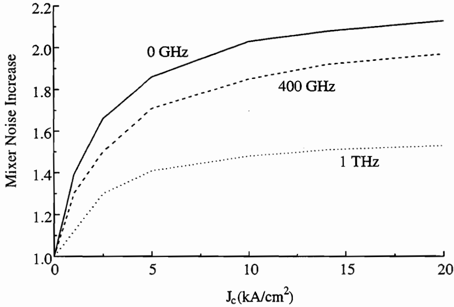
Figure 3: Correction factors to the Tucker[1] mixer noise due to the presence of MAR as a function of critical current density. At low frequencies the mixer noise is close to the shot noise at the bias voltage (the solid line). At higher frequencies the correction factor decreases because the contribution from voltages V_{bias} + \hbar\omega/e becomes important where single electron transport is dominant.
