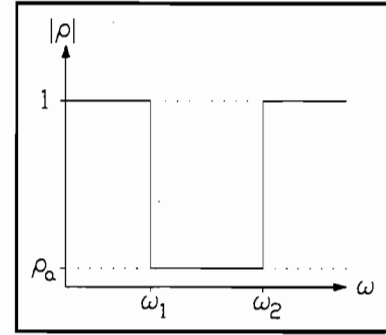
Fig. 2. Impedance matching profile for optimum bandwidth.
