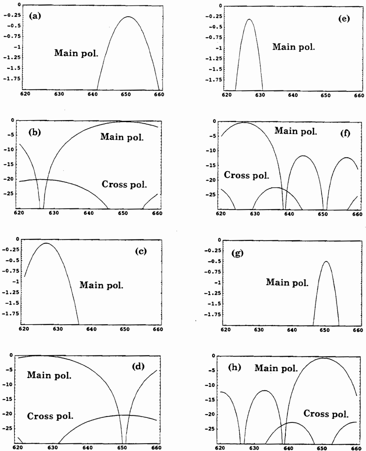
Fig.6 (a),(b) Insertion losses (dB) between MIX-1 and the Antenna Port in its main and cross polarizations. (c),(d) Same for MIX-2. (e),(f) Insertion losses (dB) between MIX-1 and the Cold Load Port in its main and cross polarizations. (g),(h) Same for MIX-2.
