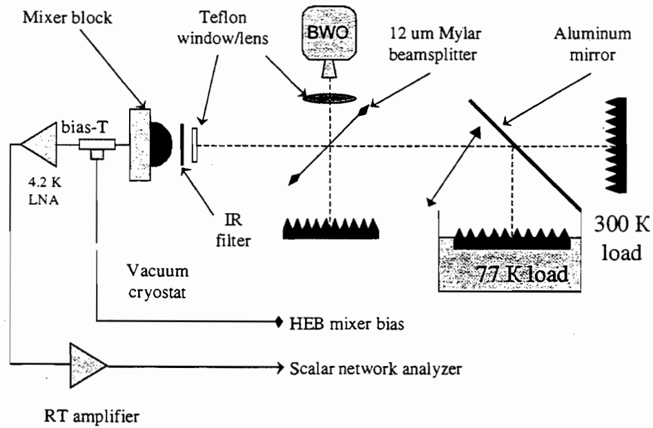
Fig.5. Setup for noise temperature measurements.
