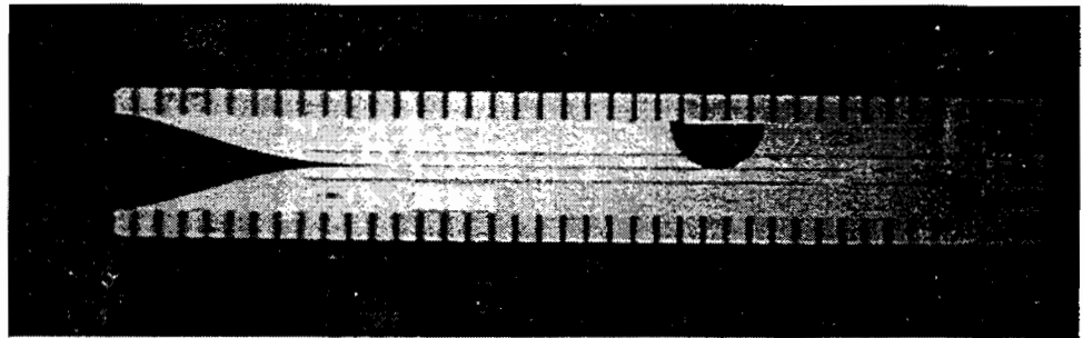
FIGURE II A magnified view and a photograph of the finline mixer chip
