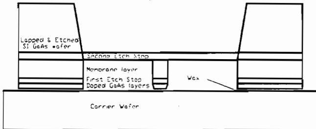
Wafer Mounted Upside Down on Carrier
