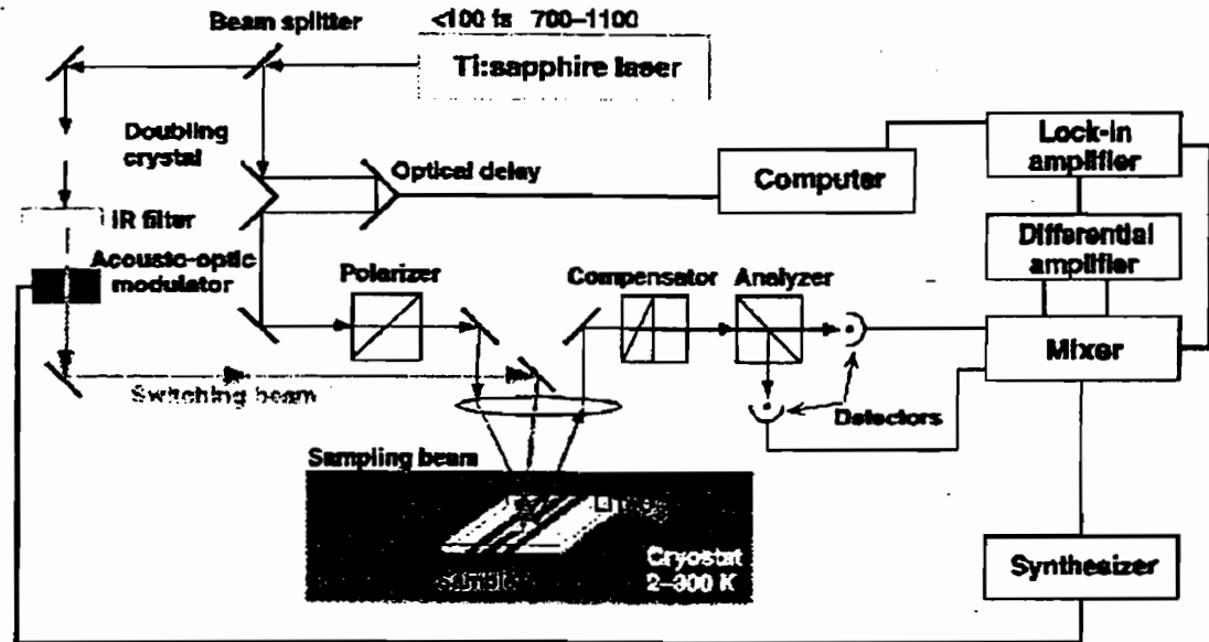
Fig.5 The cryogenic electro-optic sampling system measures ultrafast electrical transients.
