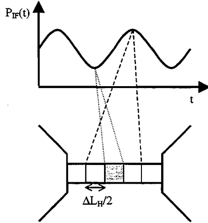
Figure 6: Schematic representation of the mixing process due to the modulation of the size of a hotspot. The grey areas schematically represent the hotspot in case of minimum and maximum power dissipation at the IF frequency. The white parts of the microbridge are superconducting.
