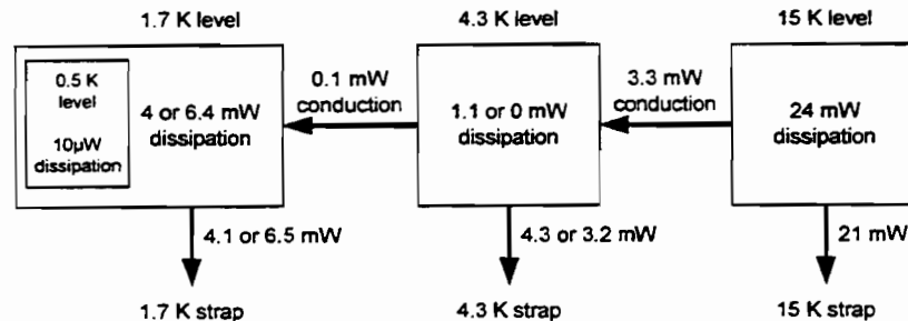
Figure 7. Diagram showing the HFPU thermal interface with the spacecraft.
