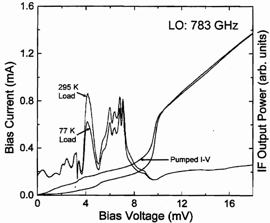
Fig.4 Heterodyne response of the receiver at 783 GHz. Shown are the I-V characteristics of the mixer device with and without LO power. Also shown is the IF power as a function of bias voltage for hot (295 K) and cold (77 K) loads.
