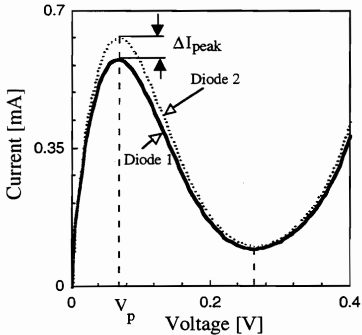
Fig. 2 If the diode I-V curves are not identical, a lower current diode (diode 1) cannot achieve the peak current I_p of the higher current diode (diode 2) at the voltage V_p .
