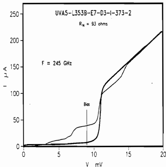
Fig. 5. I-V curve for the mixer at 4.2 K without LO power (heavy line), and with LO power at 245 GHz (light line). The operating bias voltage is indicated by the vertical line.
