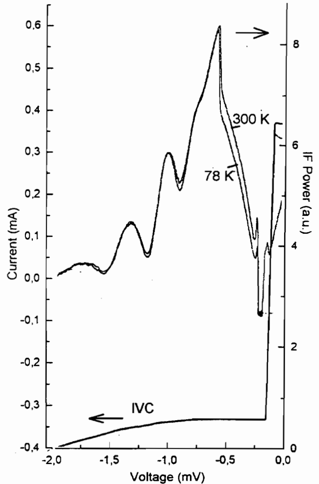
Fig. 5: Hot/Cold-measurement in the to the IF amplifier.
