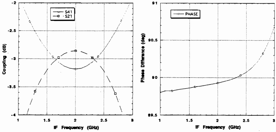
Fig.3 Calculated coupling and phase-difference of the Lange coupler which is designed for a center frequency of 2.0 GHz.
