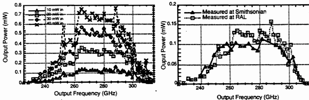
Final measured frequency response as a function of input power (Backshort fixed at 0.45mm)
