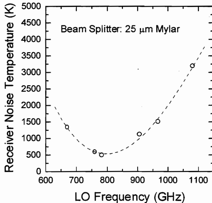
Fig. 5 DSB receiver noise temperature as a function of LO frequency.
