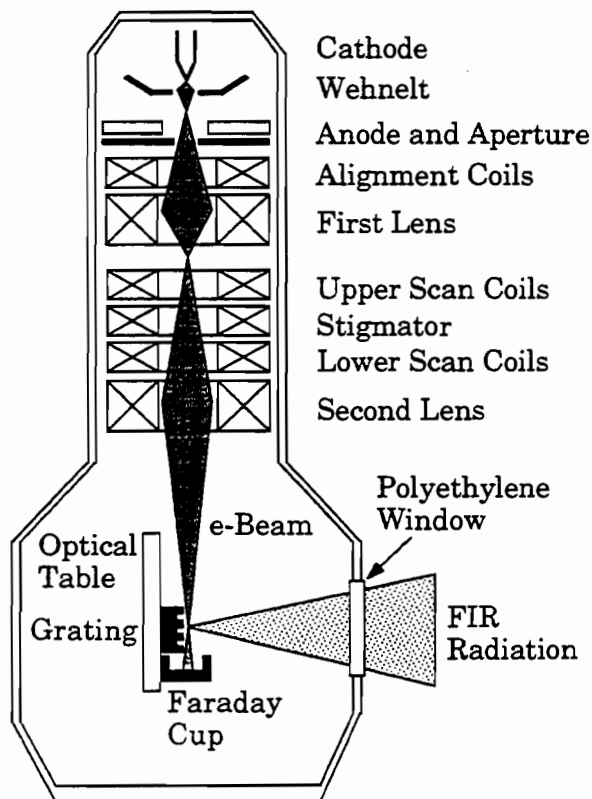
FIG. 1. Diagram of the SEM optical system.
