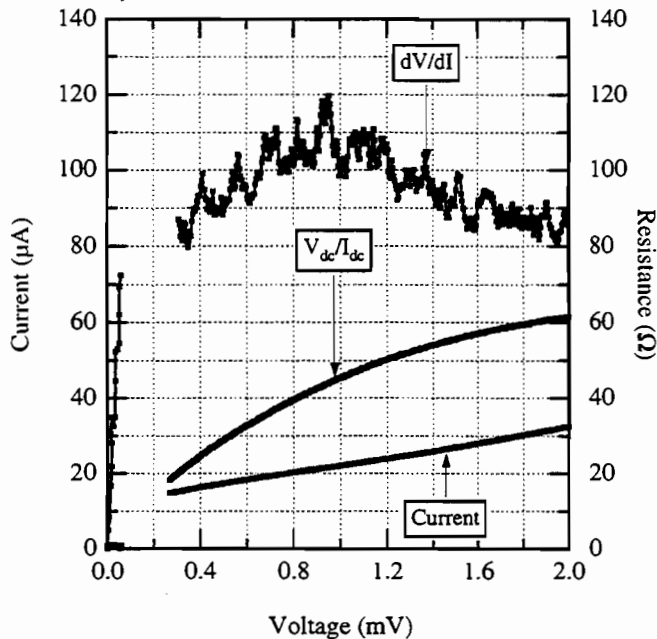
FIG. 8. IV curve, dynamic and absolute resistance for device B, optimum efficiency case.
