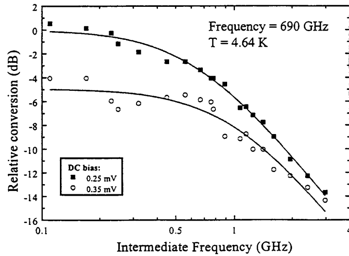
FIG. 5 Relative conversion efficiency of a HEB mixer is measured as a function of intermediate frequency at two bias voltages. The data points are the measurements and the curves are the fits (see the text).
