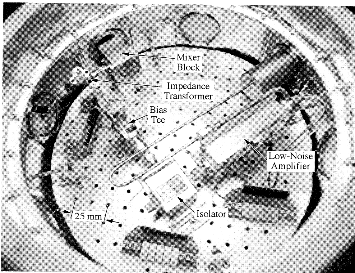
Fig. 6. Picture of the Infrared Laboratories HD-3(8) dewar used during the mixer testing at 77 K and 4.2 K.
