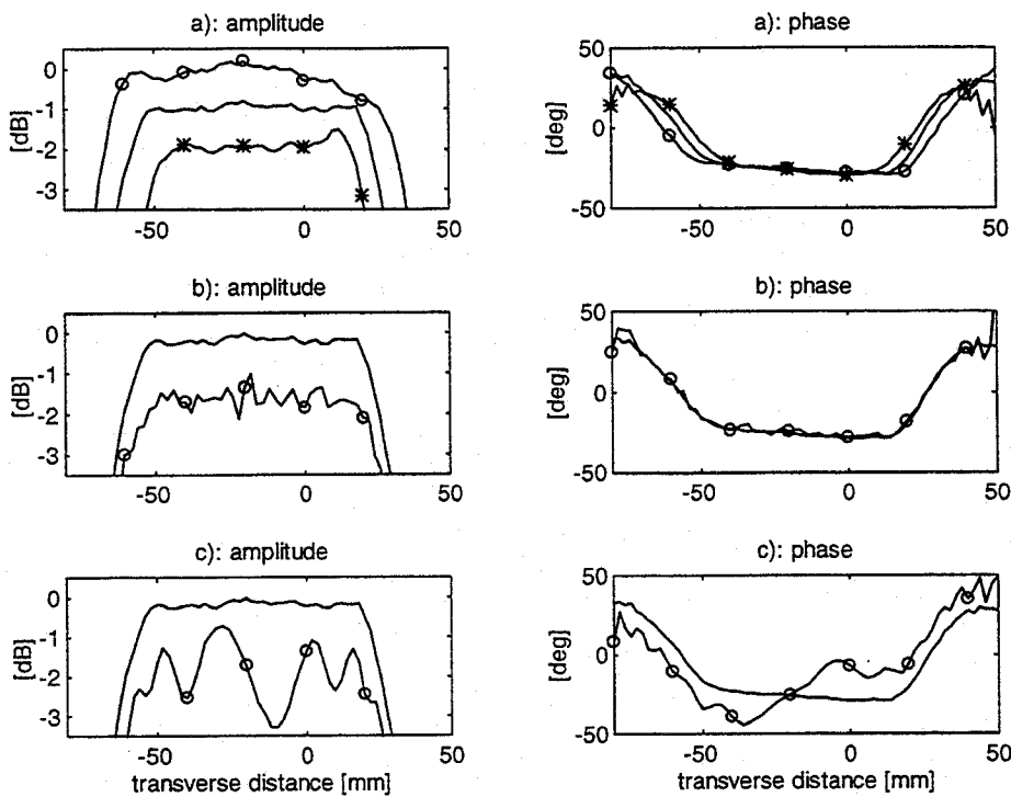
Figure 6. a) Effect of the \pm 30 \mu\text{m} systematic fabrication errors: ideal case (-), +30 \mu\text{m} (o) and -30 \mu\text{m} (*), b) effect of the random error, \sigma = 10 \mu\text{m} (o), c) effect of a 100 \mu\text{m} vertical gap in the center of the hologram (o).
