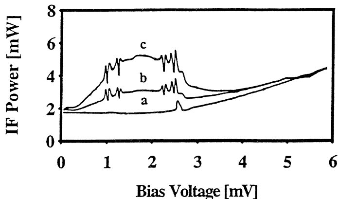
Figure 3. Receiver output power at the intermediate frequency 1.5 GHz a) without the local oscillator power P_{LO} , b) with the P_{LO} and with the nitrogen temperature load in front of the receiver, C) with P_{LO} and with the ambient temperature loads.
