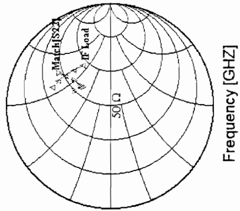
Fig. 7 A 4-8 GHz IF matching network which transforms a 50 Ohm input impedance to the required IF load impedance given the condition, S_{11}(RF) = -3\text{dB} . Since it is physically impossible to provide a negative capacitance, a good impedance match can only be provided over a limited (octave) of bandwidth.
