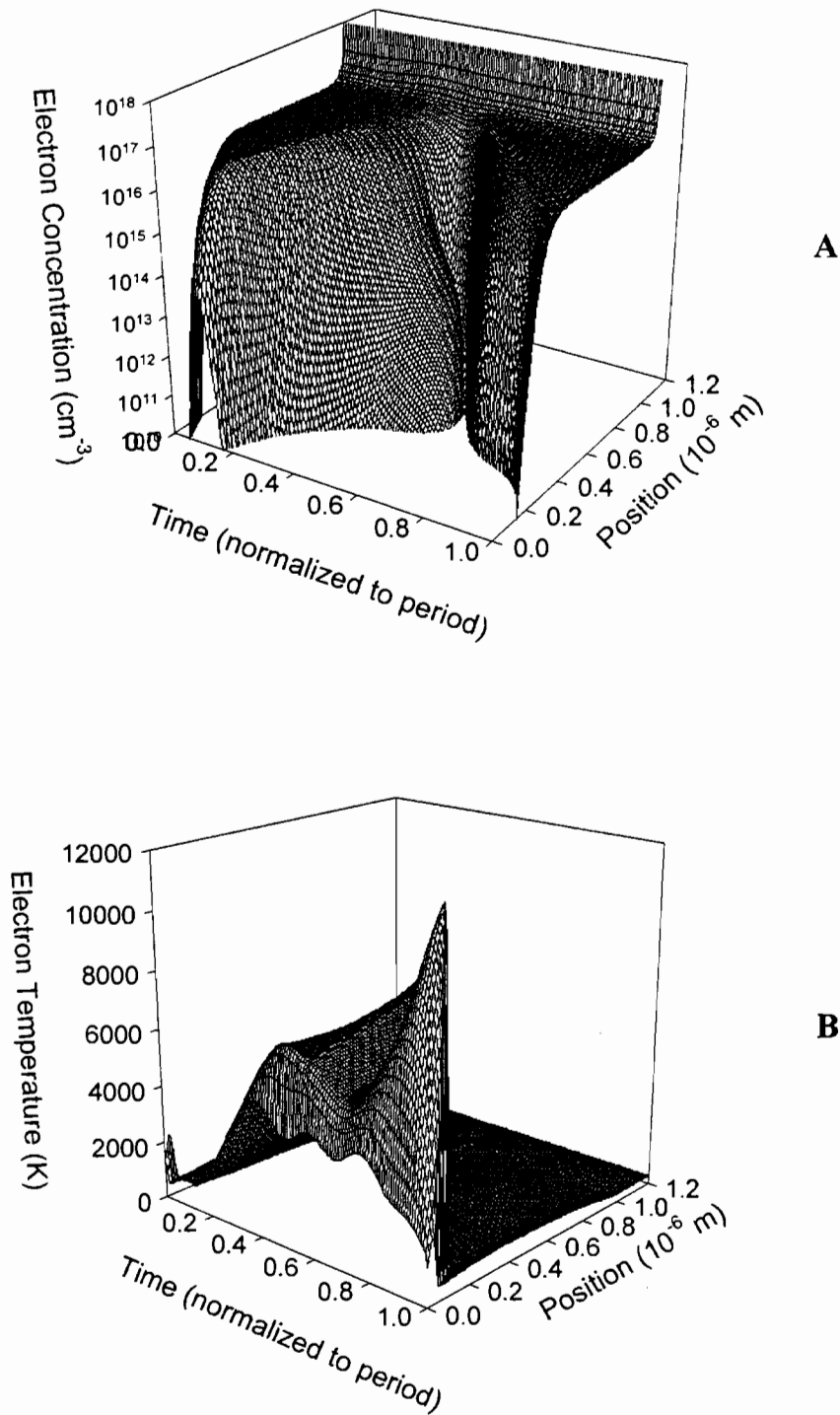
Figure 3. (A) electron density , and (B) electron temperature, versus position and time.
