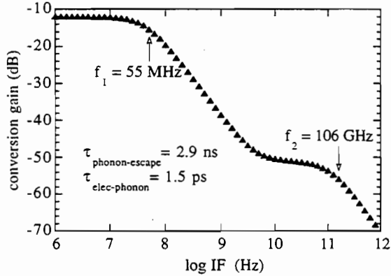
Figure 1: Calculation of the conversion gain bandwidth for a YBCO HEB mixer using the model of Ref. 6. An ideal 100% coupling of power to the HEB is assumed. The parameters used, including the phonon escape lifetime and the electron-phonon scattering time, are appropriate to YBCO with the nominal physical dimensions of the devices discussed in the text.
