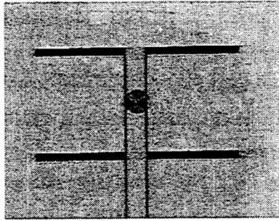
Figure 2: SEM micrograph of a YBCO HEB coupled to a 585 GHz double-slot antenna and a co-planar transmission line. The 2\ \mu\text{m} \times 2\ \mu\text{m} HEB itself is at the intersection of the two tapers in the center of the picture. The width of the antenna arms is 175\ \mu\text{m} .
