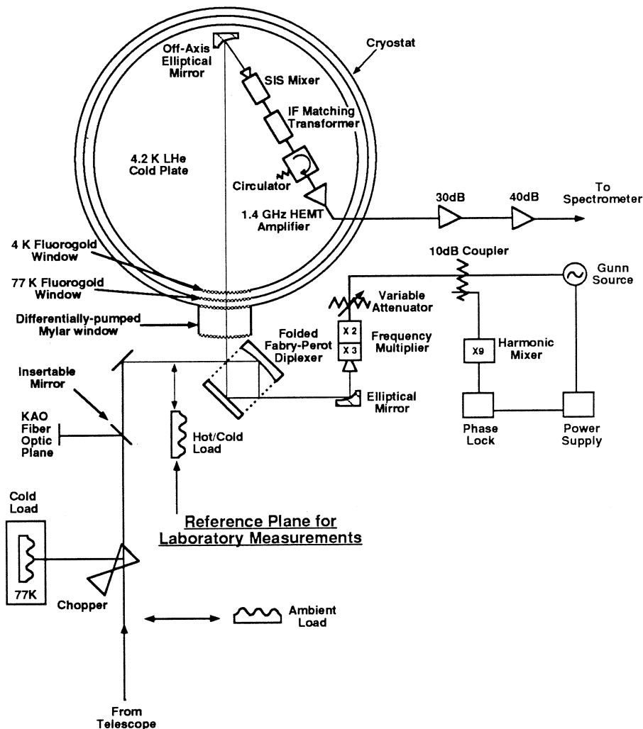
Figure 3: Block diagram of SIS heterodyne receiver. Noise measurements are referred to the reference plane at the signal input port of the Fabry-Perot diplexer.
