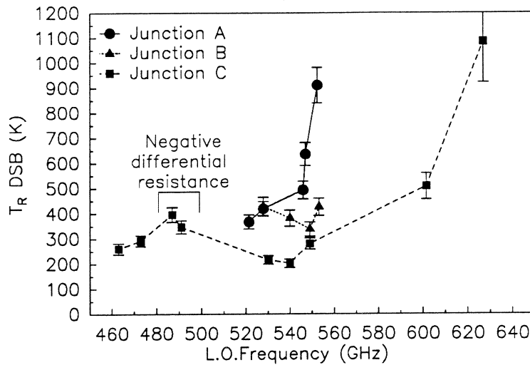
Figure 4: Receiver noise temperature as a function of the LO frequency for 3 different SIS junctions. Junction A uses a series transformer tuning circuit and junctions B and C use a parallel circuit with a radial stub (see text). Very good performance is obtained from 463 GHz to 627 GHz, with the best result T_R = 200 K at 540 GHz for junction C. Negative resistance is also observed near 490 GHz.
