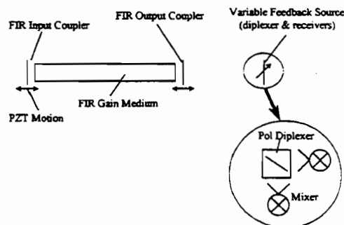
Figure 14: FIR feedback mitigation approach.
