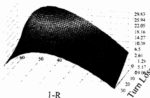
Figure 11: Rigrod prediction for FIR output vs turn loss and output coupling. Pump power fixed @ 5 W.
