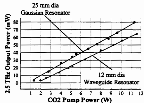
Figure 10: 1.5 m straight-guide Demonstration Program FIR results.
