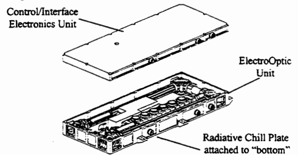
Figure 2: LLO system, enclosure opened.
