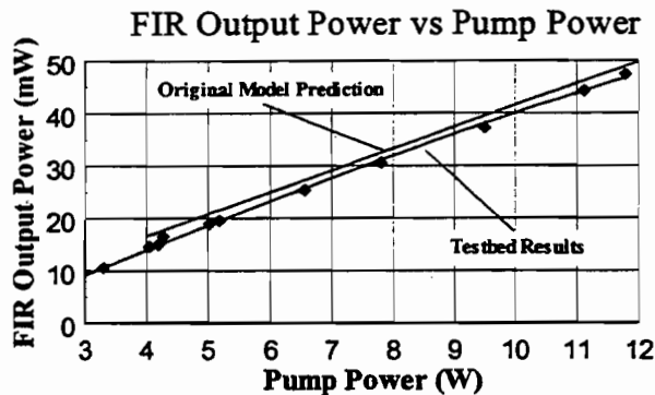
Figure 18: Testbed results: comparison with original model.
