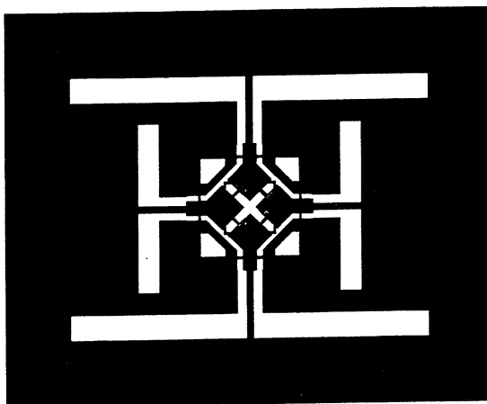
Circuit layout
