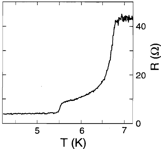
Fig. 2; Resistance versus temperature curve for the HEB mixer.
