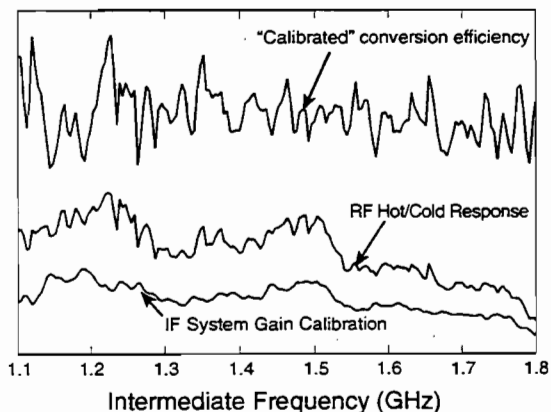
Fig.8: The RF hot/cold response, the IF system gain and the conversion efficiency calculated as the ratio of the two curves. No roll-off in the response is seen. This measurement was made at an ambient temperature of 4.2 K.
