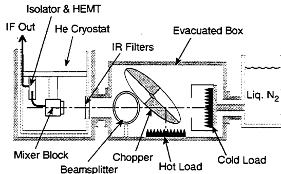
Fig. 3; Schematic of the cryostat containing the mixer and of the measurement box with the hot and cold calibration loads. There are no windows between the cryostat and box, but there are two Zitex™ infrared filters in the optical path.
