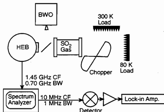
Fig. 6; Block diagram of the laboratory set-up for the gas cell measurement. A spectrum analyzer was used as a tunable IF filter.
