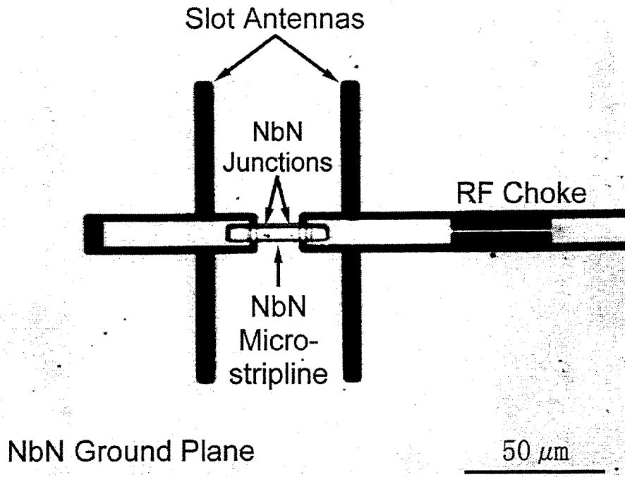
Fig. 3. Optical micrograph of the 1 THz NbN/AlN/NbN mixer. Two NbN junctions in parallel with integrated tuning circuits are fabricated with a twin-slot antenna. Each junction is approximately 0.5 \mu\text{m} in diameter.
