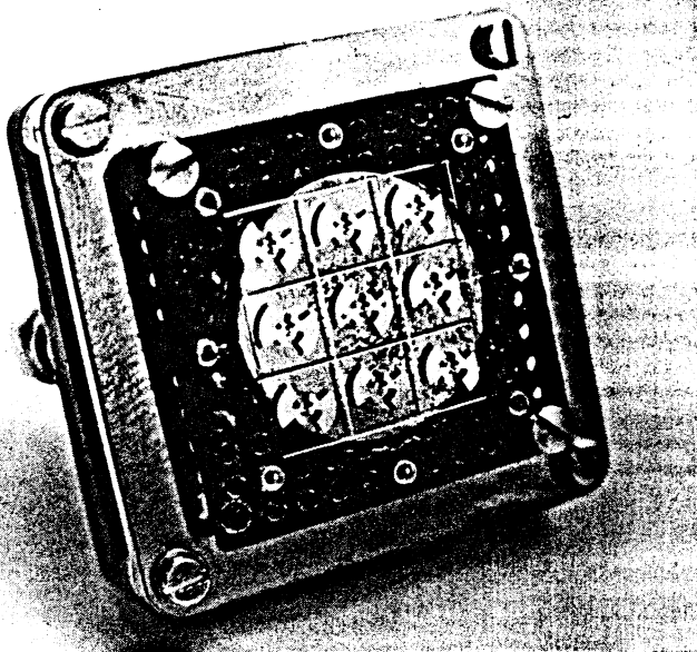
Fig. 7: Photograph of 3x3 element logperiodic planar array in a mounting with a reflecting backshort. The wires ( 25\mu\text{m Au} ) to the centre element are visible
