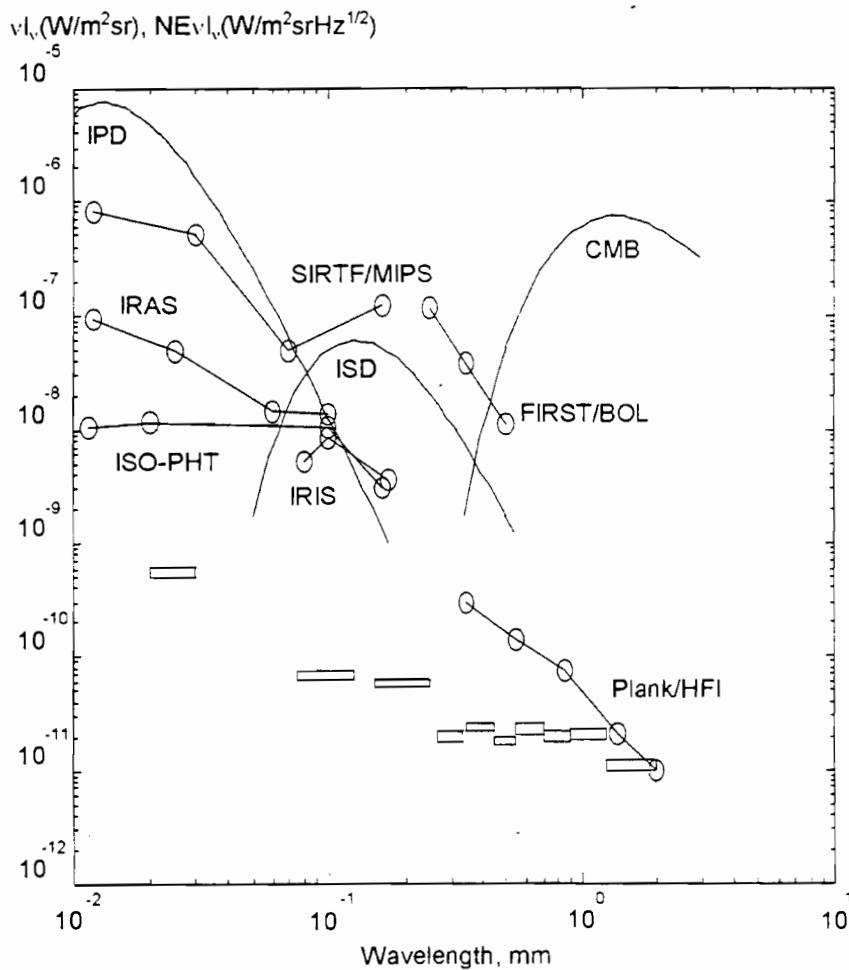
Figure 3. The sensitivity related to brightness of extended sources. Rectangles - the Submillimetre Project, circles - other projects. NE \nu I_\nu - noise equivalent brightness with S/N=1 . The brightness of sources given for comparison: CMB - cosmic microwave background, ISD - interstellar dust emission, IPD - interplanetary dust emission.
