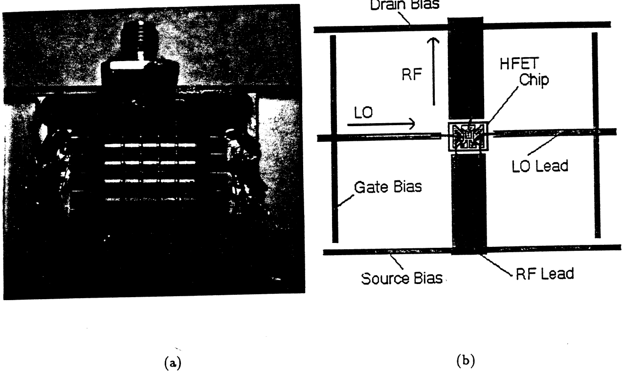
Figure 3. (a) Photograph of the 16-element HFET grid mixer. The LO signal is vertically polarized and the RF horizontally polarized. (b) Schematic of the grid unit cell showing how the chip is connected with bonding wire. Note that the unit cells in Figure 3(a) are rotated by 90^\circ
