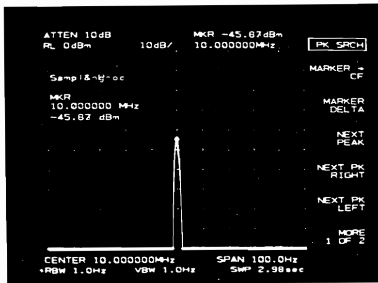
Figure 3b Output spectrum for the harmonic mixer IF down converted from the 135 GHz RF output.
