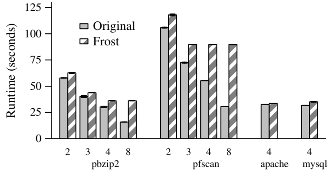
This figure shows how Frost affects execution time for four benchmarks on an 8-core machine. We show results for 2, 3, 4 and 8 threads for pbzip2 and pfscan. Apache and MySQL are I/O bound, so results are the same between 2 and 8 threads; we show the 4 thread results as a representative sample. Results are the mean of five trials; error bars are 90% confidence intervals. Frost adds a small amount of overhead (3-12%) when there are sufficient cores to run the extra replicas. When the number of worker threads exceeds 3 (pfscan) or 4 (pbzip2), Frost cannot hide the cost of running additional replicas.
