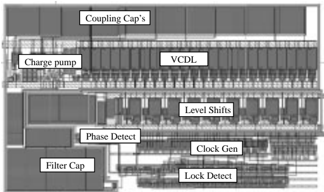
FIGURE 8. DLL synthesizer layout.
