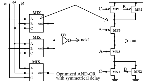
FIGURE 5. Clock frequency multiply X3 circuit.
