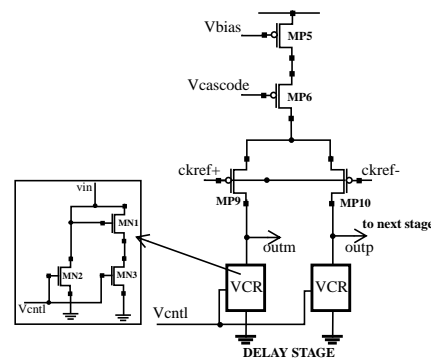
FIGURE 3. VCDL delay stage biasing schematic.
