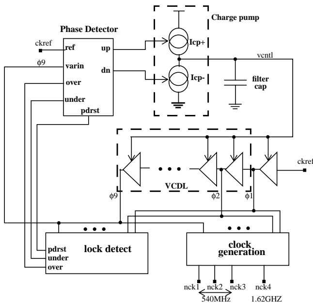
FIGURE 2. Clock synthesizer block diagram.
