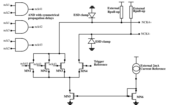
FIGURE 7. 1.62GHz clock generation schematic.
