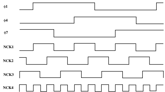
FIGURE 6. Clock generation waveforms.
