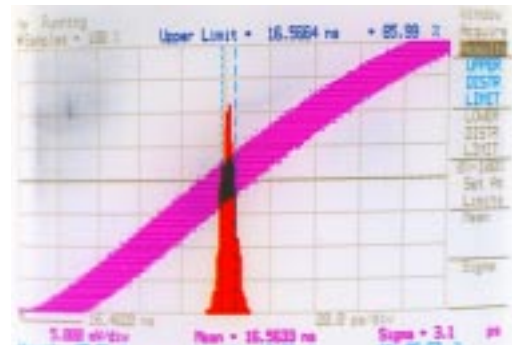
FIGURE 9. Measured 1.62GHz output clock edge jitter.
